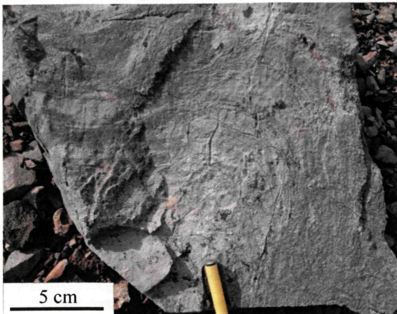
Plate 4: Stromatolitic Carbonate, Gillespie Lake Formation
