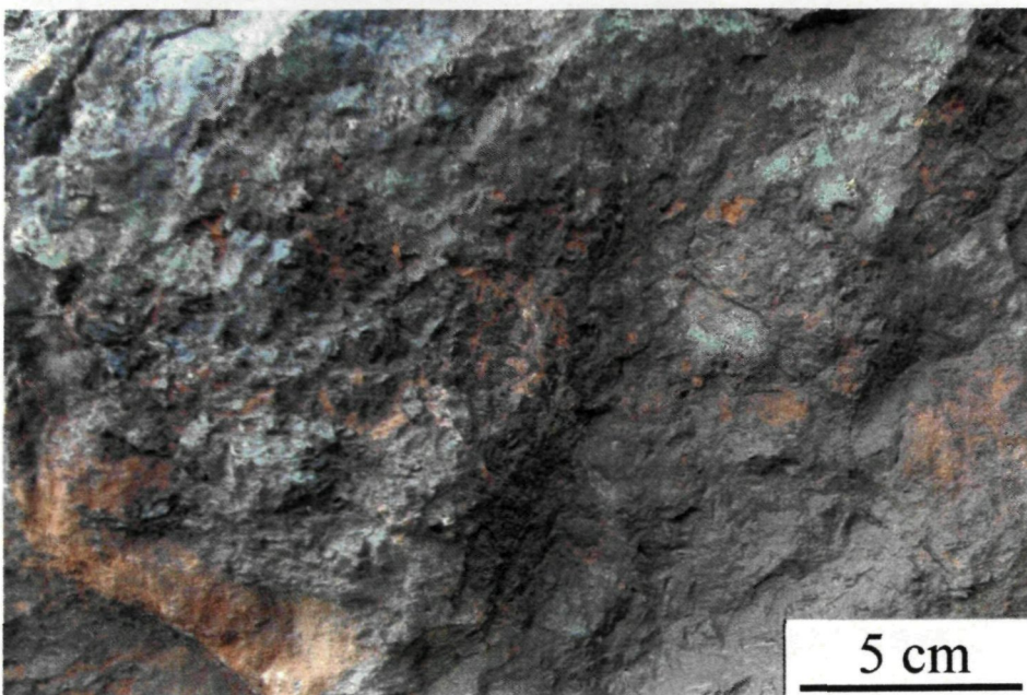
Plate 12: Malachite in siderite-Mn vein
