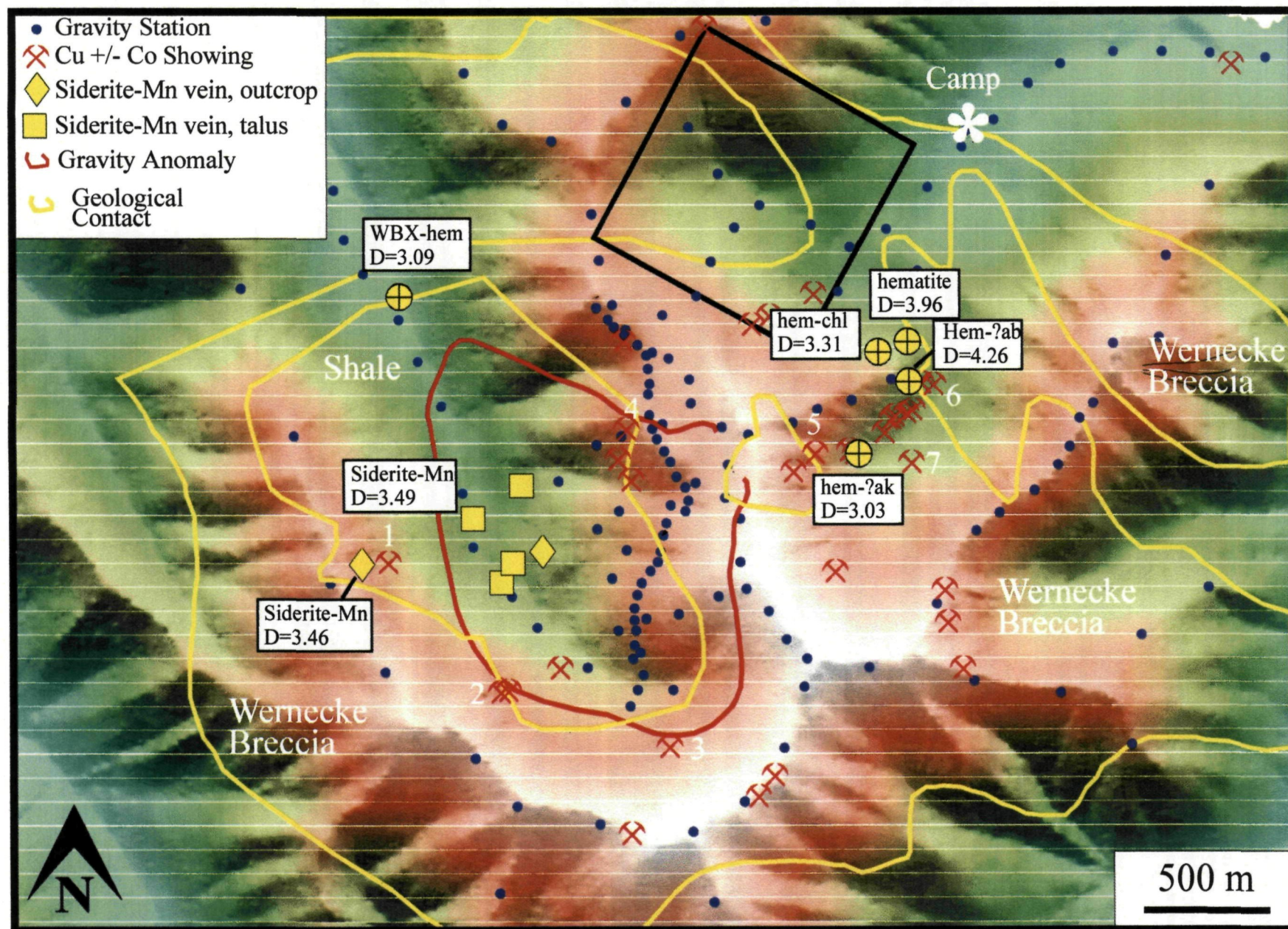
Figure 10: Main Gravity Anomaly, Showings and Dense Samples. 1: M-203 (2.2% Cu, grab, Siderite-Mn vein); 2: Champagne North (11.35% Cu, grab); 3: Champagne East (3.4% Cu, grab); 4: Panther (1.3% Cu, grab); 5: Cobalt Cirque (4.2% Cu, 295 ppb Au, grab); 6: Goblin (0.34% Cu, 0.04% Co, 1 m chip); 7: Mark's High Grade (3.5% Cu, 2.72% Co, 50 cm chip).
