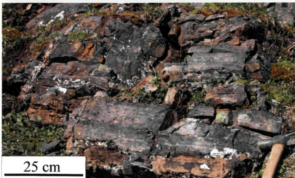
Plate 3: Partly carbonatized shale
