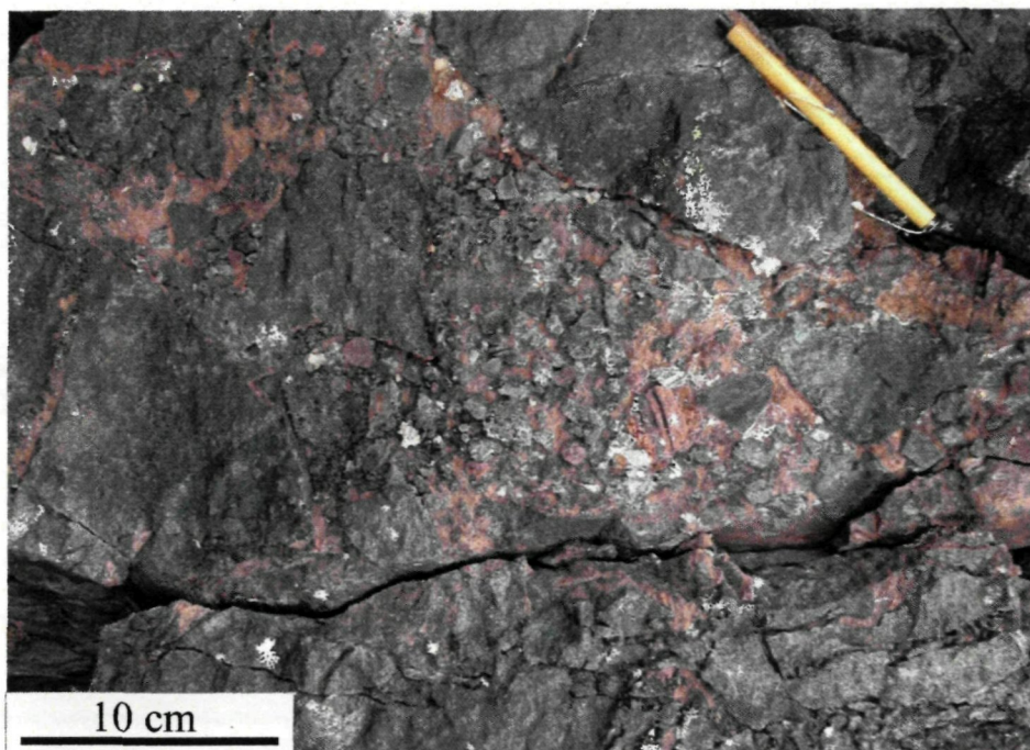
Plate 7: Dismembered diorite dike incorporated into the Wernecke Breccia
