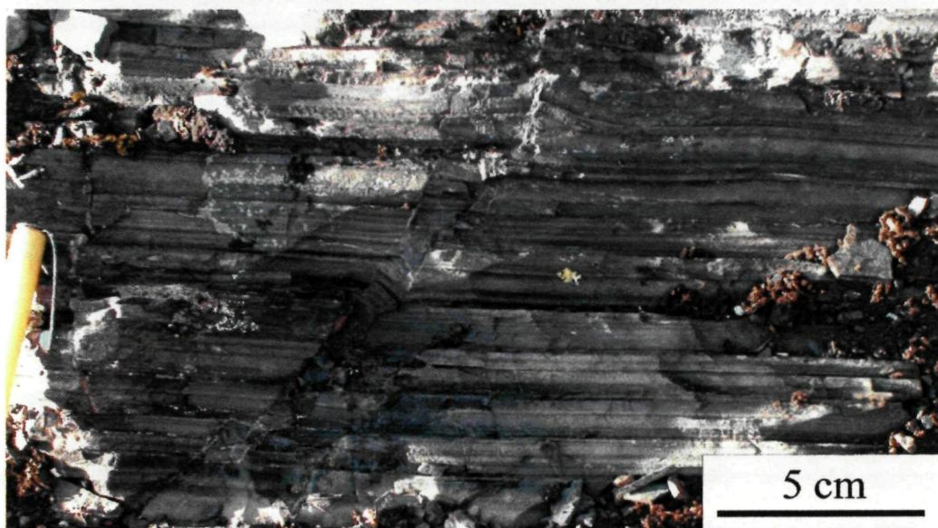
Plate 2: Bedded shale
