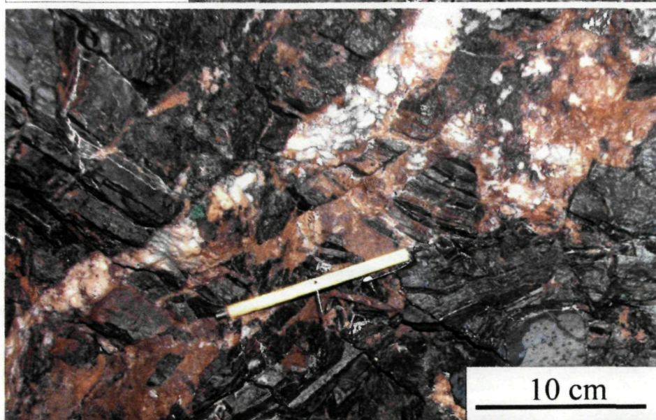
Plate 8: Malachite in carbonate-quartz vein which cuts shale
