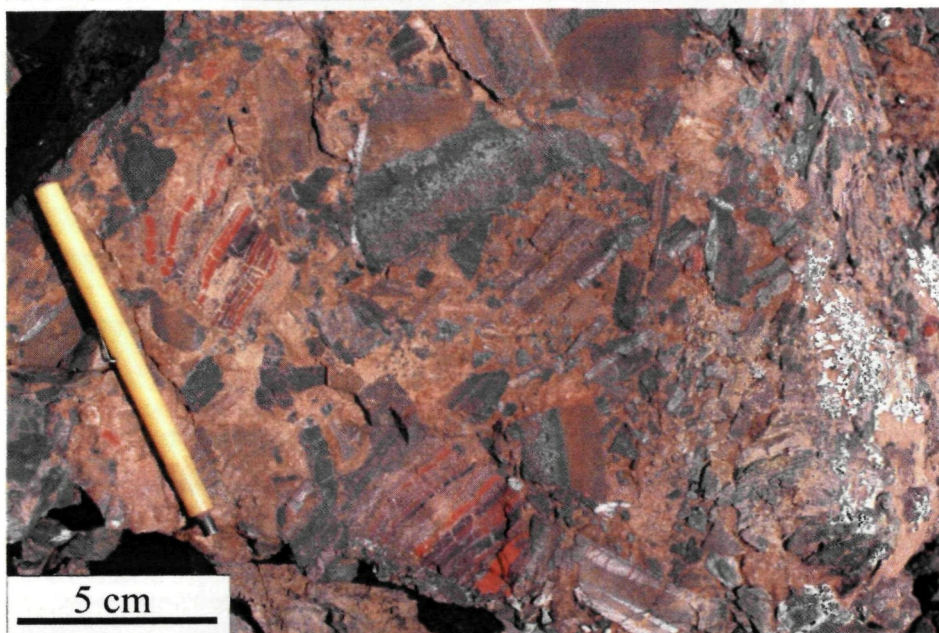
Plate 5: Wernecke Breccia with carbonate matrix
