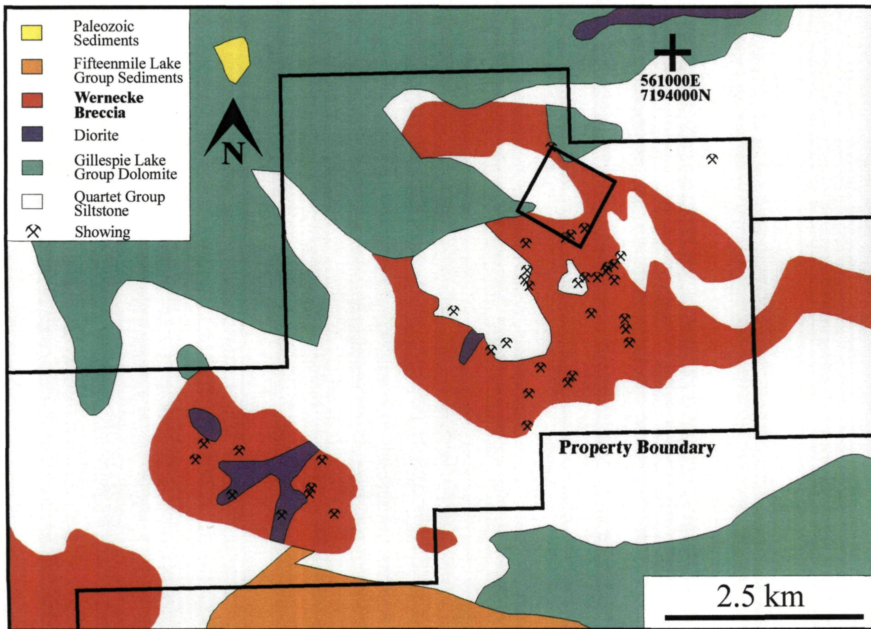
Figure 8: Showings in the core of the Monster Claims
