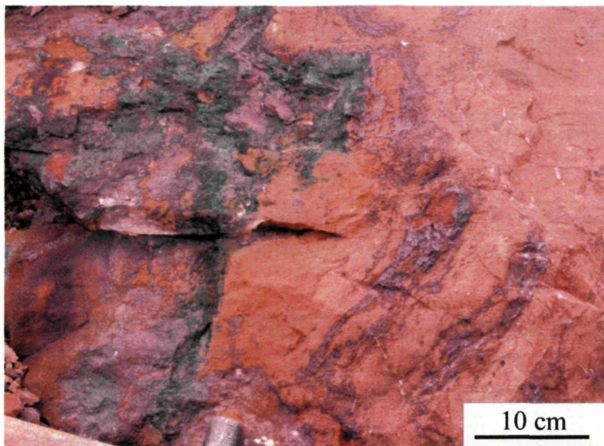
Plate 10: Malachite in carbonate-rich Wernecke Breccia
