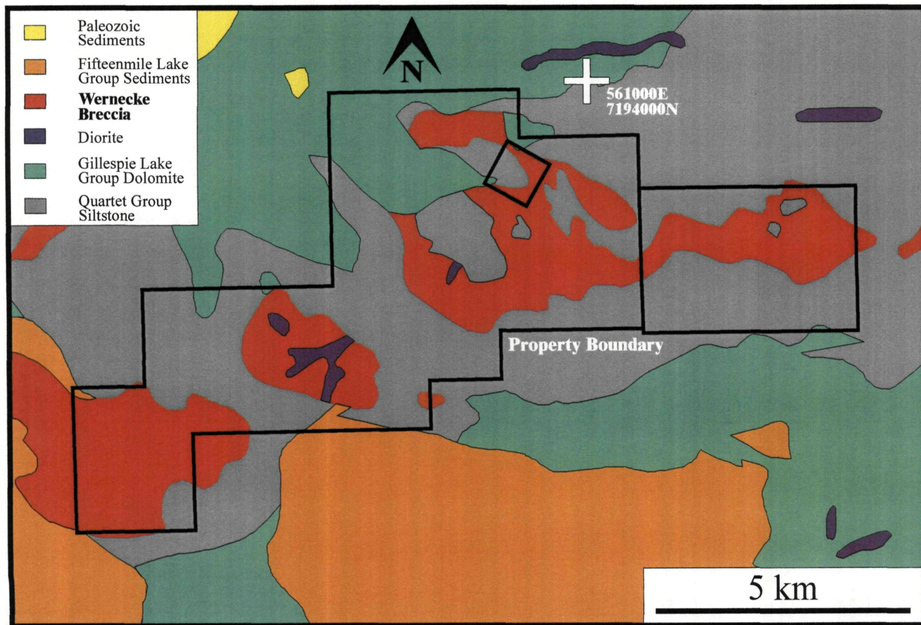
Figure 7: Geology of the Monster/Cookie Property. Modified after Thompson et al. (1992).
