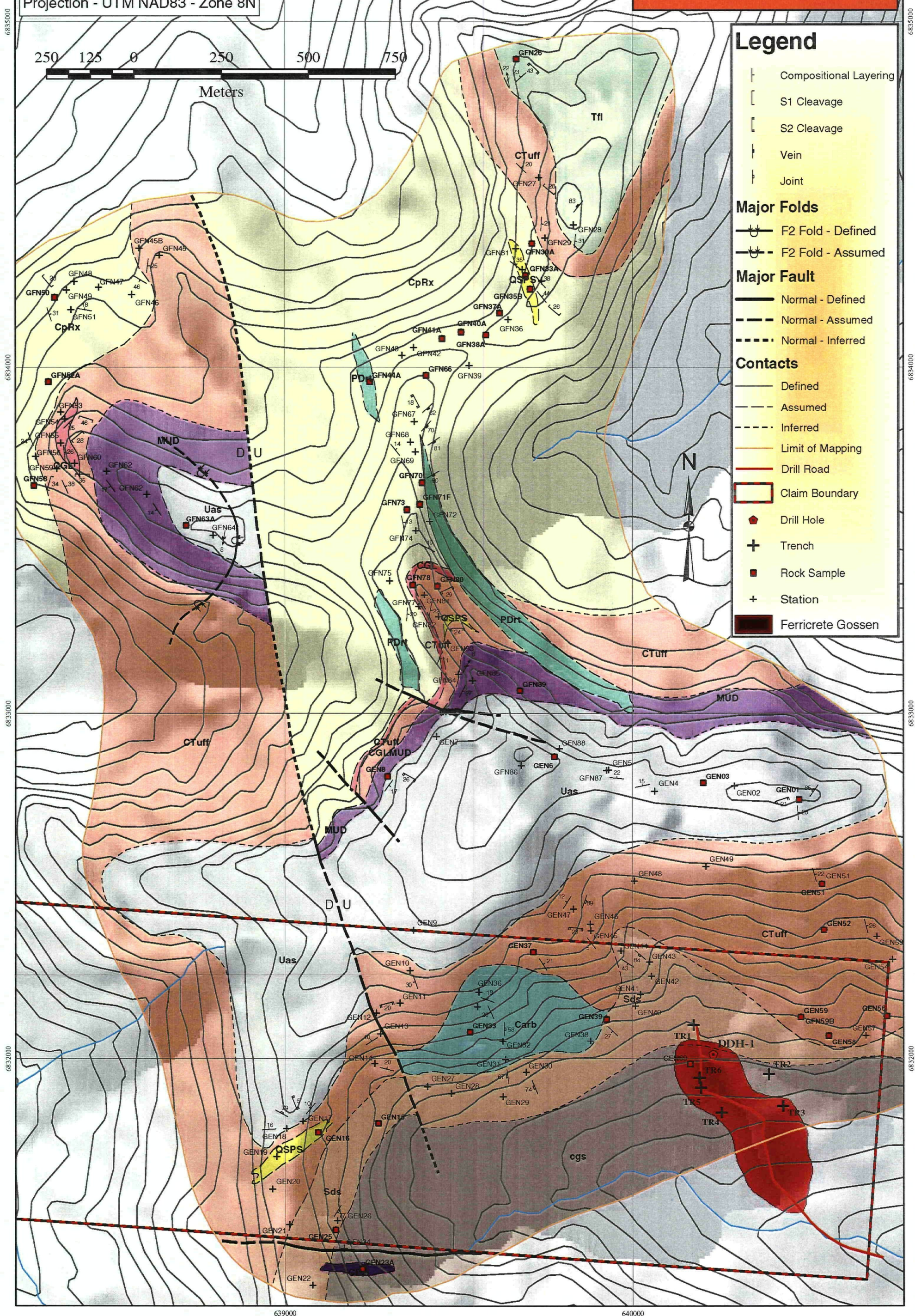
Figure 5 - Eros Property Geology (after Gallagher, 2002 and Greig, 2002)
