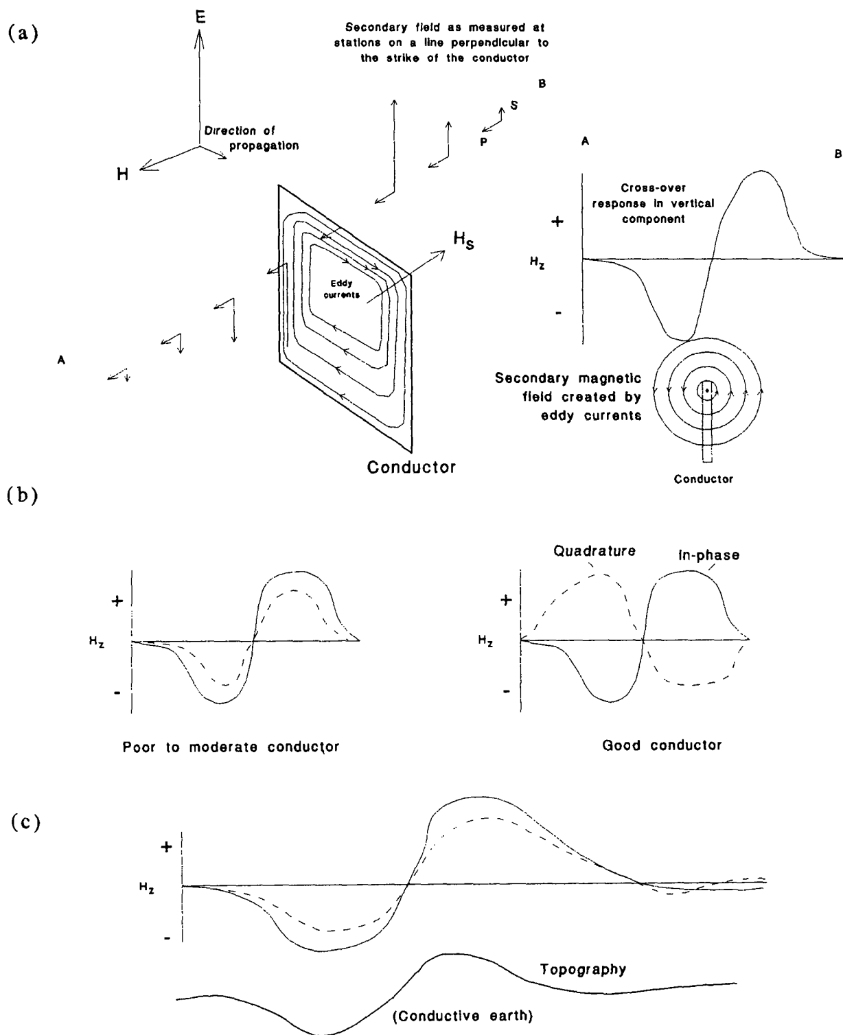
Figure VLF-2 VLF responses (a) The horizontal magnetic flux from a VLF signal induces a secondary field in a conductor. This, together with the primary field, produces a cross-over response (b) Quadrature sign can be determined by target conductance (c) If the ground is conductive, topography can induce VLF responses similar to those expected from bedrock conductors
