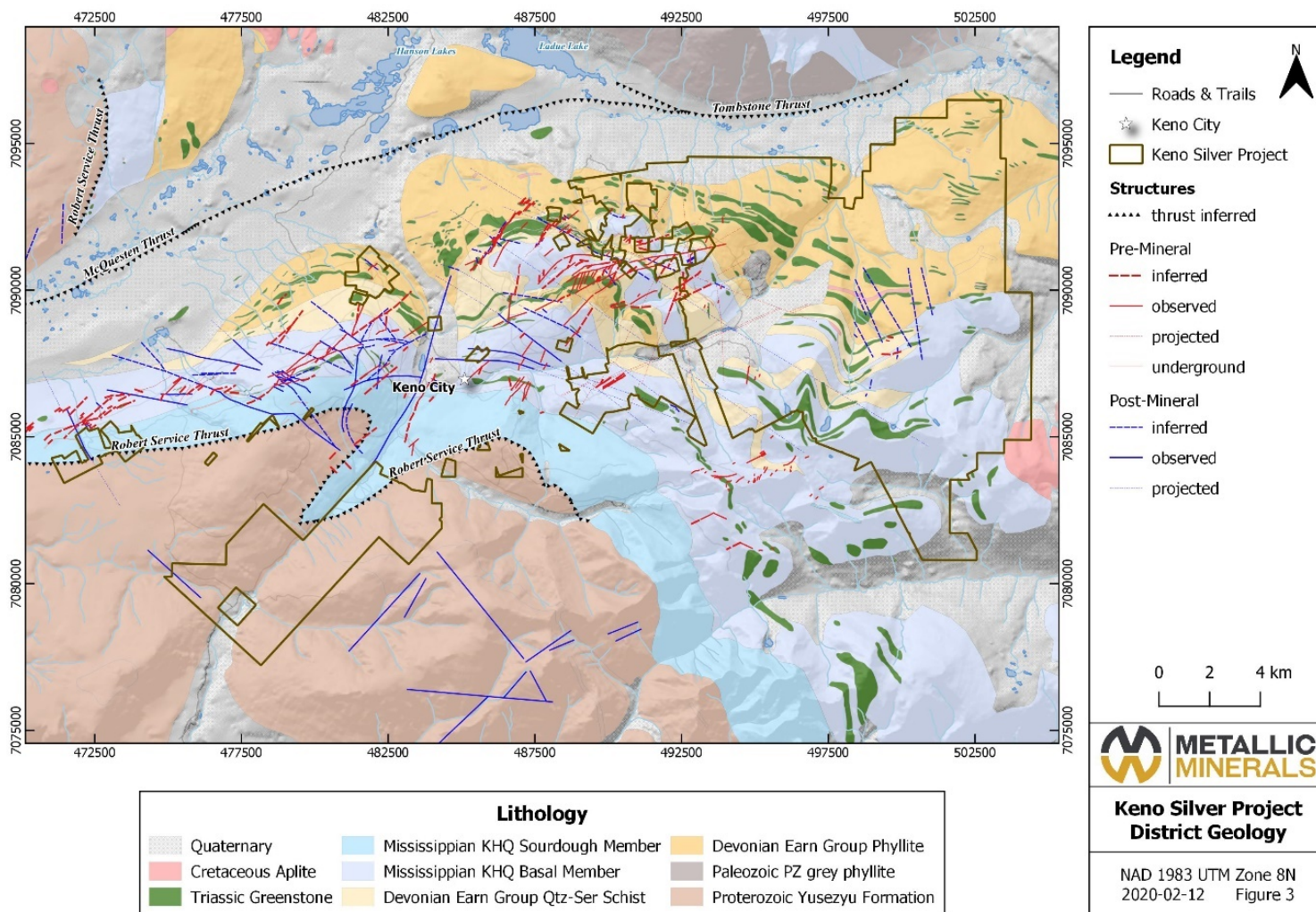
Figure 3. District Geology
