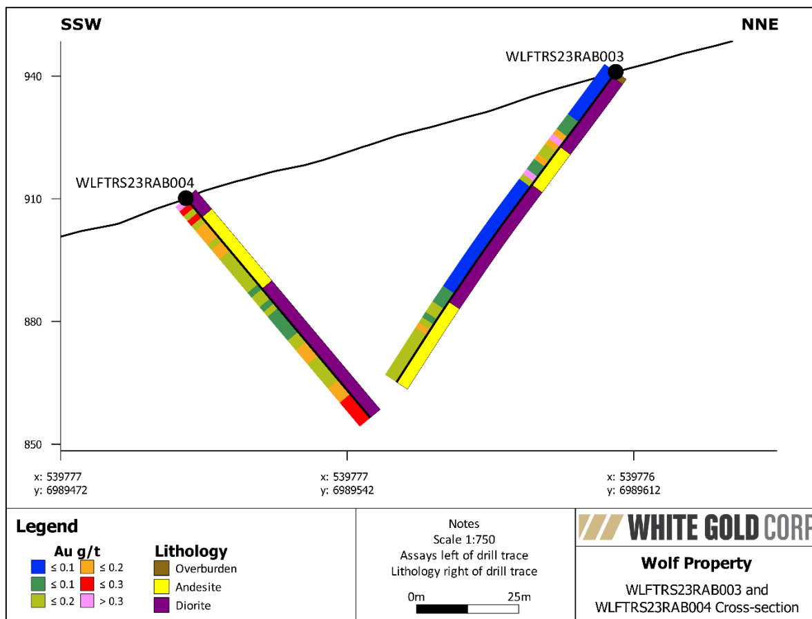
Figure 19. Cross-section of RAB holes 003 and 004 showing lithology paired with gold assays in g/t
