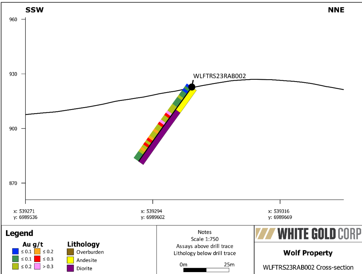
Figure 18. Cross-sections of RAB holes 001 and 002 showing lithology and gold assays in g/t
