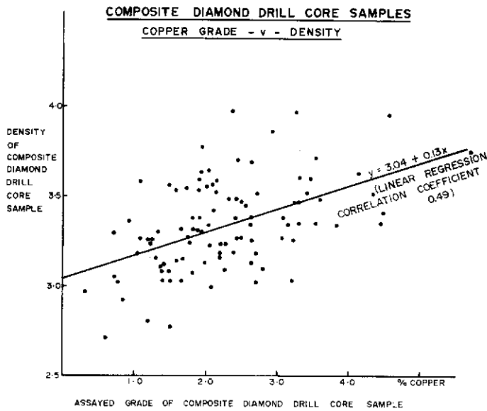
Figure 18. Plot of copper grade against density for composite underground diamond drill core samples. Note the regression line is almost the same as that in figure 32, suggesting that dilution has little influence on density of ore delivered to the mill.
