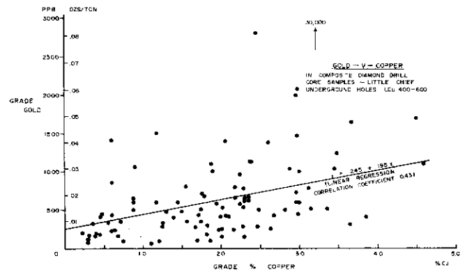
Figure 20. Plot of gold against copper for the same samples plotted in figure 19. The relationship is not as strong as for silver (linear regression correlation coefficient 0.43) which confirms limited visual observations of native gold in diamond drill core samples not being associated with unusual quantities of copper. The gold is generally free.
