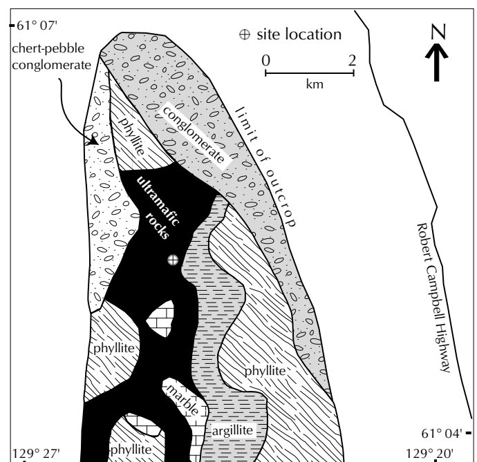
Figure 4. Simplified geological map of Frances Lake area with site location (modified from Murphy, 2001).
