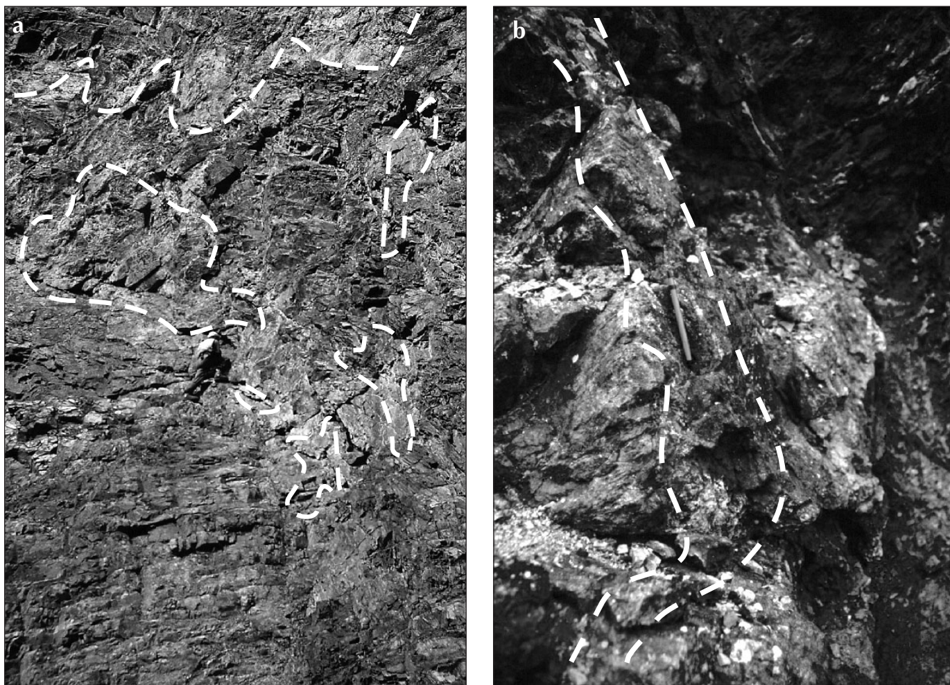
Figure 9. (a) Malachite-stained (area inside dashed lines) Fairchild Lake Group sedimentary rocks form the peak of Slab Mountain (person for scale). (b) A 10-cm-thick pyrite-chalcopryite-quartz-white mica vein (inside dashed lines) cutting carbonate-magnetite altered rock in the Canyon zone.
