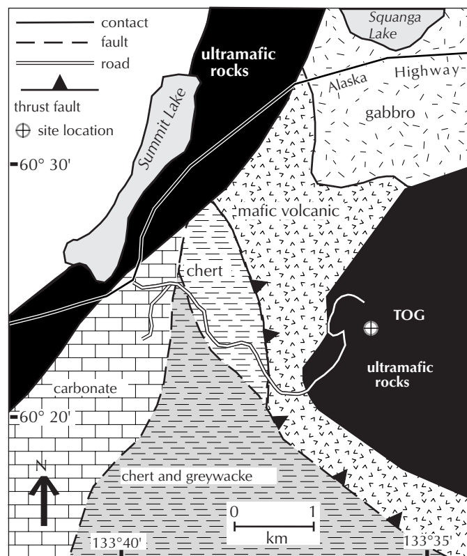
Figure 5. Simplified geological map of Tonnes of Gold area with site location (modified from Hart, 1996).
