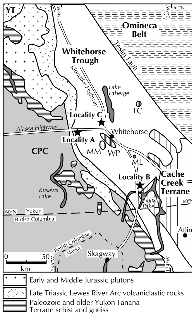
Figure 2. Generalized tectonic map of the south-central Yukon and collection Localities (A, B and C) for the Conglomerate formation of the Laberge Group (YT = Yukon-Tanana Terrane; CPC = Coast Plutonic Complex; MM = Mount McIntyre pluton; WP = Whitehorse pluton; TC = Teslin Crossing stock; ML = Mount Lorne stock).
