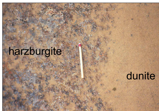
Figure 10. Coarse harzburgite with dunite lense from Atlin. Match is six centimetres.
