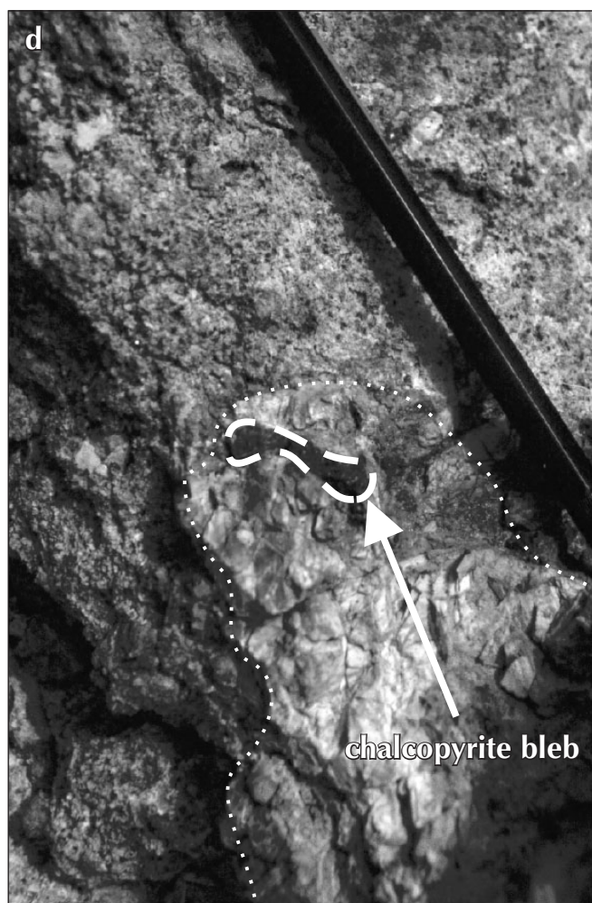
Figure 9. (c) Massive sulphide clast in Type 2 Wernecke Breccia at Slab Creek; (d) chalcopyrite bleb (dashed line) in a siltstone clast (dotted line) in Type 2 Wernecke Breccia on Slab Mountain.
