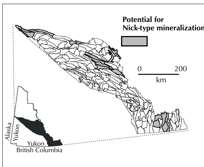
Figure 4. Map of Selwyn Basin displaying tracts that have potential for sedimentary-hosted nickel (Nick-type) mineralization.
