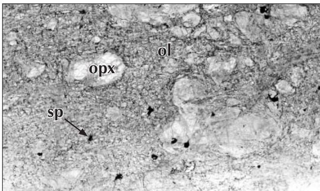
Figure 11. Plane-polarized light image of coarse harzburgite with olivine (ol), orthopyroxene (opx) and spinel (sp). Thin section is about 3.6 cm long by 2.1 cm wide.
