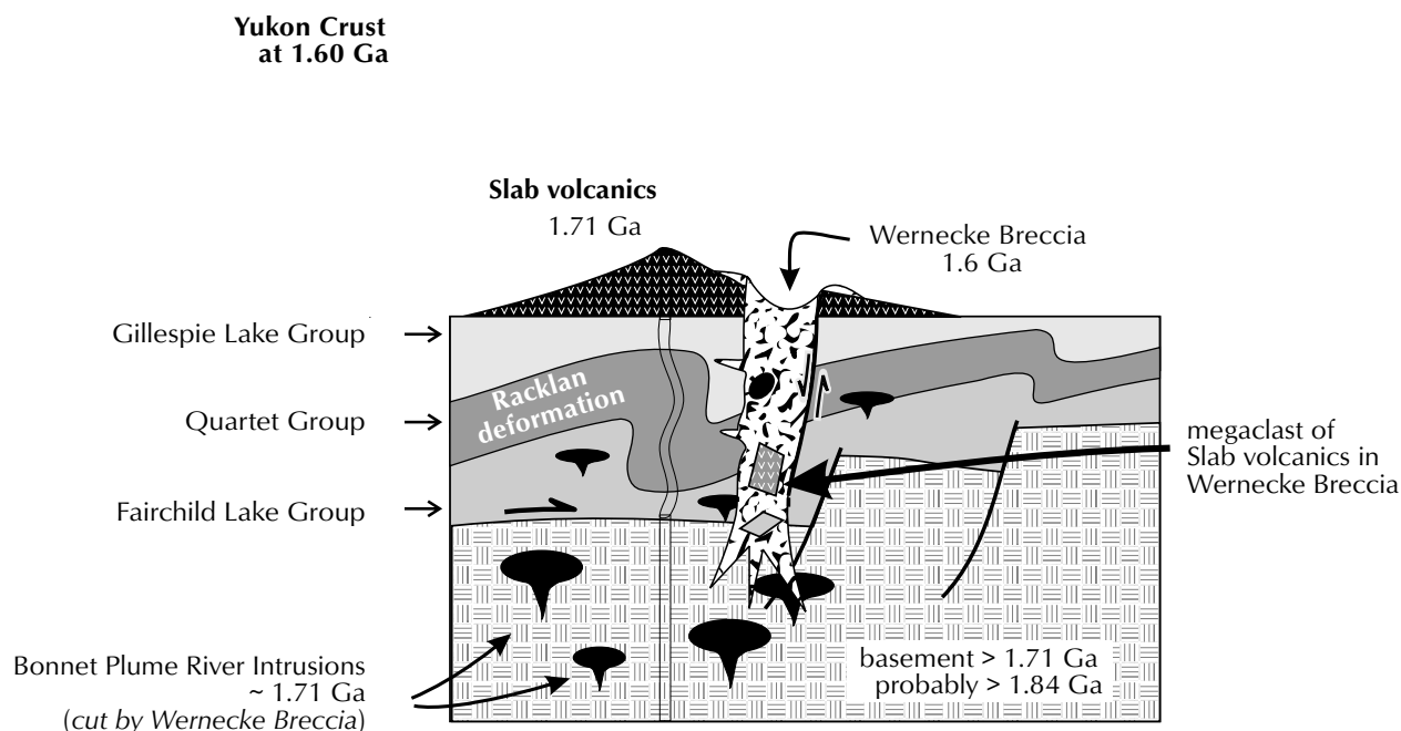
Figure 4. Cartoon illustrating a hypothetical crustal cross-section, showing relations between Wernecke Supergroup, Slab volcanics, Bonnet Plume River Intrusions and Wernecke Breccia (modified after Thorkelson et al., 2001a).
