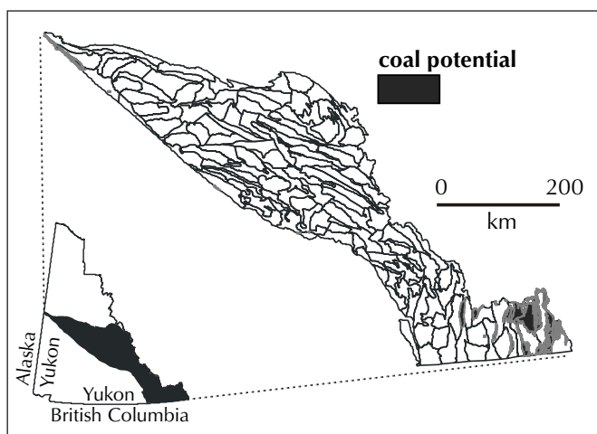
Figure 3. Map of Selwyn Basin displaying tracts that contain coal potential, showings, or deposits.
