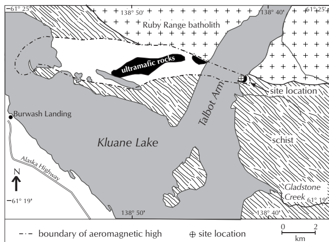
Figure 2. Simplified geological map of Kluane Lake area with site location (modified from Mezger, 2000).
