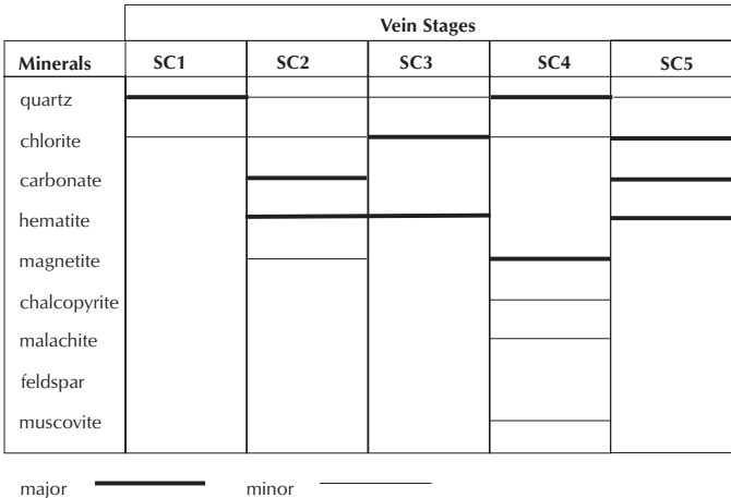
Figure 5. Sericite ± chlorite alteration zone - preliminary vein paragenesis.
