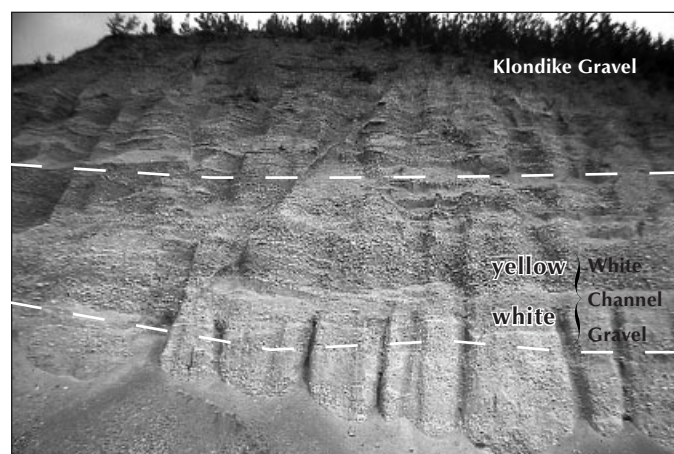
Figure 4. White Channel Gravel, showing the white gravel and yellow gravel sub-units and the overlying Klondike Gravel, Australia Hill.
