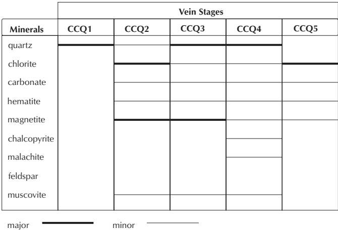
Figure 6. Chlorite-carbonate-quartz alteration zone – preliminary vein paragenesis.
