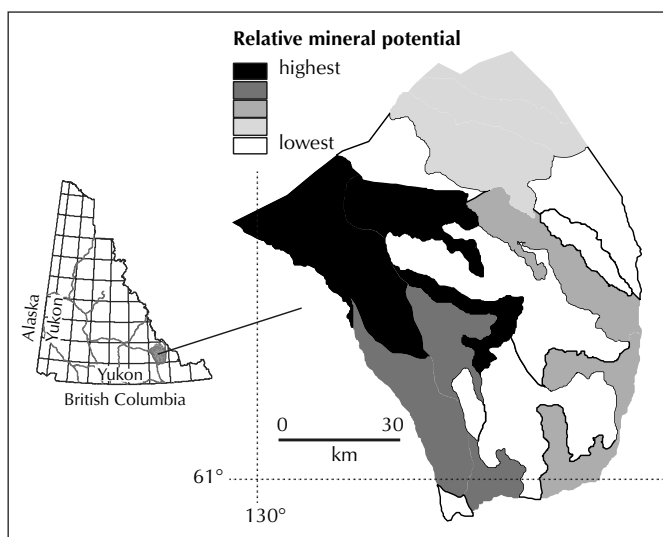
Figure 6. Detailed mineral potential map of central Frances Lake map area.
