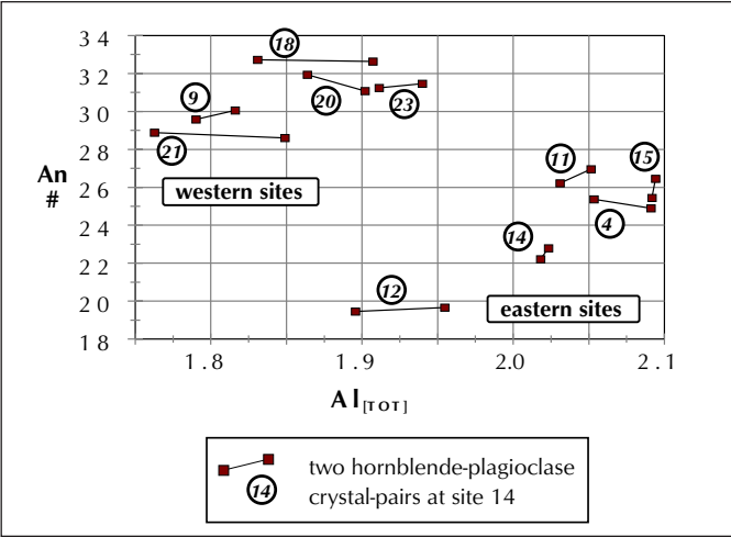
Figure 7. Plagioclase and hornblende crystal-pairs for each site plotted as calcium content in plagioclase (Anorthite # - An #) versus total number of aluminum cations (Al[TOT]) in hornblende. Within-site consistency is indicated by the similarity of pairs from each site.
