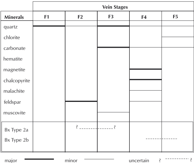
Figure 7. Feldspar alteration zone – preliminary vein paragenesis and inferred timing of Type 2a and Type 2b breccia emplacement. Bx = breccia.
