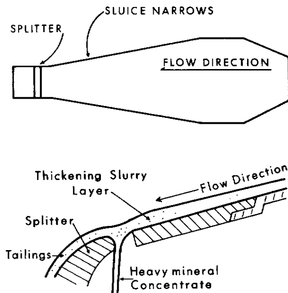
Figure 5: Plan and cross-sectional diagrams of a pinched sluice, showing the separation of high density material from low and medium density material at the end of the sluice.
