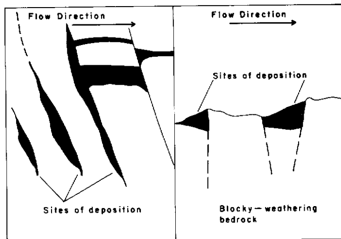
Figure 9: Sites of gold deposition behind obstructions in the bedrock surface. A plan view is at left, and a cross-section is at right.
