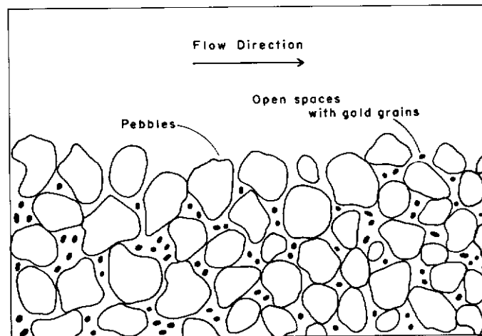
Figure 13: Cross-section of gravel deposits with little matrix. The open spaces between clasts are sites of gold deposition.
