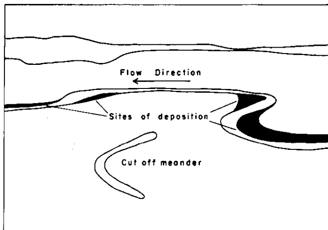
Figure 3: Sites of gold deposition along the inside of meander curves. Gold is also deposited on the ends of sand and gravel bars in braided streams.
