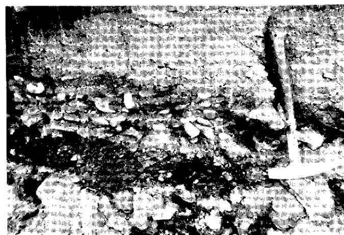
Figure 12: View of gravel section with black manganese stain where little matrix is present between the pebbles.
