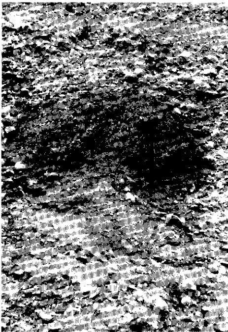
Figure 26: Granodiorite boulder in White Channel gravel along the Klondike River. The boulder is almost completely decomposed and is held together solely by the gravel surrounding it.
