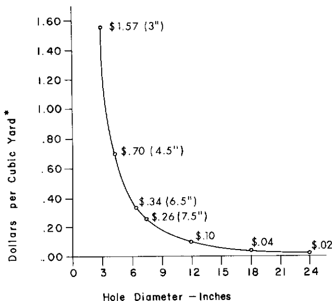
Figure 32: The effects of one stray 1 mg (.00003 oz.) particle of gold on grade calculations from drill holes of various diameter (after Wells, 1973).
