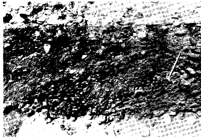
Figure 27: Quartz-rich gravel at Dominion Creek. Deposits for the 50 cm (20 inches) above bedrock are stained by iron oxides.
