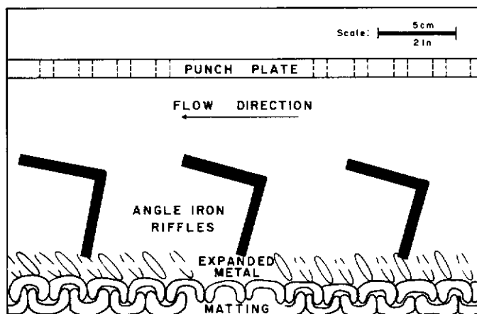
Figure 37: Schematic cross section of punch plate, riffles, expanded metal, and matting in a sluice box.
