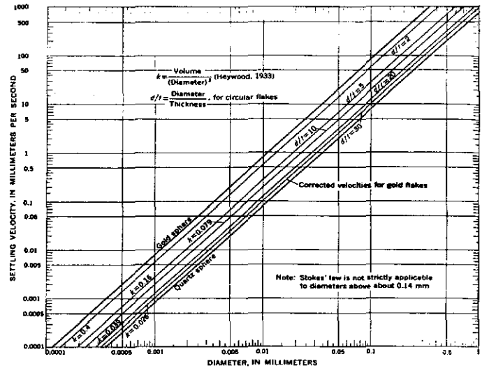
Figure 3: Chart showing settling velocities in water of gold grains of various degrees of flattening, and quartz (after Tourtelot, 1968).
