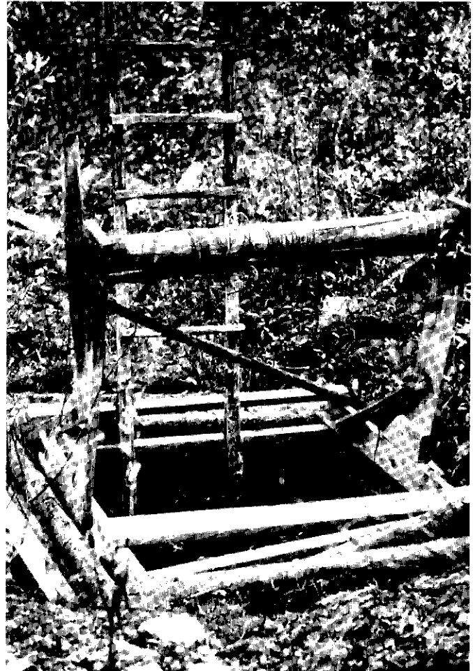
Figure 31: Mouth of hand-dug test shaft along Bear Creek. A bucket hung from the windlass was used to bring gravel from the shaft to surface.
