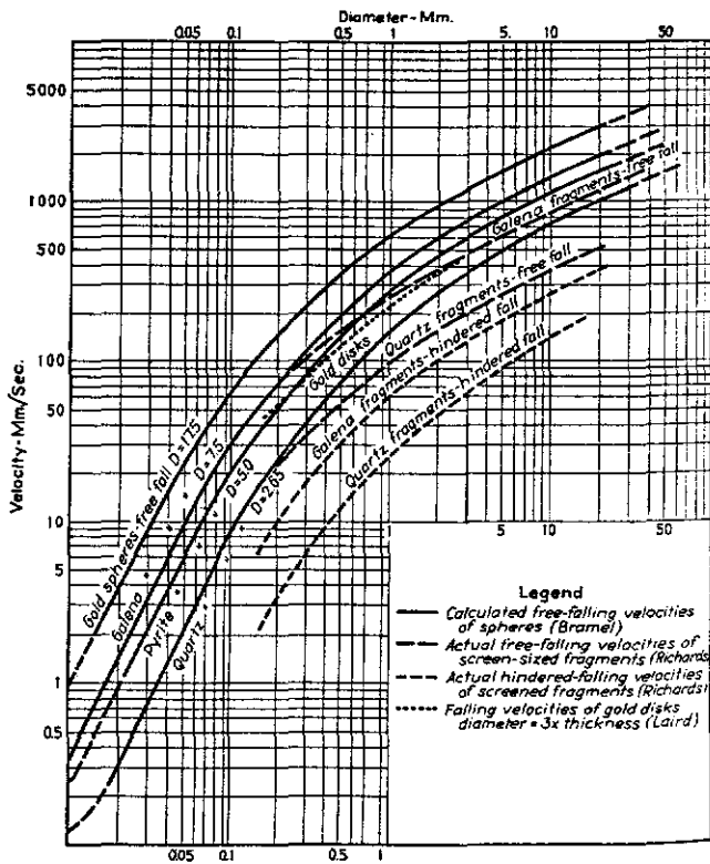
Figure 2: Chart showing settling velocities in water of gold, galena, pyrite, and quartz grains of various sizes and shapes (after Hague, 1940).
