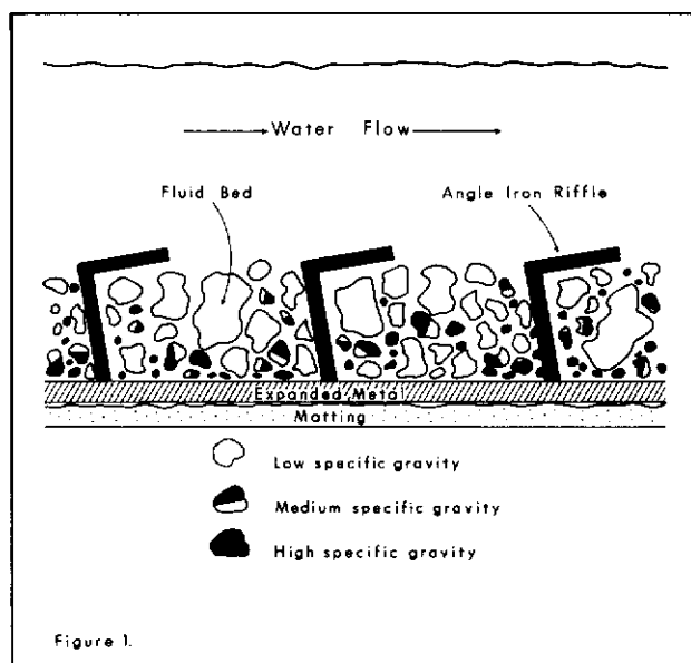
Figure 1: Cross Section of riffles in sluice box.
