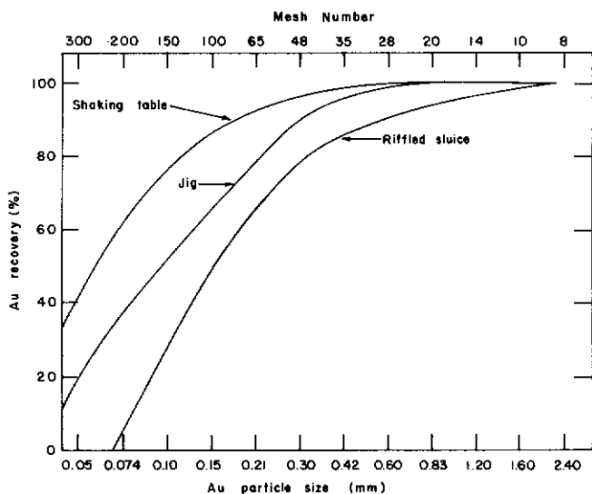
Figure 6: Recovery rates of fine-grained gold for sluice box, jig, and shaking table (after Wang, 1979).
