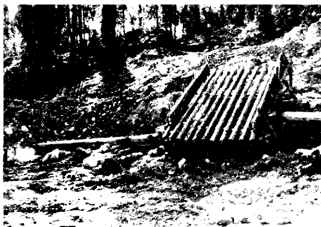
Wooden grizzly and sluice box at the M. Pilote property, McLagan Creek.
