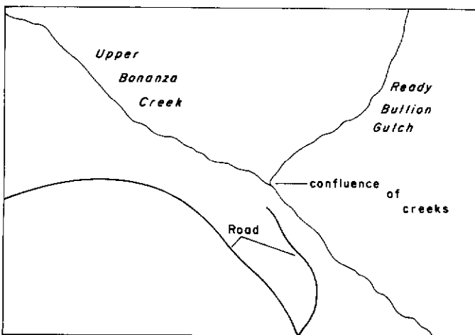
Figure 7: Site of gold deposition downstream from the confluence of Ready Bullion Gulch and upper Bonanza Creek.
