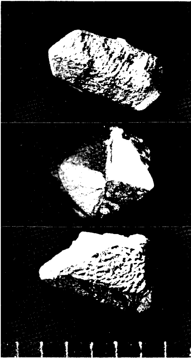
Figure 25: Crystalline gold recovered from placer deposits at Bear Creek. The scale markings are 1 mm (.04 inches) apart.
