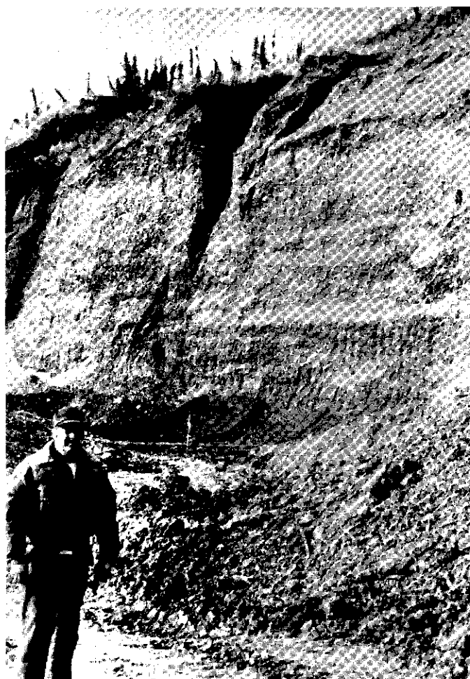
C. Brisebois at his cut along the left limit bench of Sixty Mile River. Colluvium at the top of the cut is slightly darker than the underlying gravel and silt horizons. The layer immediately above bedrock, which is mostly hidden by stockpiles of gravel in this photograph, is gold-bearing.
