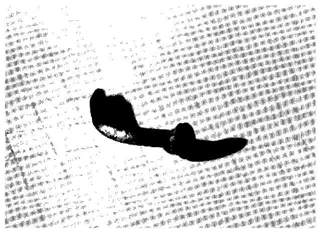
Figure 28: Copper nail recovered from old underground workings on Miller Creek. A thin plating of gold covers the convex side of the bent nail. The spaces on the grid paper are 5 mm (.2 inches) apart.
