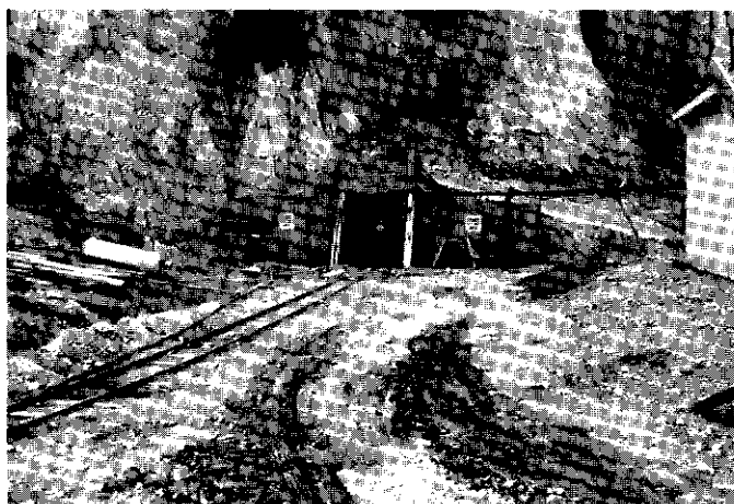
Portal of underground mining operation at Dago Hill during 1981. The miner is using a compressed air-powered locomotive and side-dumping car on tracks to haul gravel to a stockpile.
