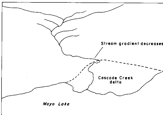
Figure 5: Site of gold deposition at the apex of the Cascade Creek delta, where the stream gradient decreases.
