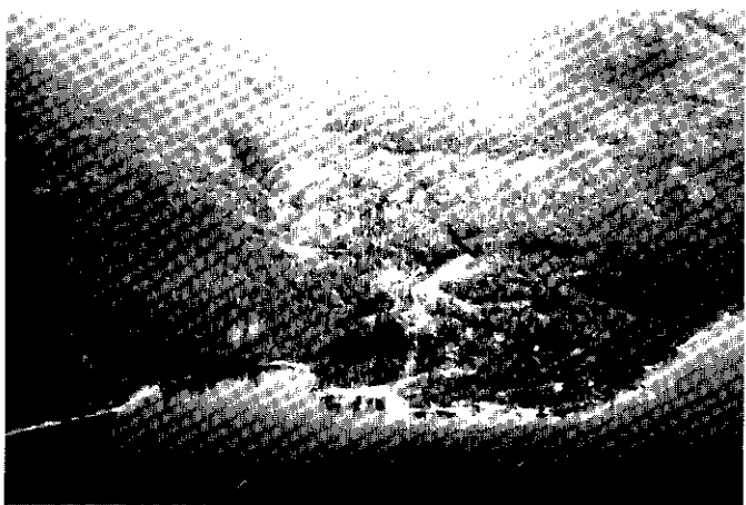
Figure 4: View of delta at the mouth of Cascade Creek on Mayo Lake.
