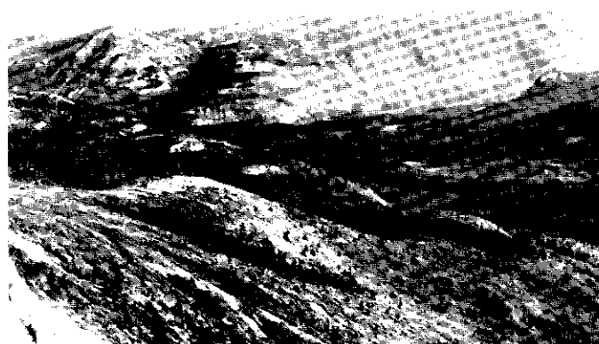
Figure 17: The ridge in the distance of the photograph comprises a remnant of pre-glacial valley-and-ridge topography in the glaciated terrain at Long Lake, 48 km (30 miles) north of Whitehorse.
