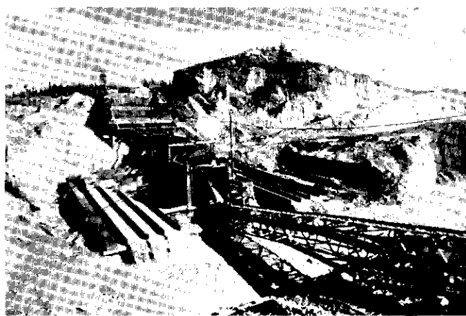
Processing unit at Miben Mining Company operation at Dago Hill during 1981. Gravel from the hopper being fed by the bulldozer at top left is washed into the trommel, from which oversized material is transported to tailings by the conveyor belt in the foreground, and undersized material is sluiced in the parallel sets of sluice boxes. This processing unit was built from parts salvaged from two old dredges, and an asbestos mine.
