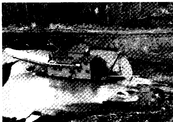
View of the Queenstake Resources Ltd. dredge in 1982. The bucket line at the right of the dredge is digging gravel from the creek bed and transporting it to the trommel inside the dredge. Oversize from the trommel is being dumped on a tailings pile by the stacker at the left of the dredge. Undersize from the trommel is being sluiced. Tailings from the sluices are being dumped from the small tail races at the left of the dredge in part, and in part are being pumped out the stacker with the coarse tailings.
