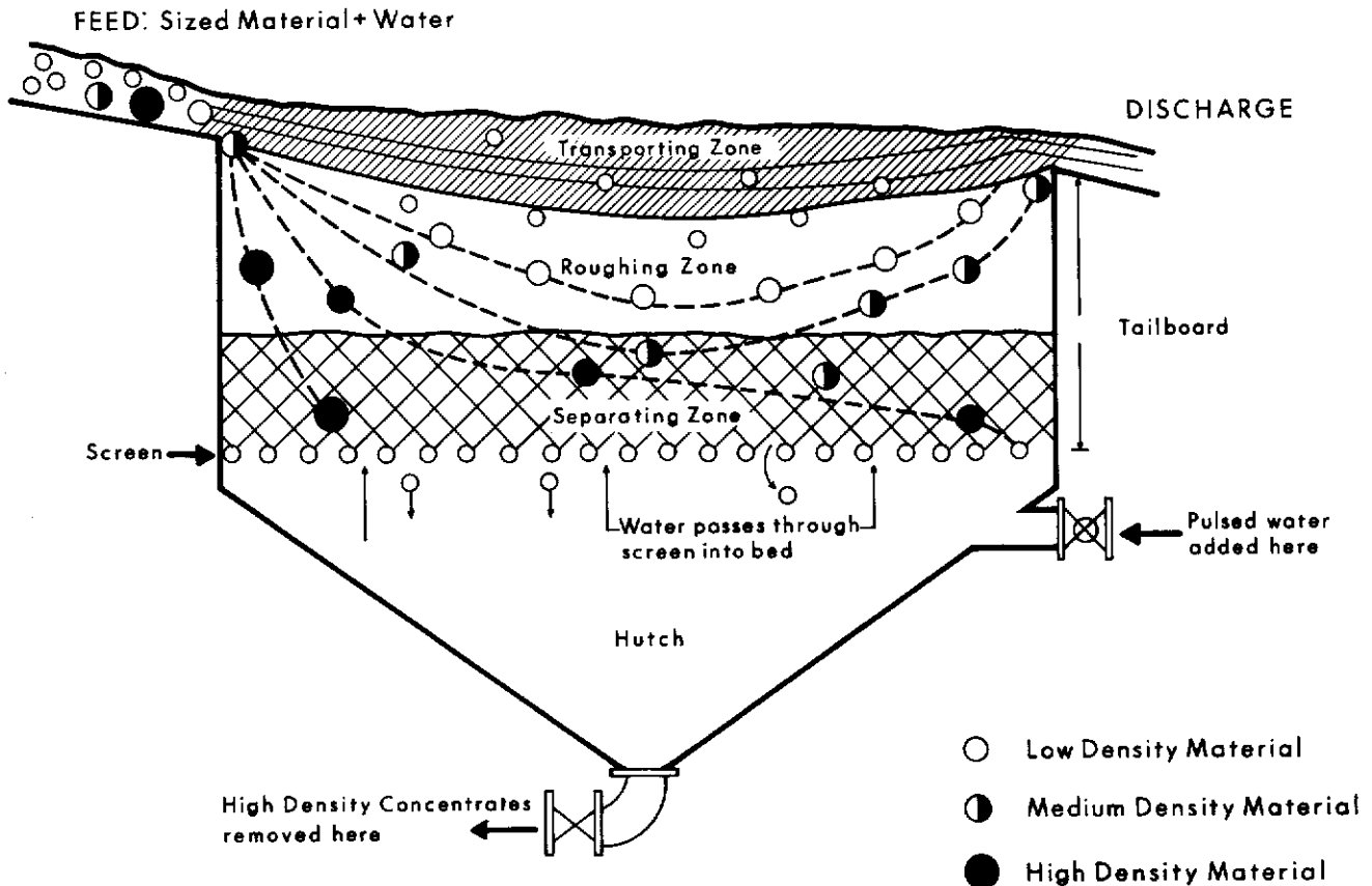
Figure 4: Cross-sectional diagram of a jig, showing the paths of particles of various densities.
