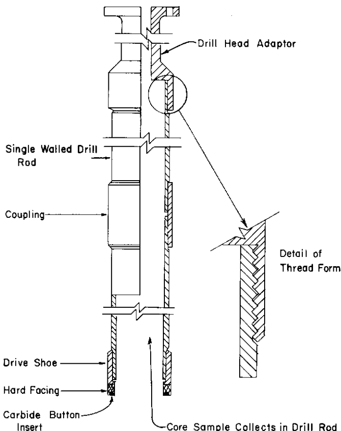
Figure 3: Drill rod column and bit of Hawker Siddeley Canada Inc. Sonic drills.
