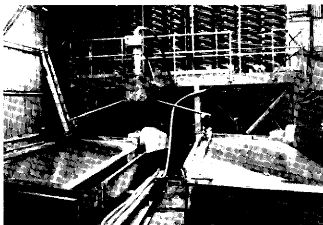
View of spiral concentrators and separation tables at Canada Tungsten Mining Corp. Ltd. Dublin Gulch mining operation. The dark areas on the tables are covered by a mixture of heavy minerals and water.
