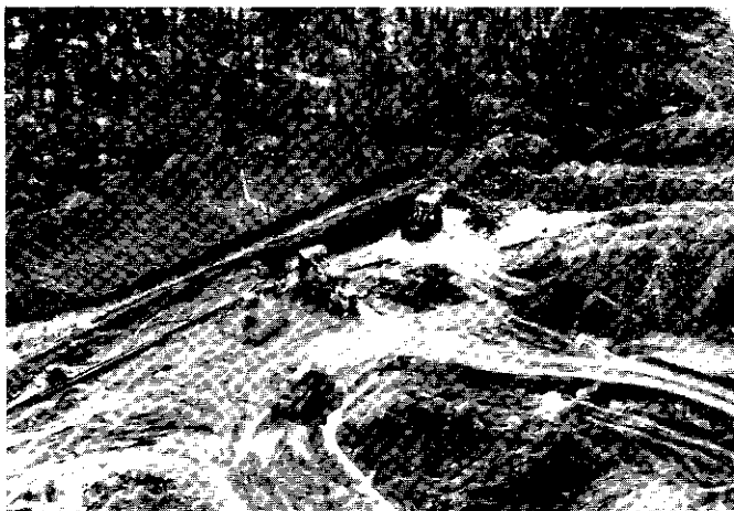
View of mining operations at the Blackstone Placer Mining Ltd. property of Clear Creek in 1982. A bulldozer is being used to mine the gravel and move it to a stockpile. A loader is being used to feed the sluice box. Tailings are being removed by a second loader.
