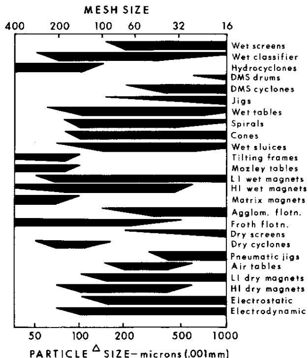
Figure 7: Grain size range applicability of commercial gravity concentrating units.
