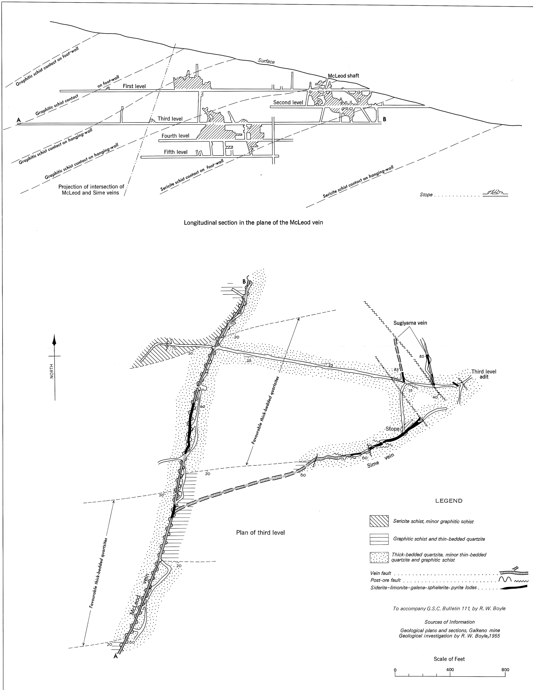
Figure 13. Plan and longitudinal section, Galkeno mine, Galena Hill, Yukon Territory
