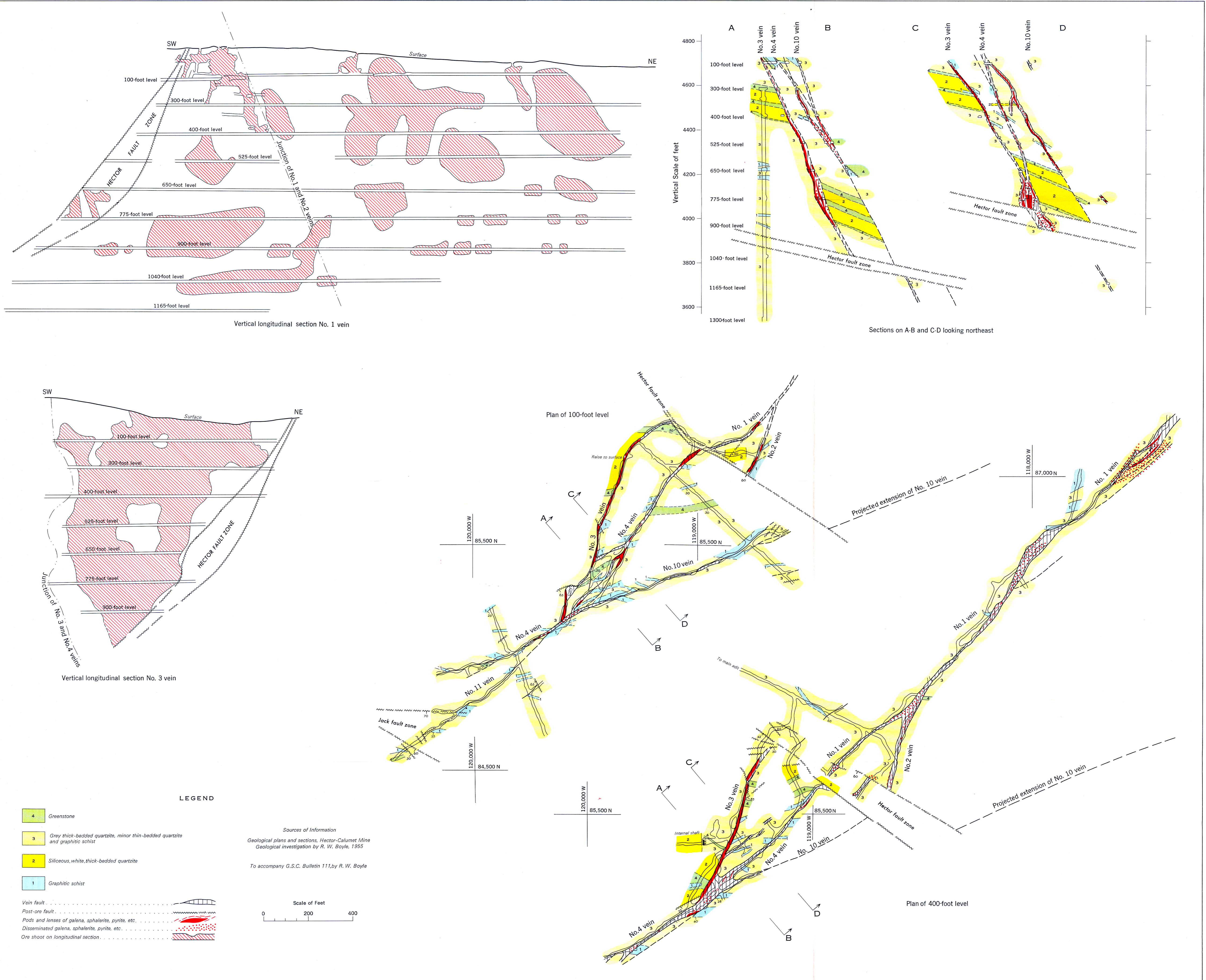
Figure 14. Plans and sections, Hector-Calumet Mine, Galena Hill, Yukon Territory
