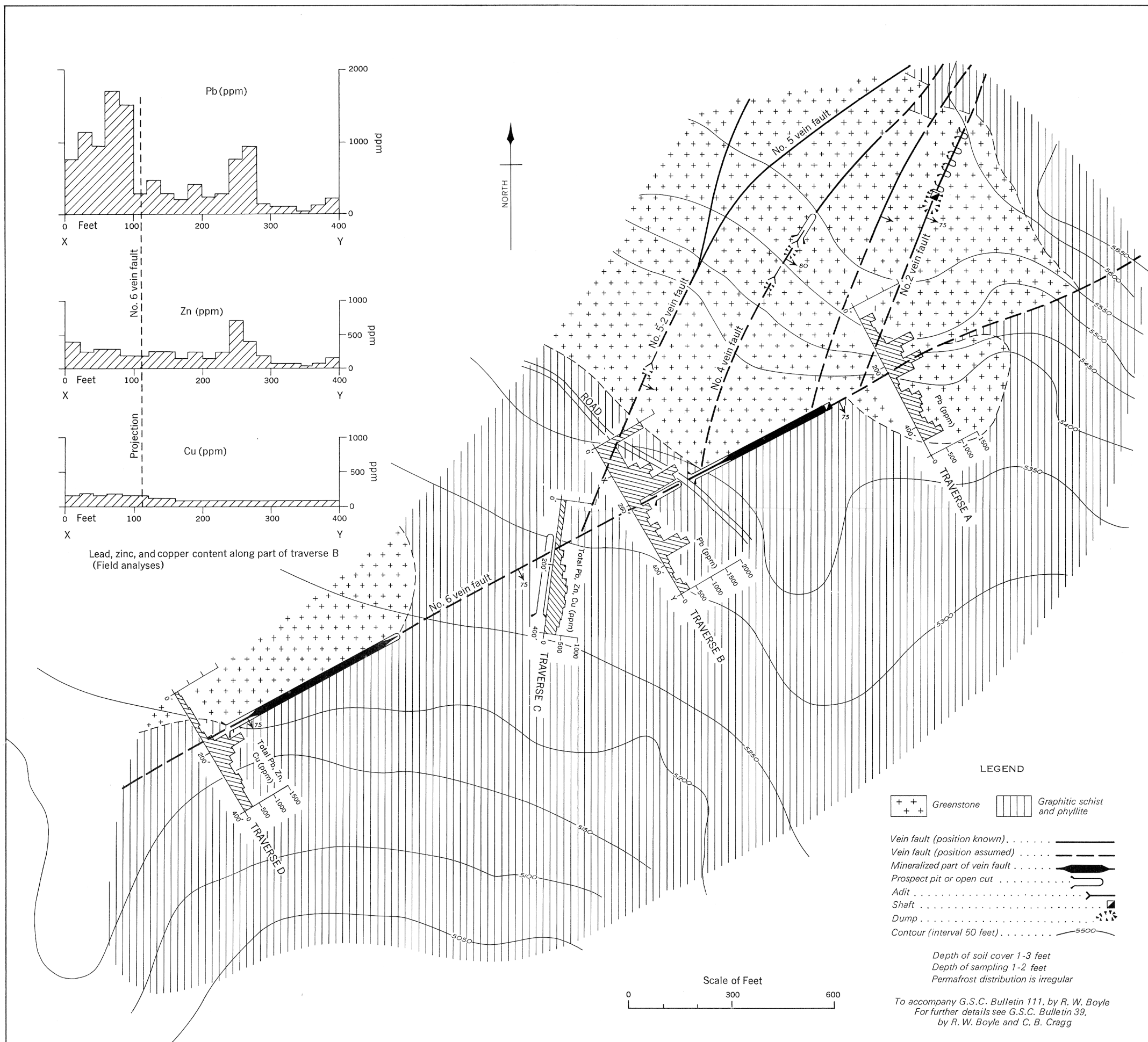
Figure 20. Heavy metal content of soil, No. 6 vein fault, Keno Hill, Yukon Territory
