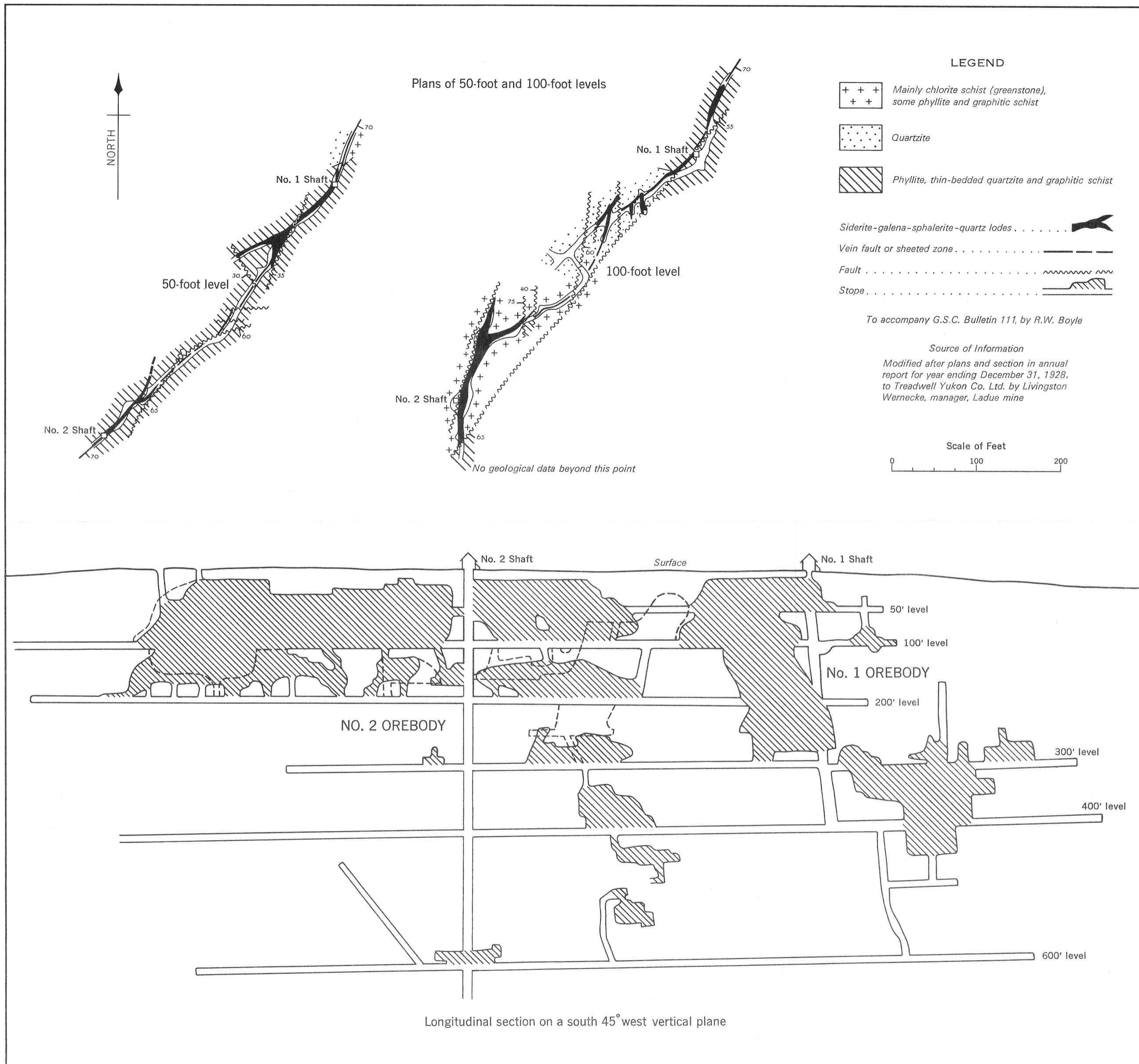
Figure 6. Plans and longitudinal section, Ladue mine, Keno Hill, Yukon Territory
