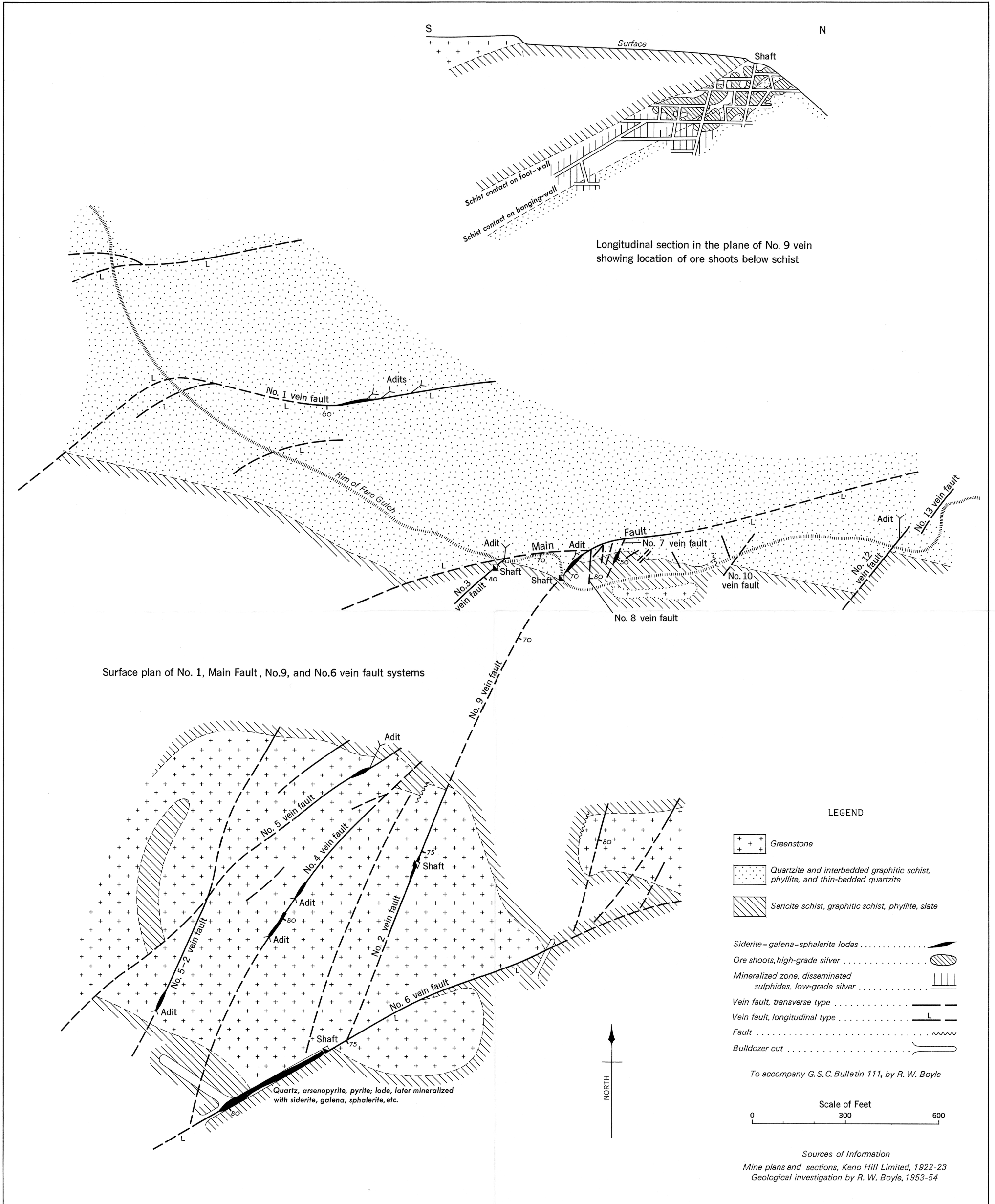
Figure 9. Surface plan of No.1, Main Fault, No.9, and No.6 vein fault systems, and longitudinal section in the plane of No.9 vein, Keno Hill, Yukon Territory
