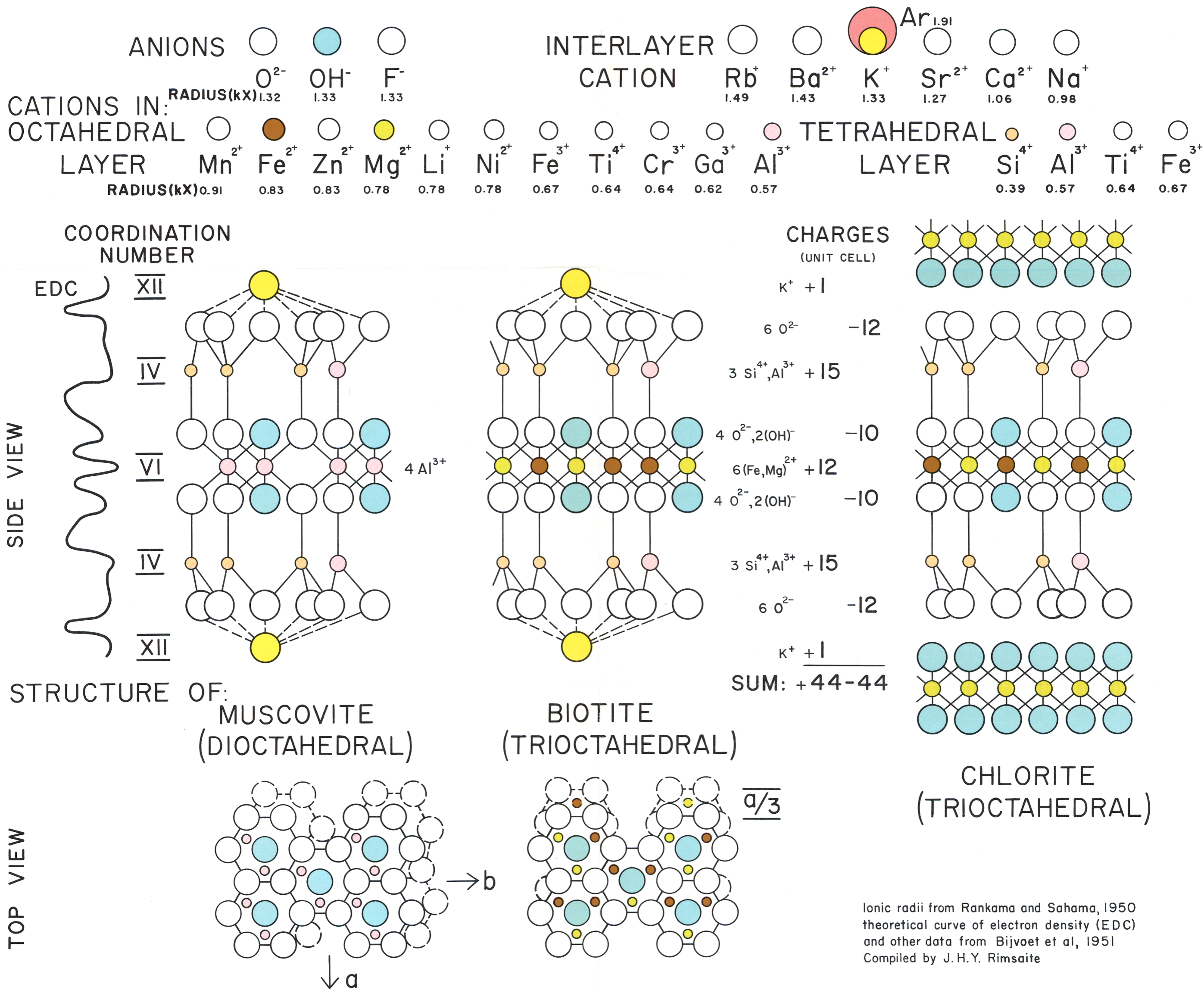
Figure 3. Diagrammatic representation of muscovite, biotite, and chlorite structures
