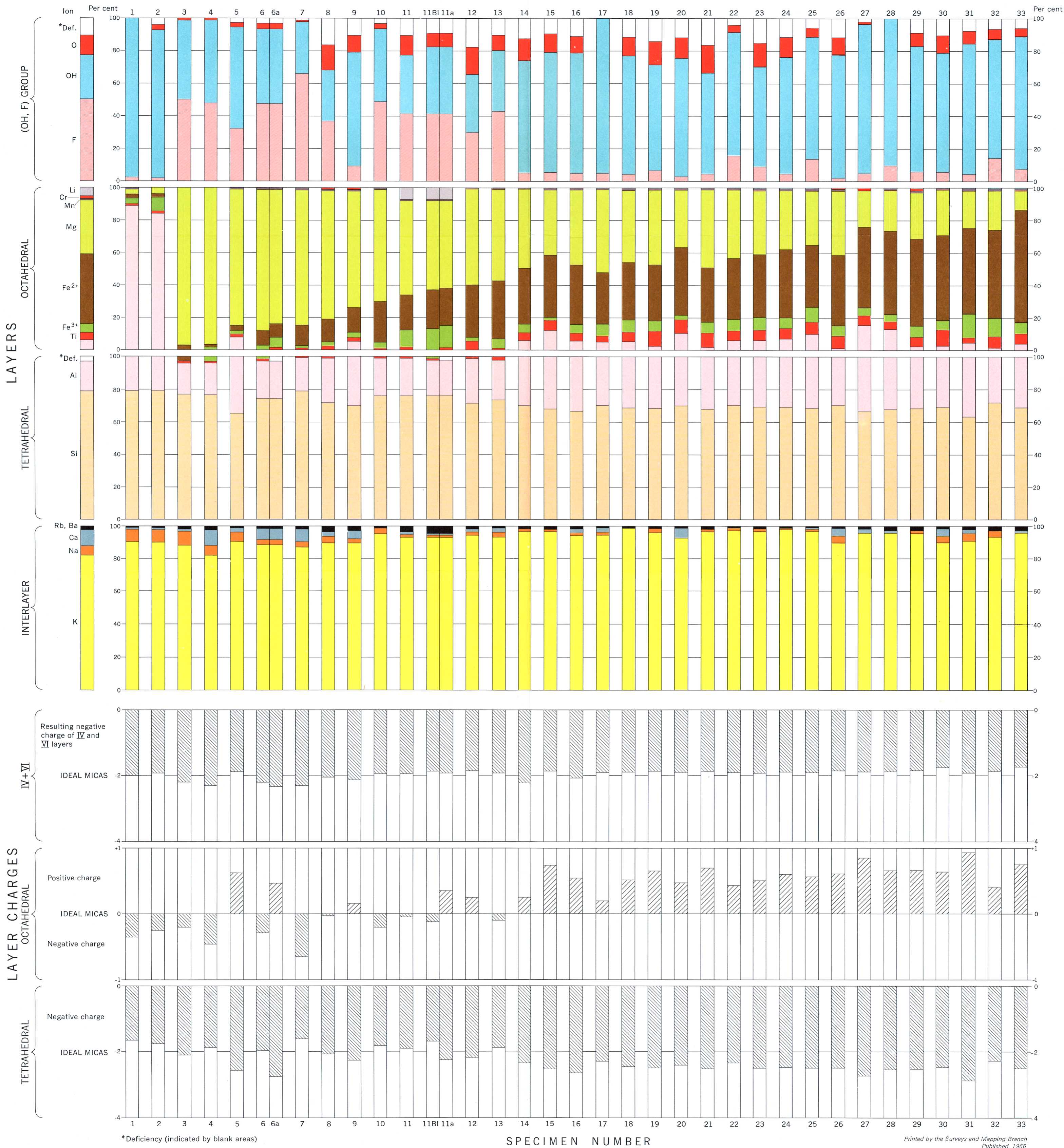
Figure 5. Percentage occupancy of layers and layer charges of micas
