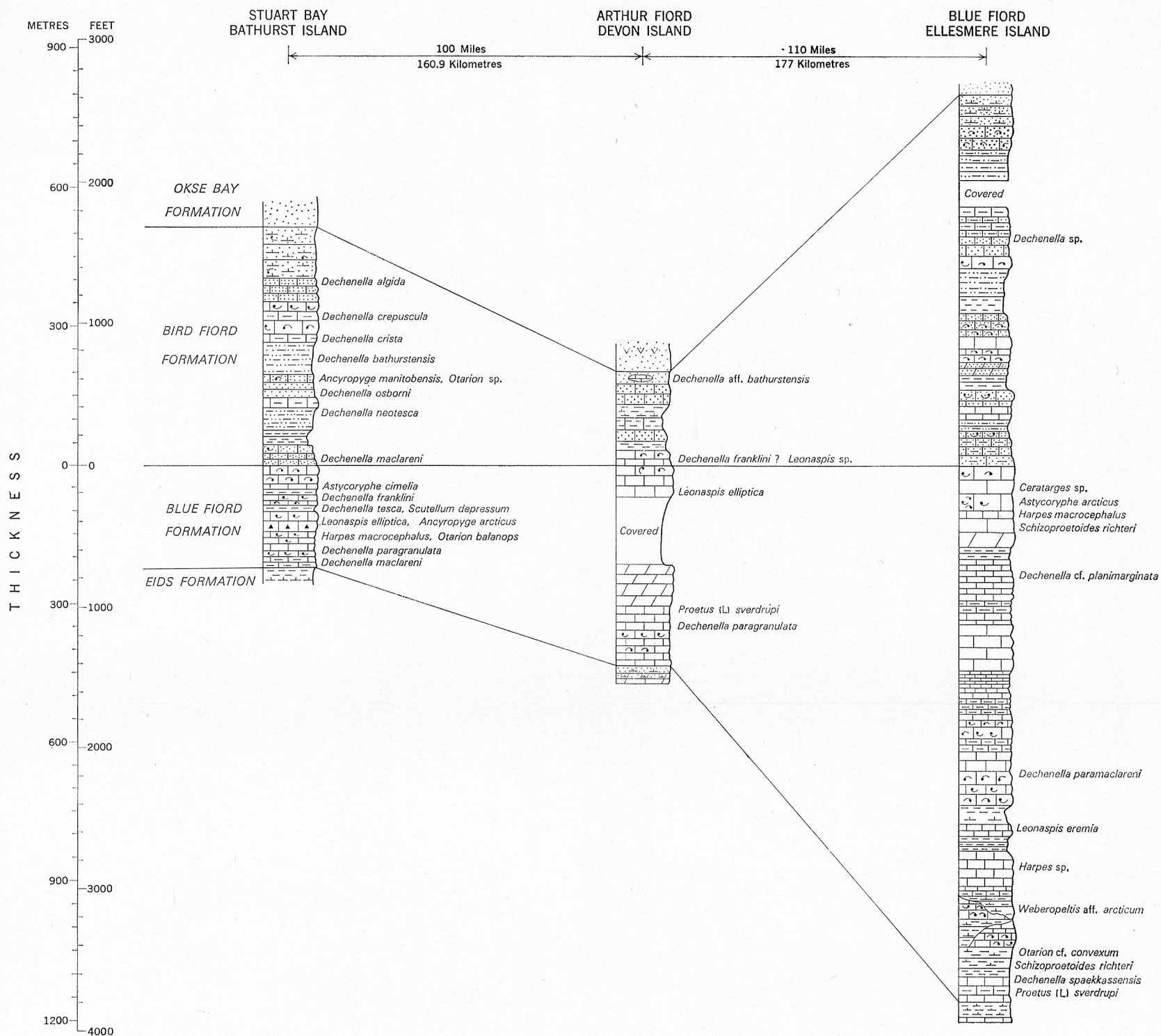
FIGURE 5. Distribution of trilobite species in the Blue Fiord and Bird Fiord Formations.
