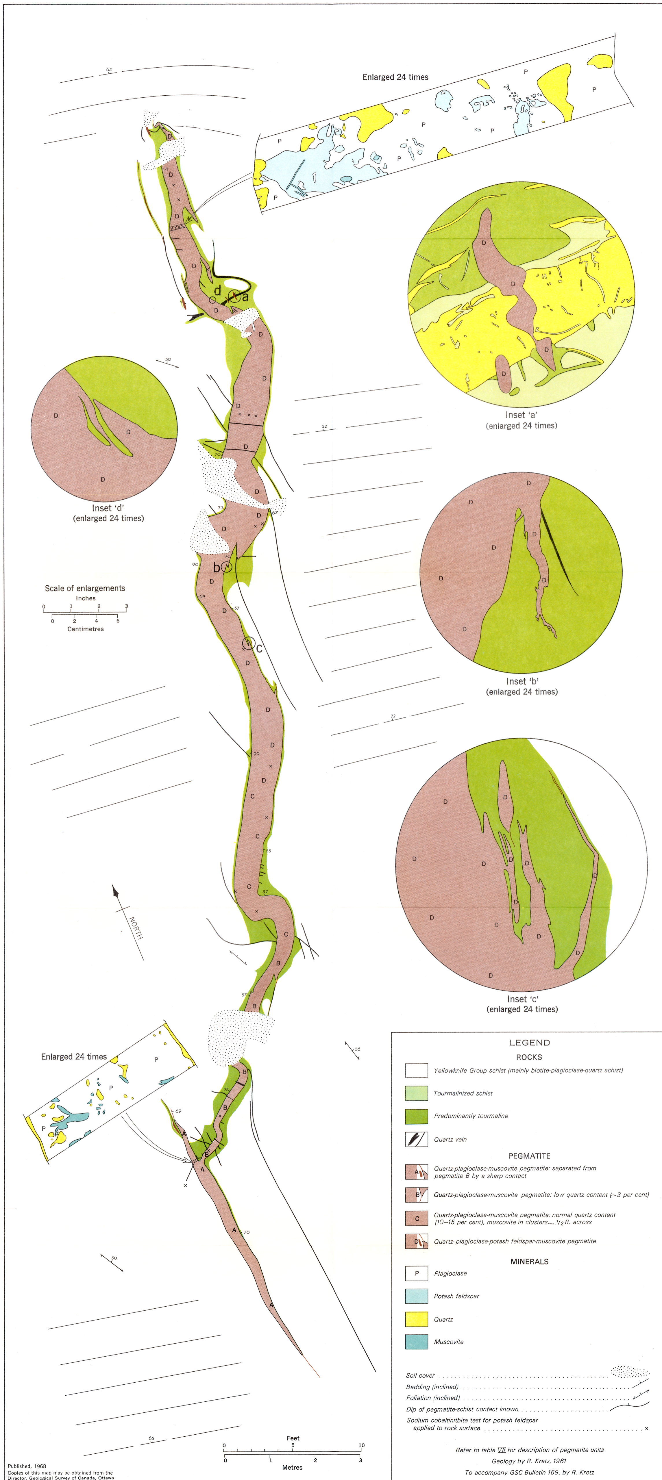
Figure 14. Detailed map of pegmatite dyke in schist, Sparrow Lake-Thompson Lake area, District of Mackenzie. (Site 372, Figure 4)
