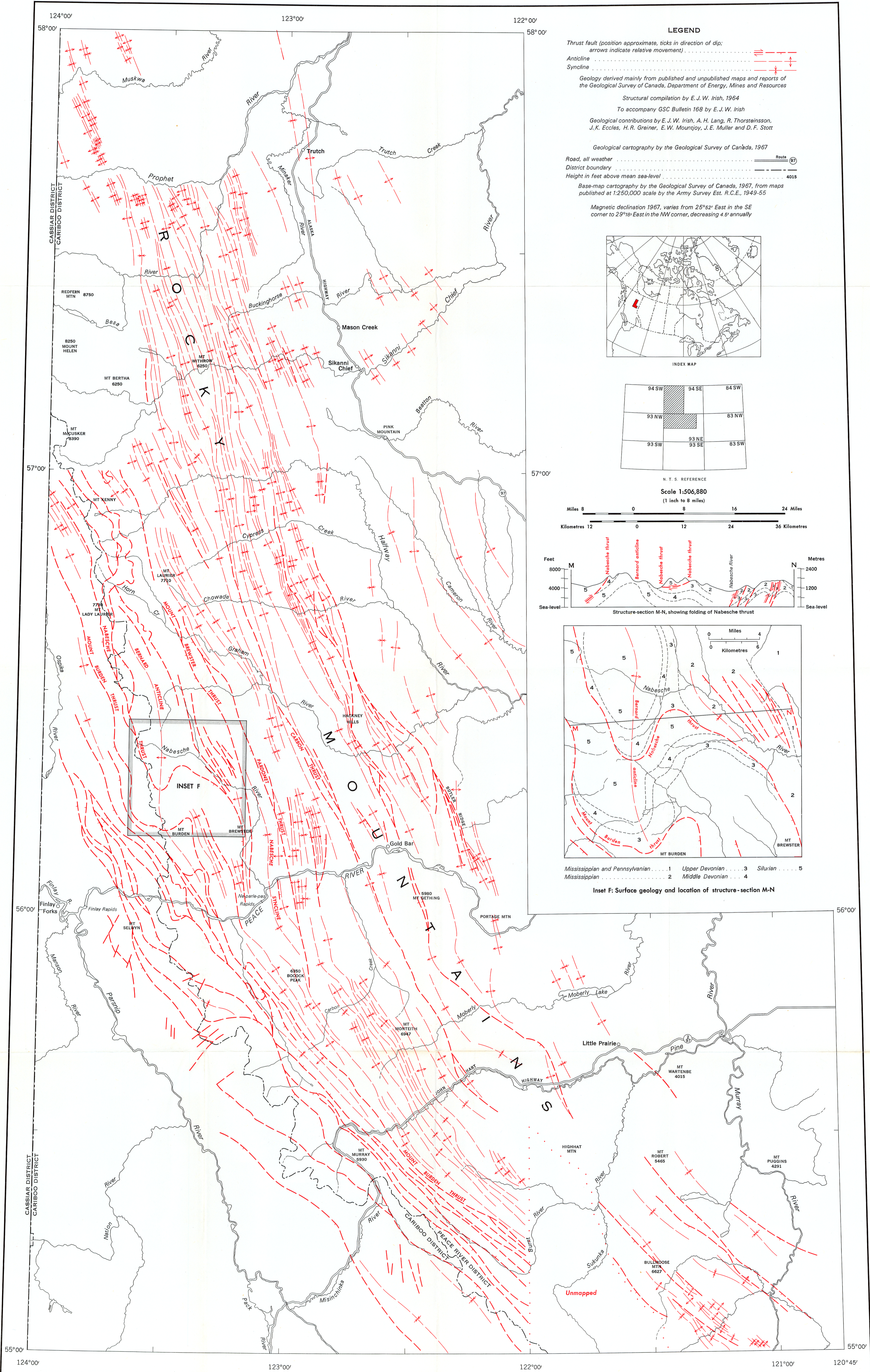
Figure 2. Tectonic map of part of northeastern British Columbia
