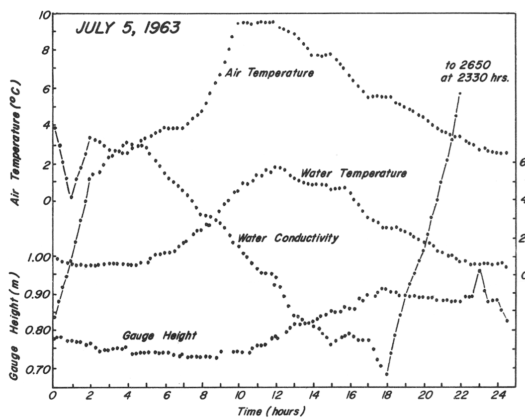
Figure 21. Air temperature and water characteristics for selected 24-hour periods at Lewis River:
