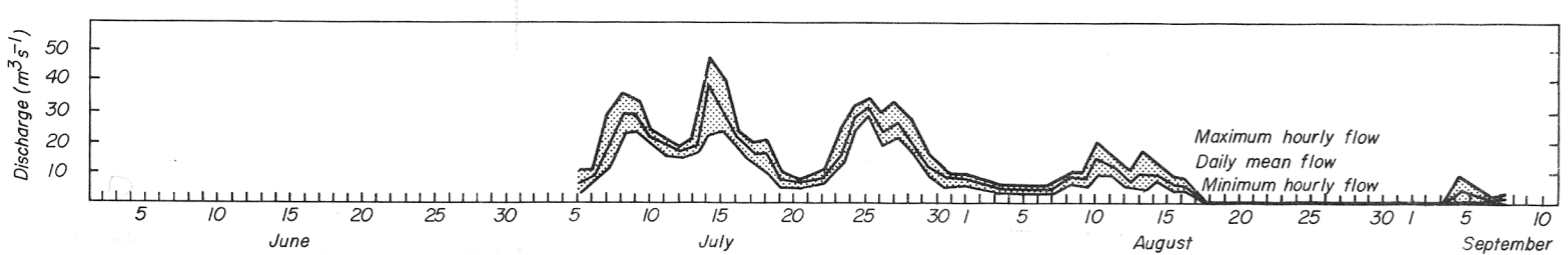
Figure 15. Summary of runoff and weather at Ekalugad valley: 1967-1968 (South River runoff data only given for 1968).
