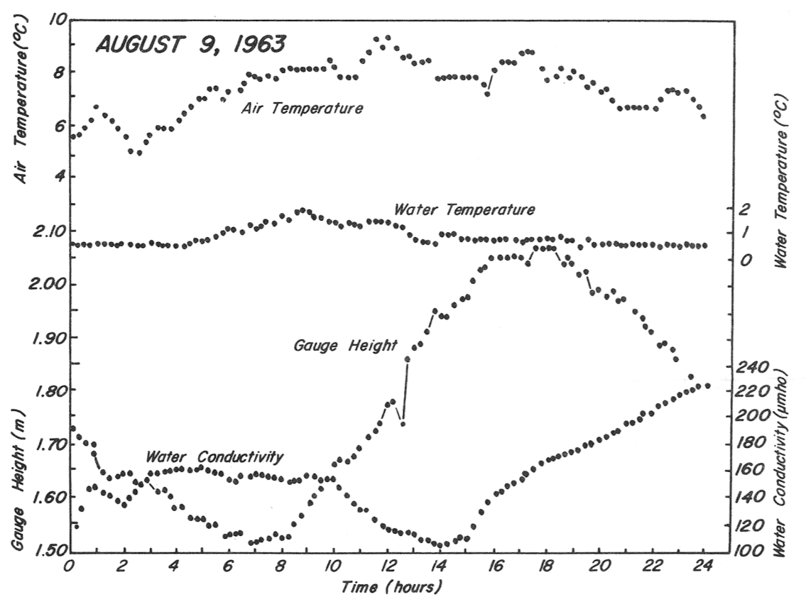
Figure 21. Air temperature and water characteristics for selected 24-hour periods at Lewis River:
