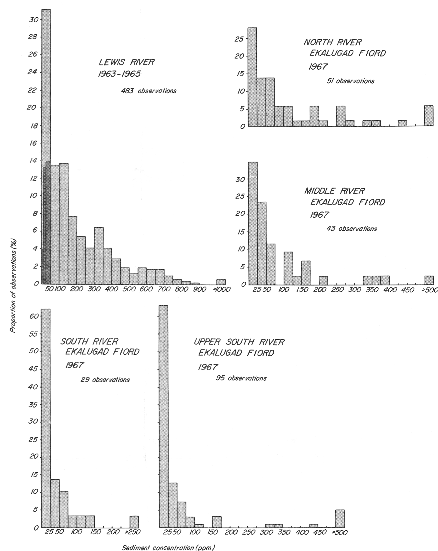
Figure 33. Distribution of suspended sediment load concentration from sample observations.
