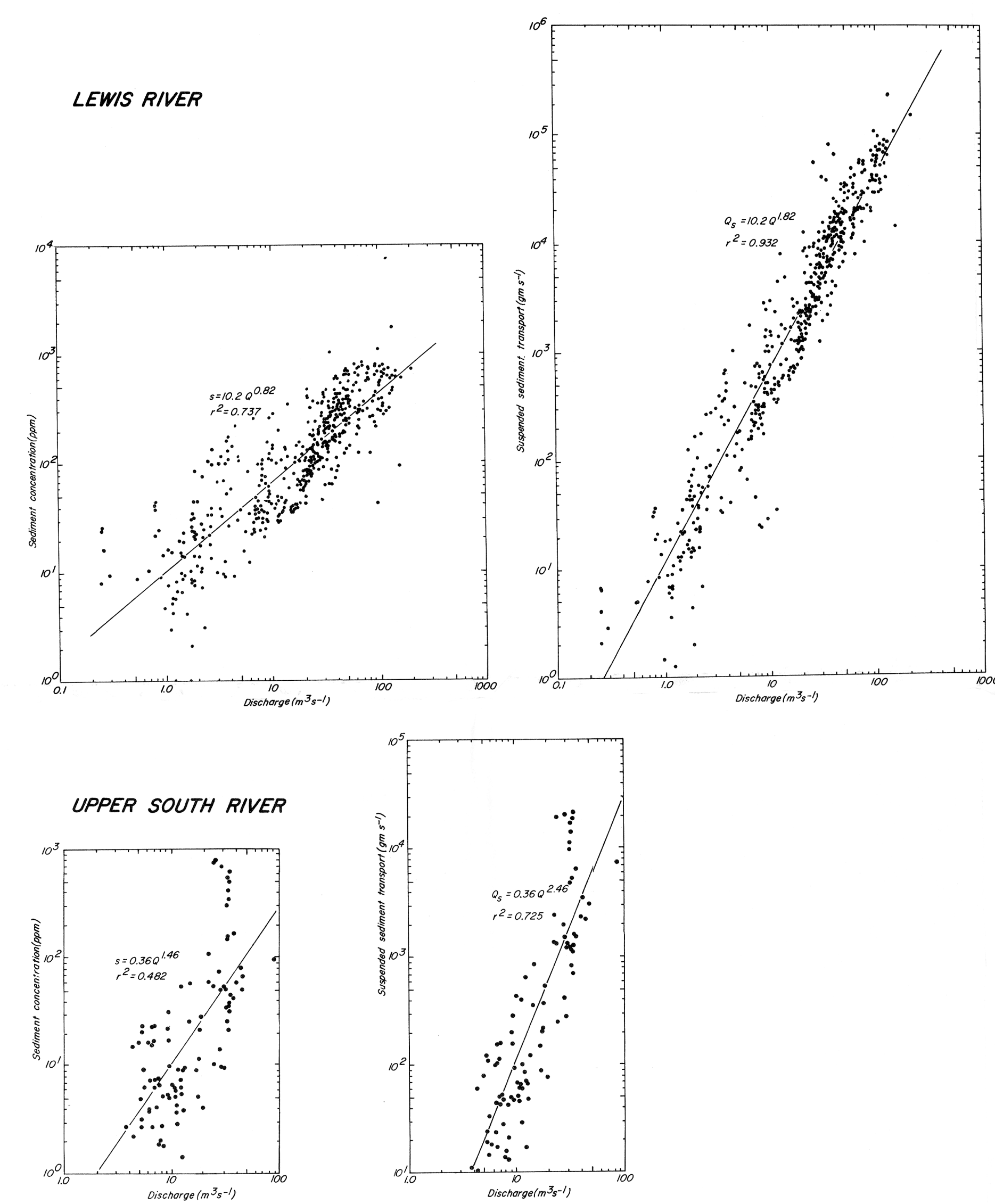
Figure 34. Examples of suspended sediment relations: concentration and transport of suspended sediment, and discharge in Baffin Island streams. A. Lewis River, 1963-1965 B. Upper South River, Ekalugad Fjord, 1967
