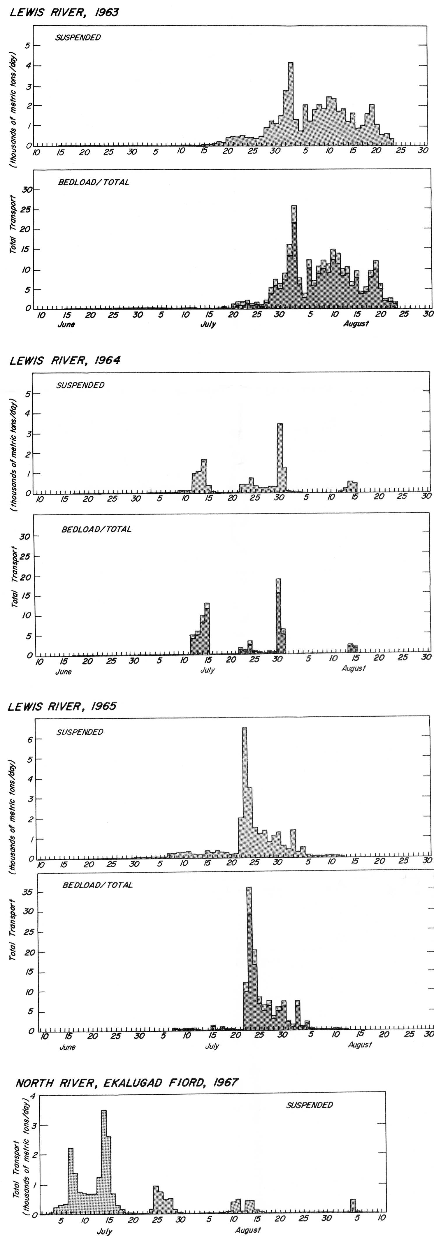
Figure 40. Daily sediment transport.
