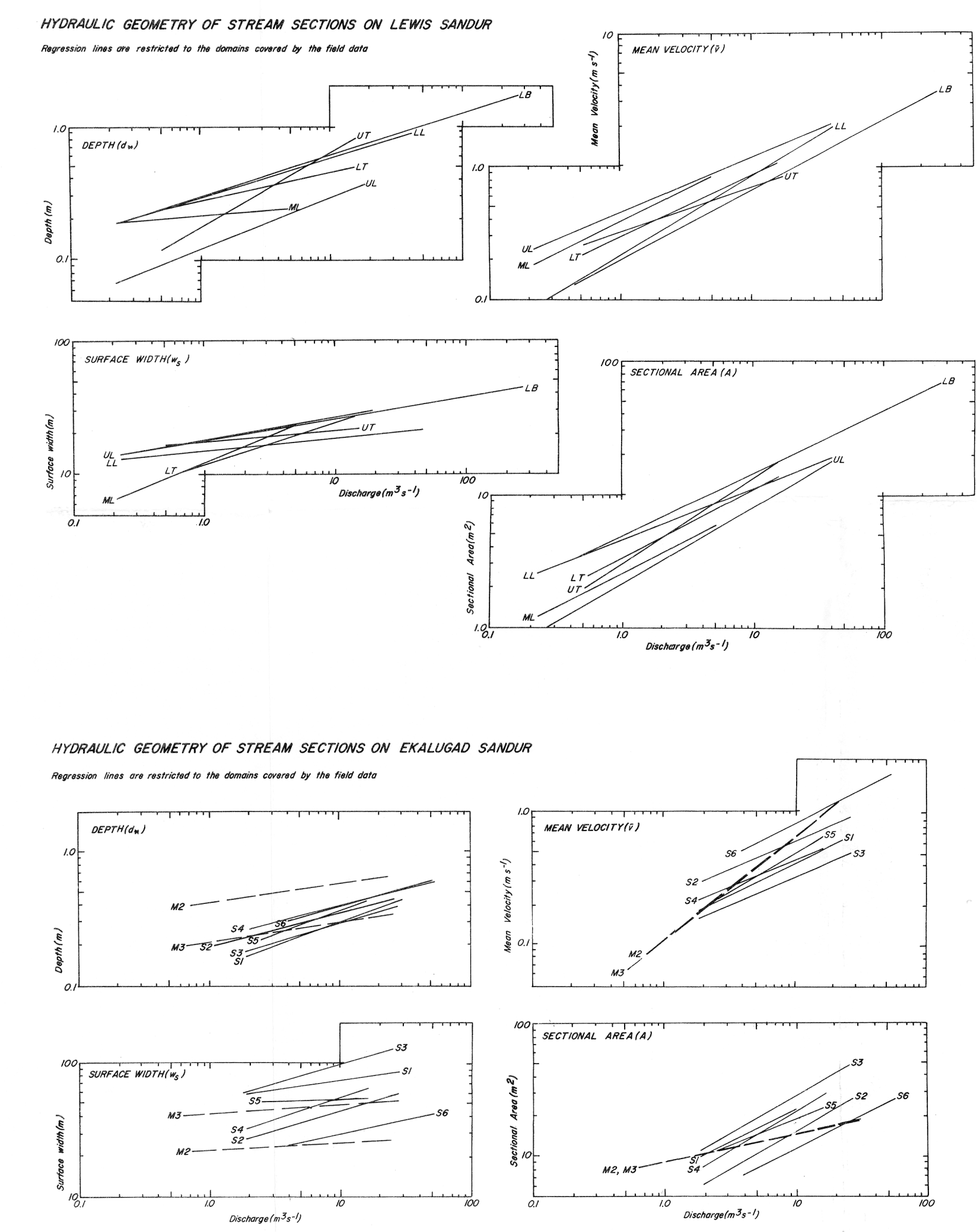
Figure 44. Hydraulic geometry of stream sections (regression lines are restricted to the domains covered by the field data). A. Lewis sandur B. Ekalugad sandur
