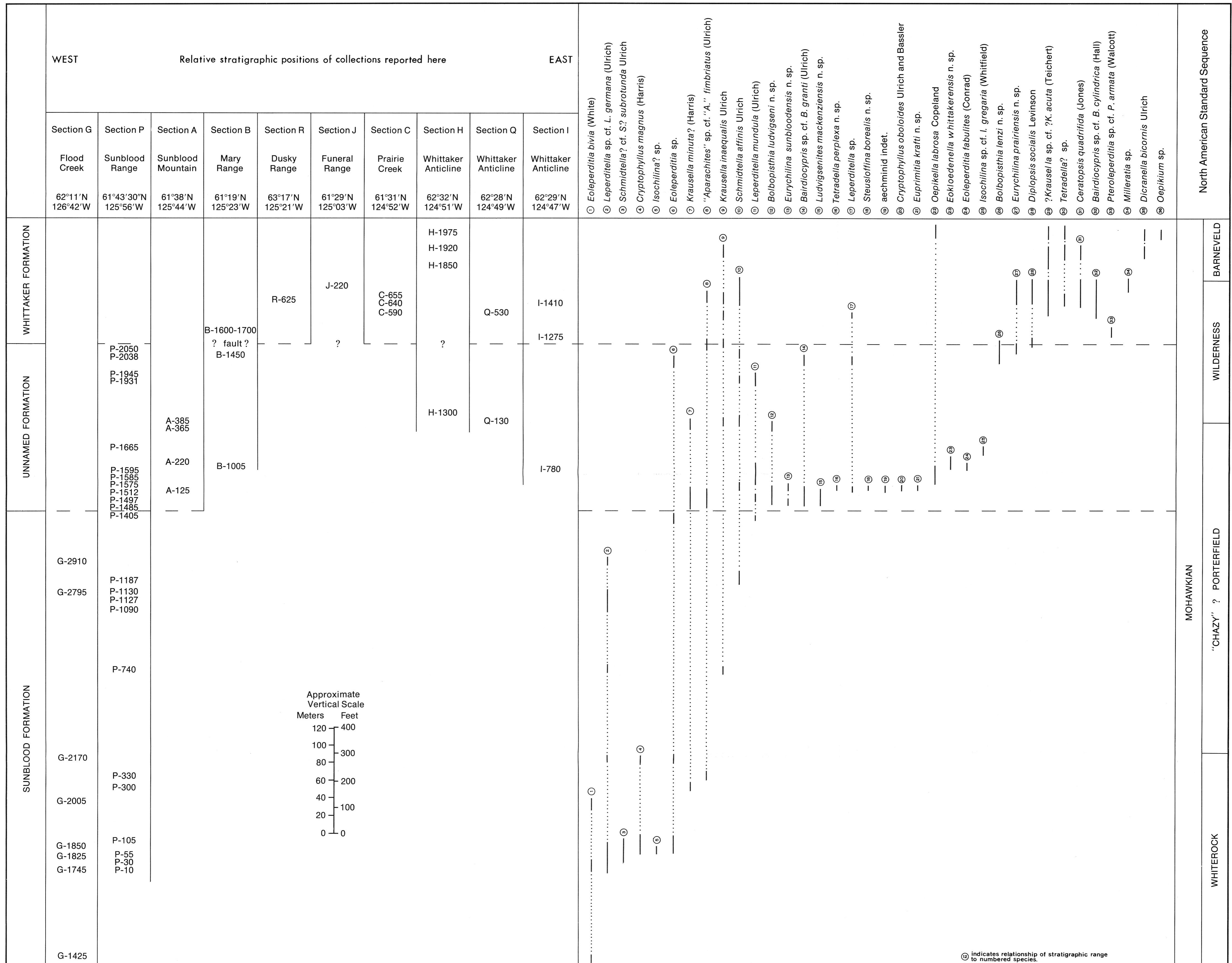
Text-Figure 3. Stratigraphic occurrence of Middle Ordovician ostracodes, southwestern District of Mackenzie
