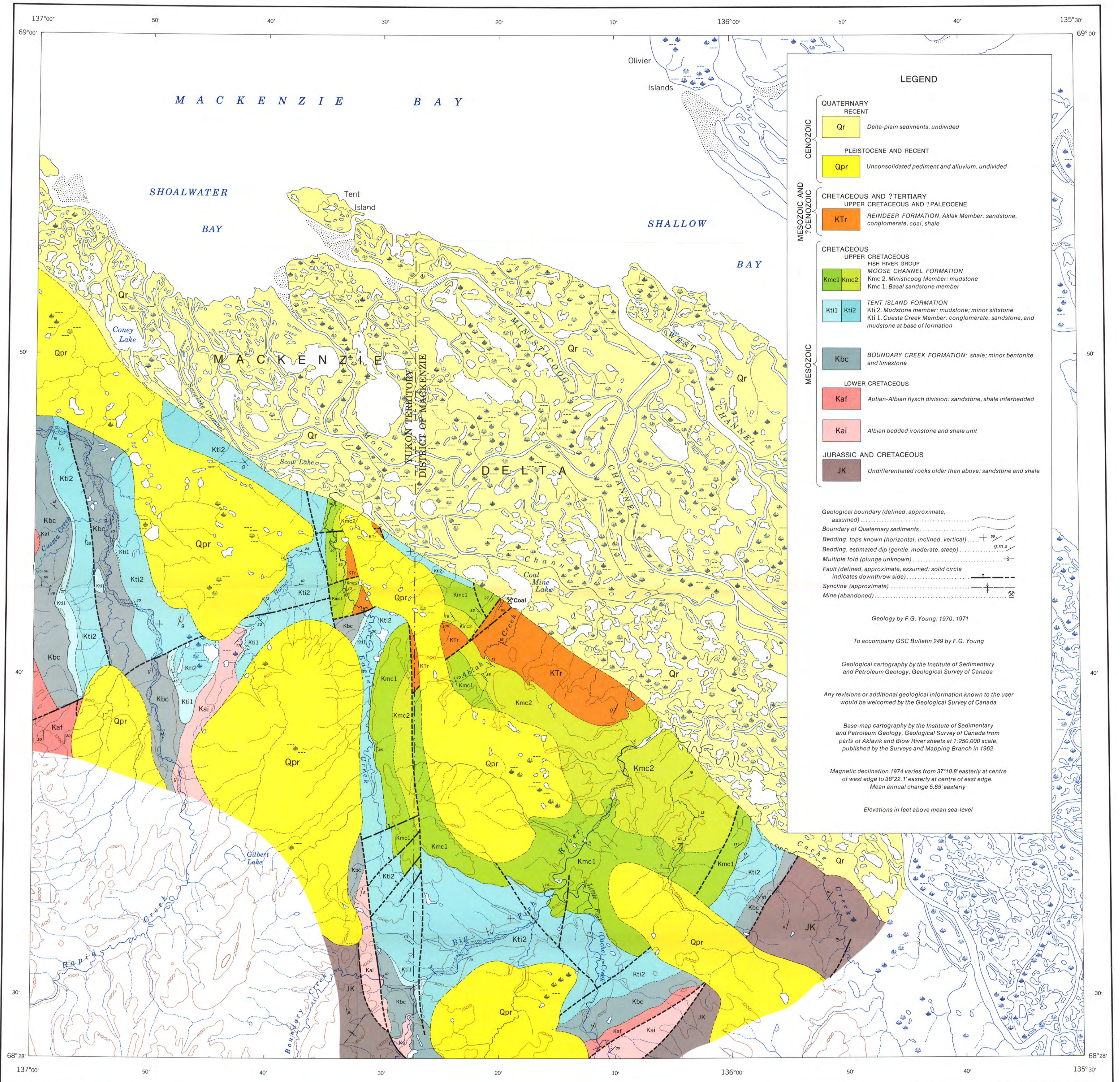
Figure 1. Geological map of northeastern Yukon Coastal Plain
