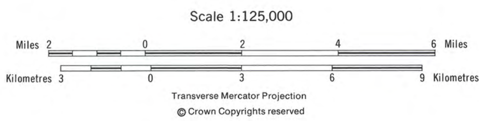
Figure 1. Geological map of northeastern Yukon Coastal Plain
