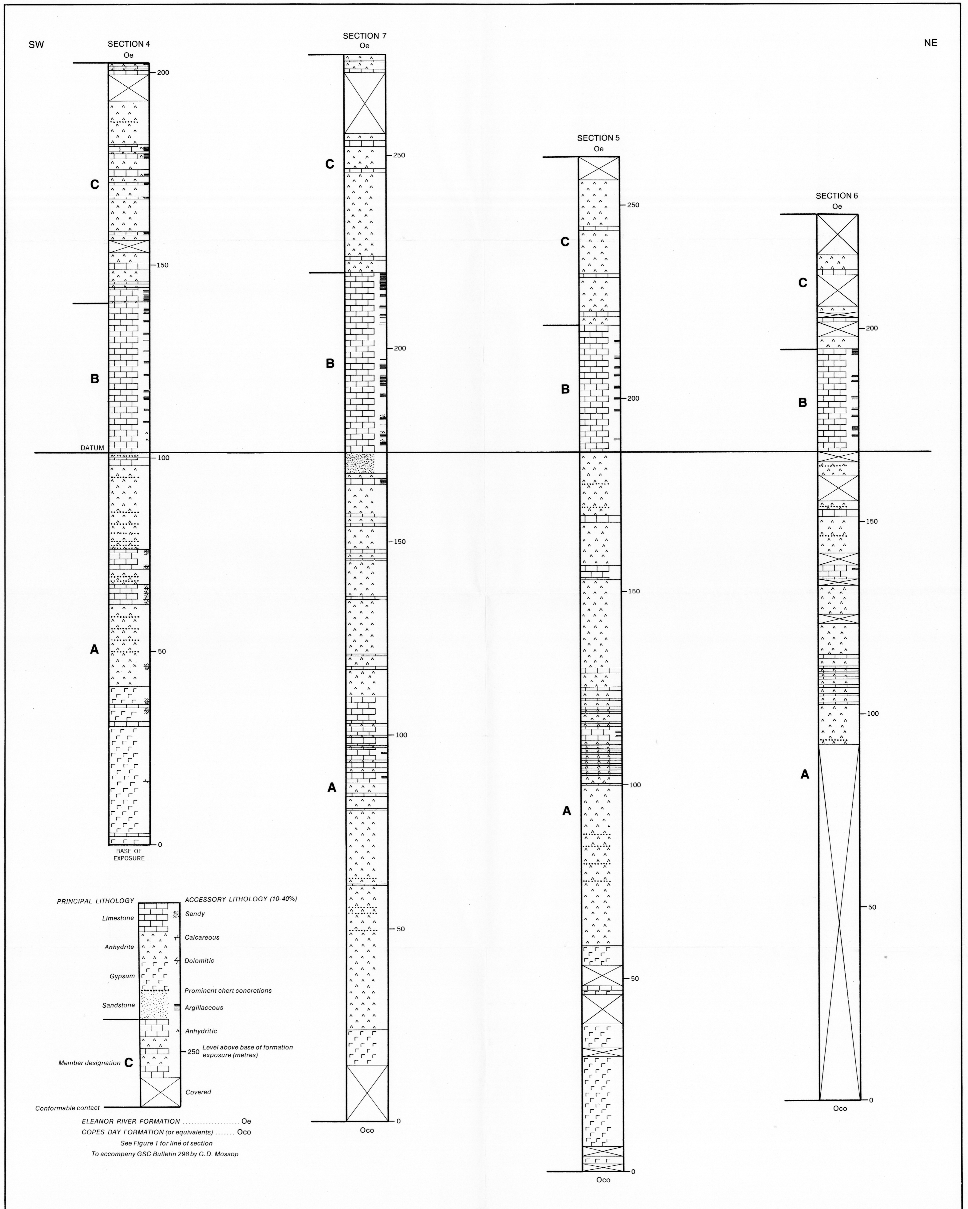
Figure 5. Lithologic columns for measured sections of the Baumann Fiord Formation in the Arctic Platform region, Sverdrup Pass to Bache Peninsula, Ellesmere Island
