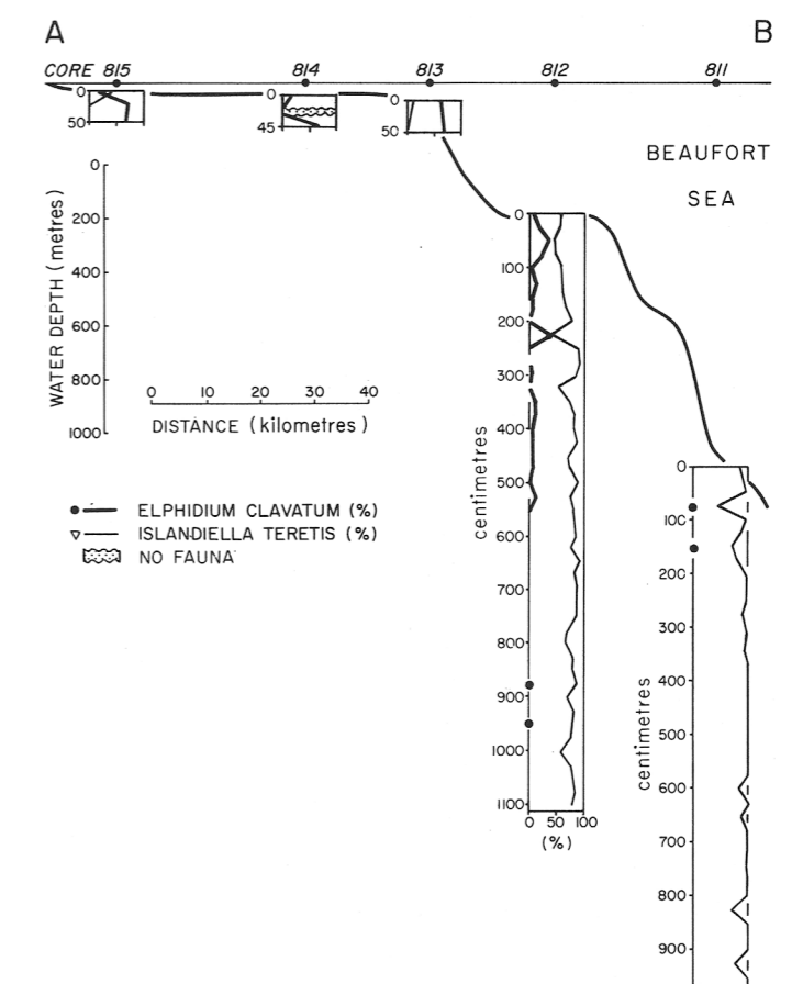
c. Relative percentages of Elphidium clavatum and Islandiella teretis to total foraminifera in sediment cores.
