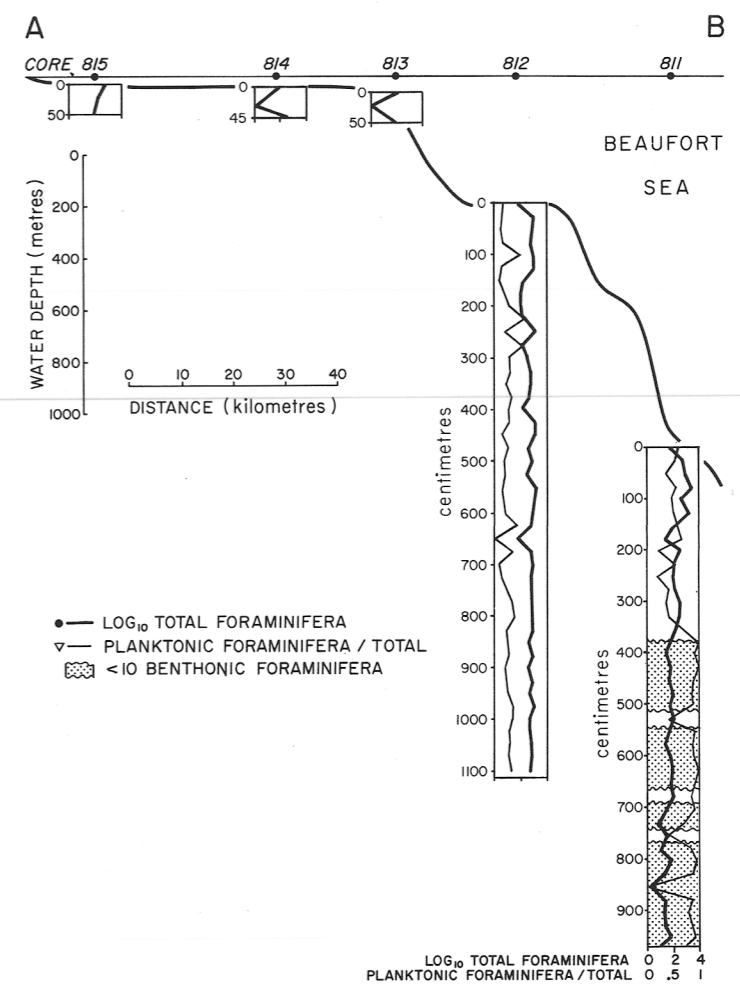
b. Total foraminifera and the ratios of planktonic foraminifera over total foraminifera in sediment cores.
