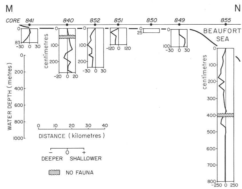
Figure 37. Traverse MN
