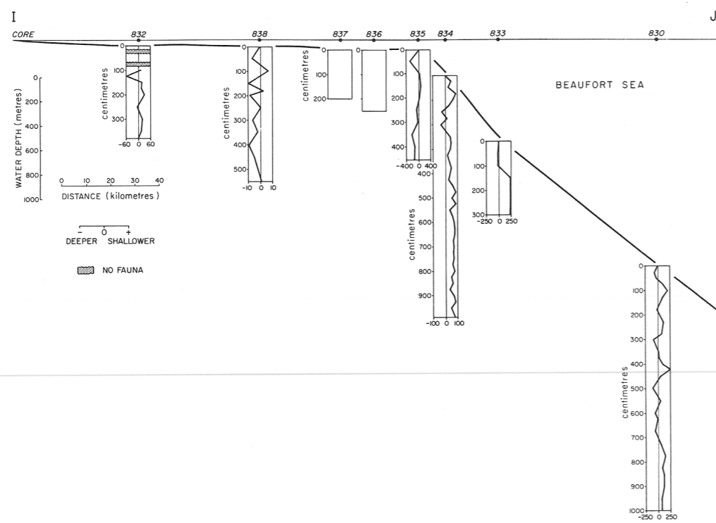
Figure 35. Traverse IJ
