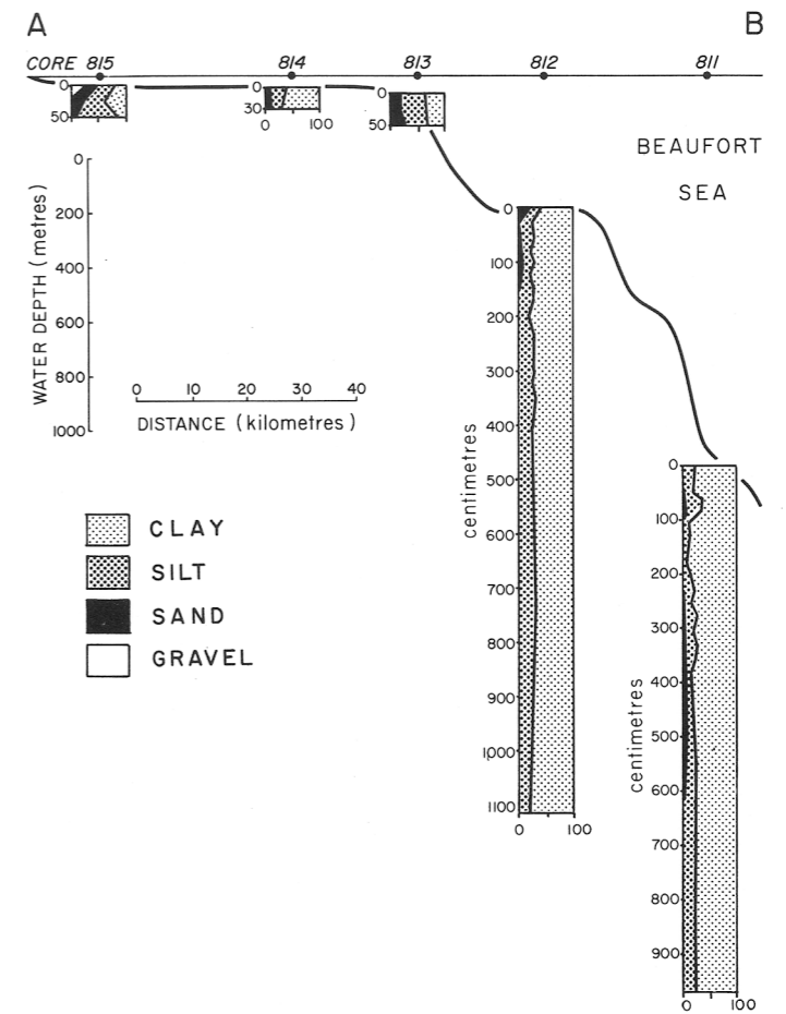
a. Relative percentages of clay, silt, sand, and gravel in sediment cores.
