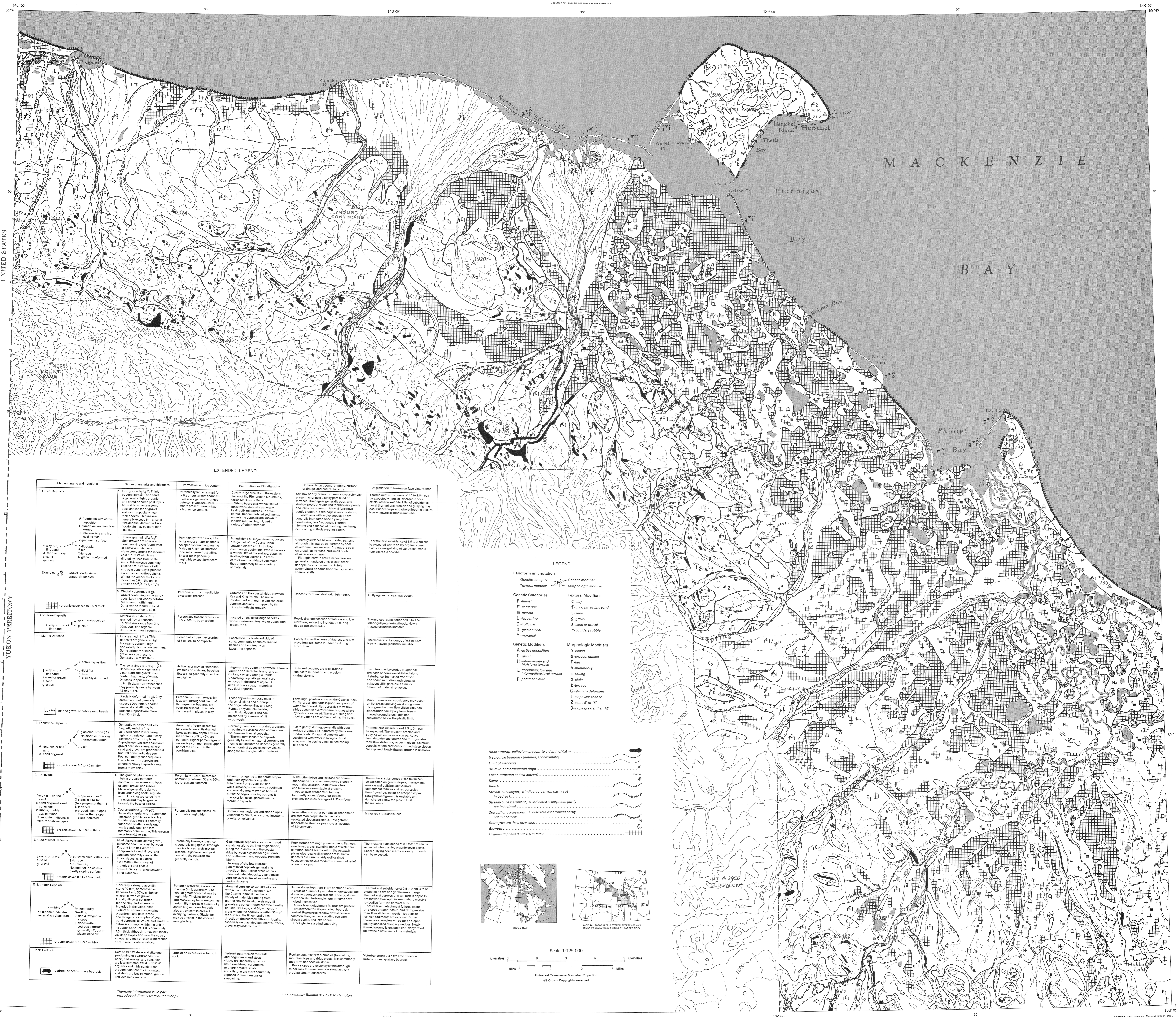
Figure 37. Surficial deposits and landforms, western Yukon Coastal Plain
