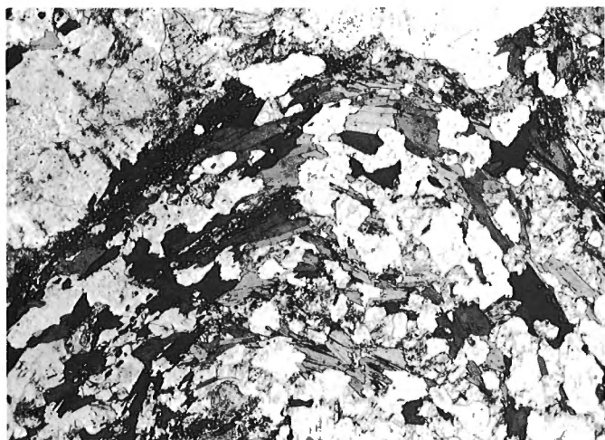
Figure 6. Microfold in pelitic gneiss. Note that gneissosity and biotite foliation are deformed in the fold hinge. Width of photo area is 5 mm. (GSC 202949-1)
