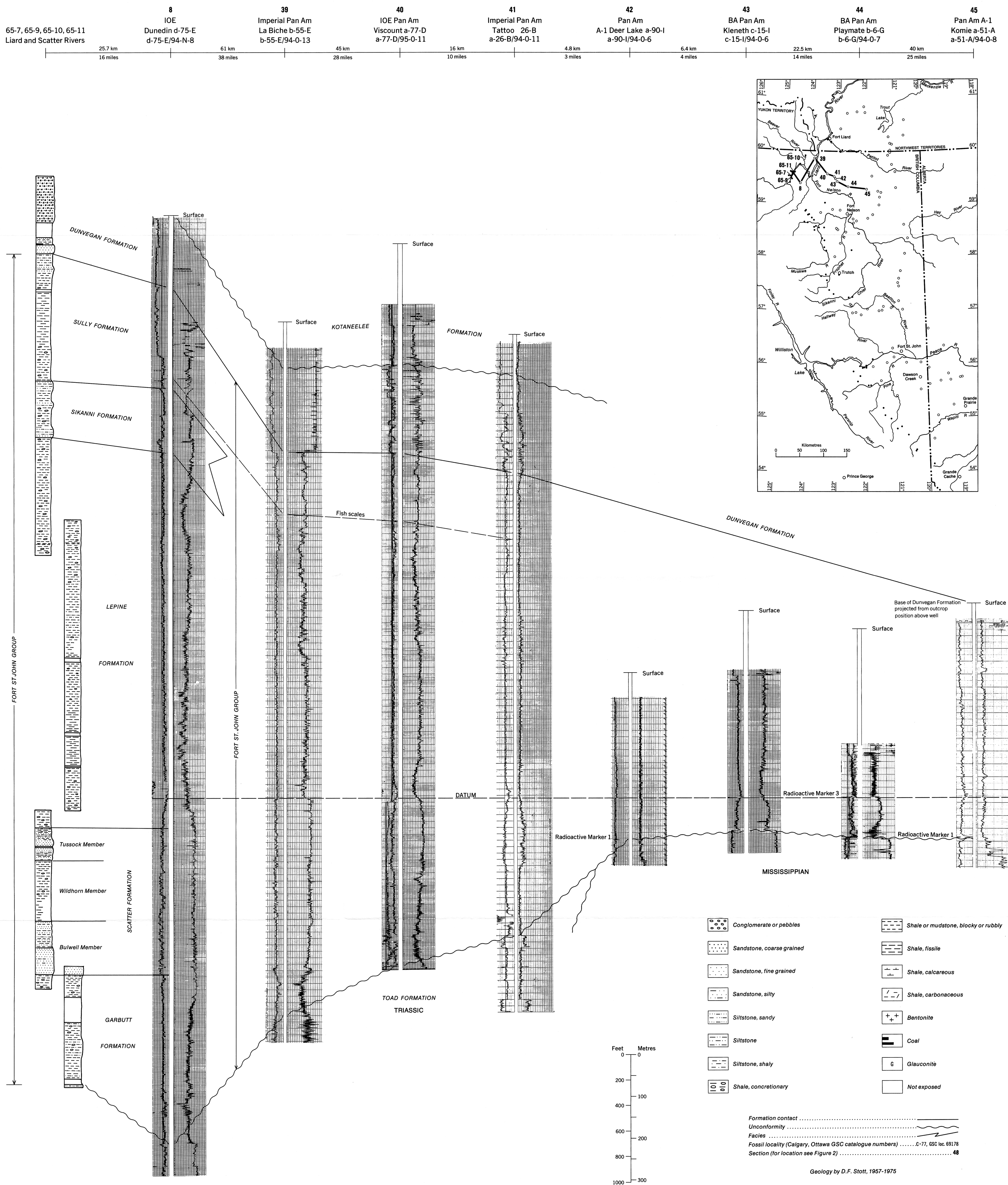
Figure 18. Columnar sections of Fort St. John Group and Dunvegan Formation between Scatter River and Pan Am A-1 Komie a-51-A well, northeastern British Columbia.
