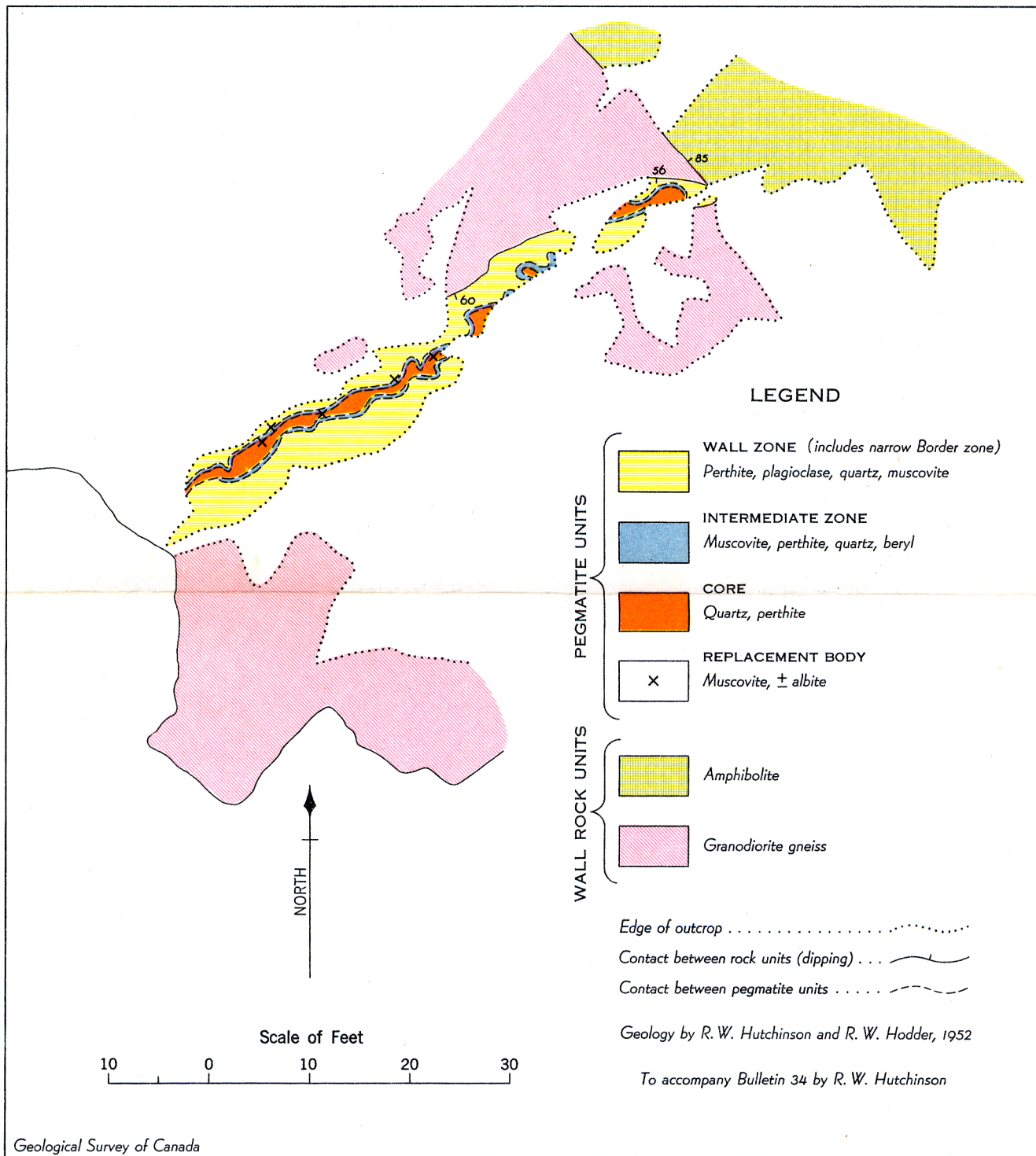
Figure 8. Dyke No. 97, Ross Lake area, Northwest Territories
