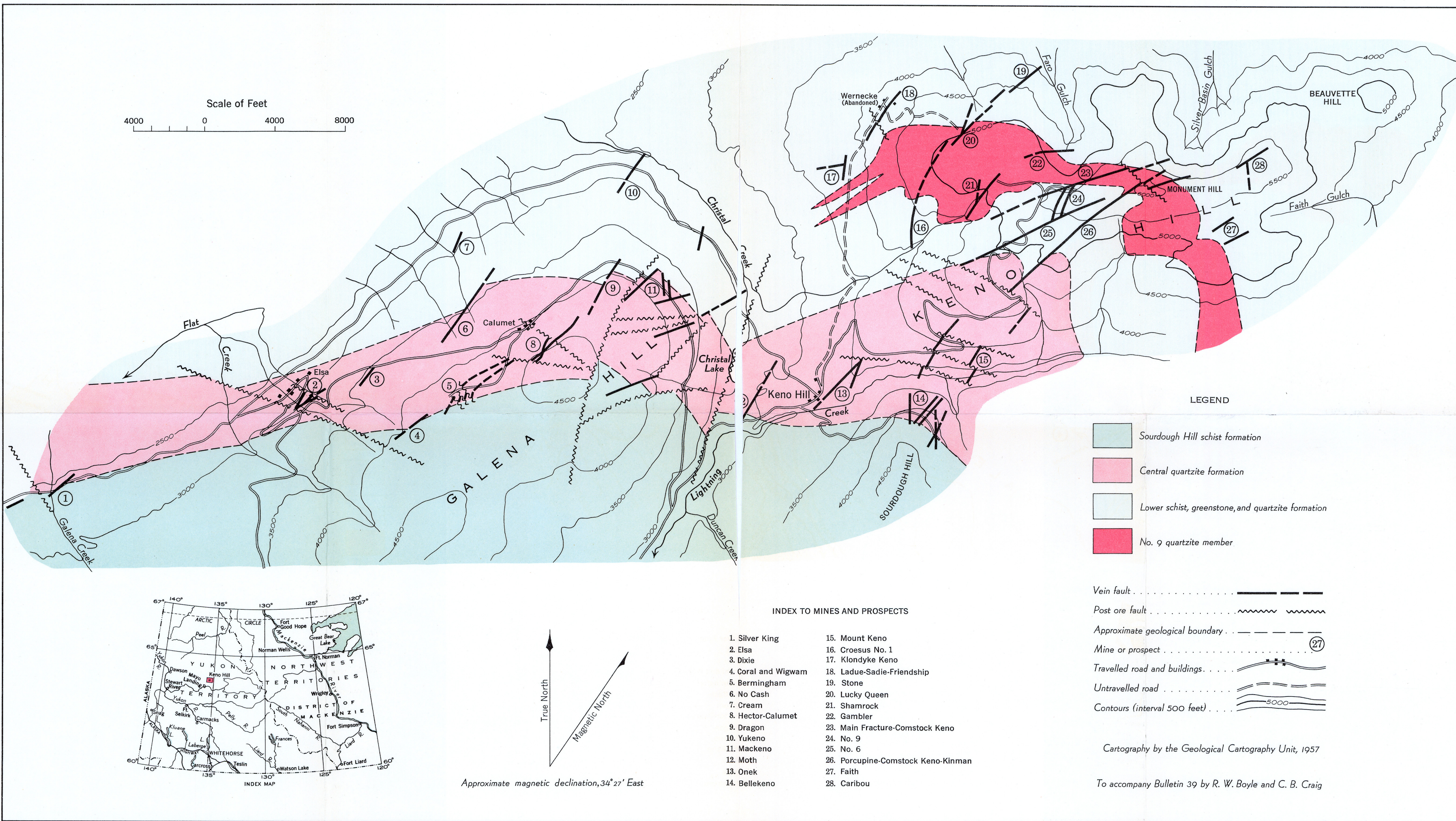
Figure 2. Map showing main geological features and principal mines and prospects, Keno Hill - Galena Hill area, Yukon Territory
