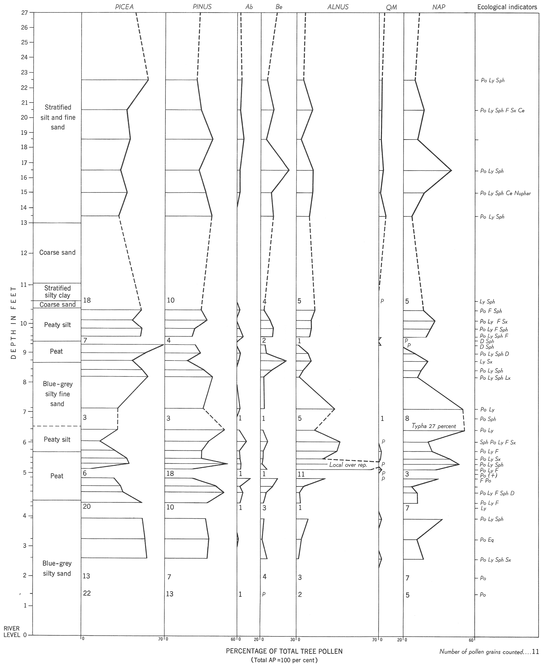
Figure 4. Pollen diagram of Les Vieilles Forges section To accompany Bulletin 46, by J. Terasmae
