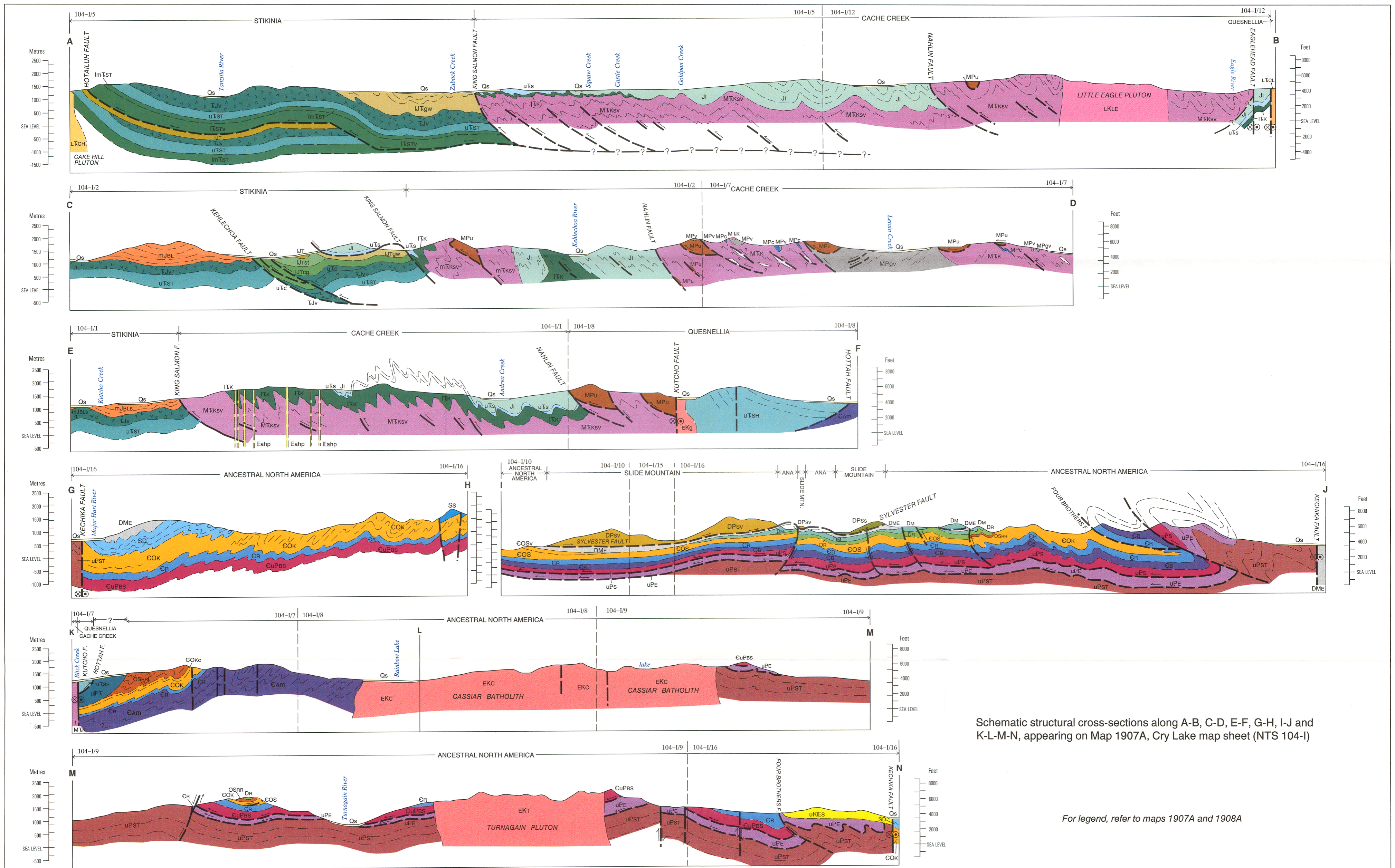
Figure 64. Schematic, structural cross-sections to accompany maps 1907A and 1908A
