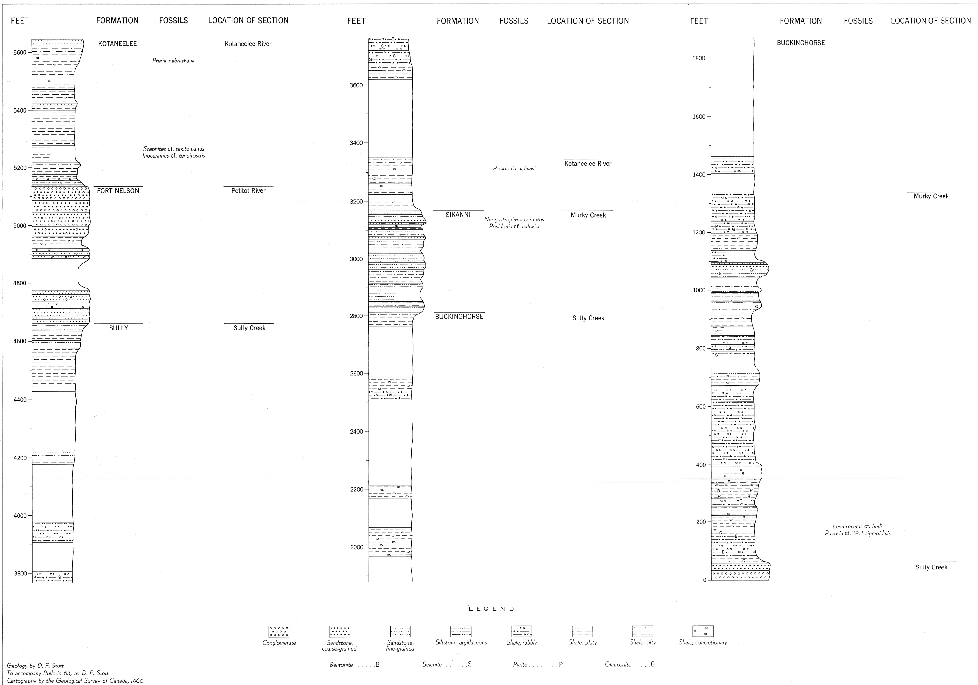
Figure 3. Composite columnar sections of Cretaceous formations in vicinity of Fort Liard, Northwest Territories
