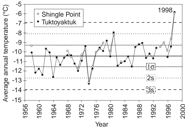
Figure 2. Average annual air temperatures for Tuktoyaktuk, Northwest Territories, and Shingle Point, Yukon Territory. Also depicted is the mean (-10.4°C) and the first, second, and third standard deviations for Tuktoyaktuk. Data from Atmospheric Environment Services, Environment Canada.
