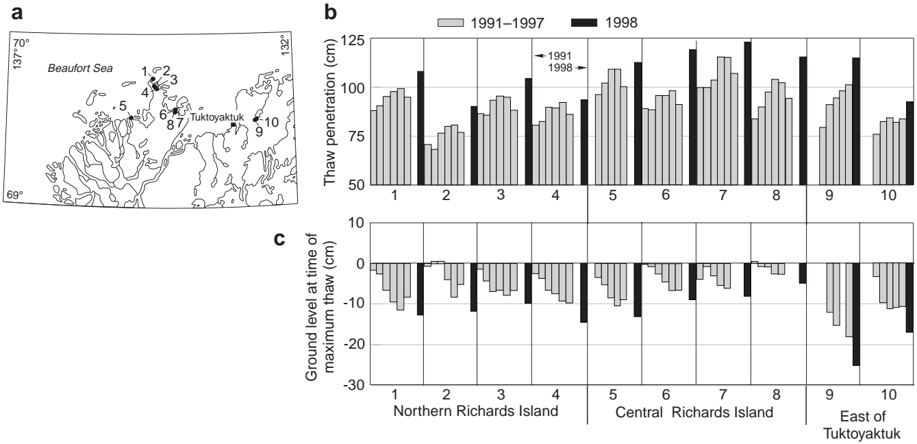
Figure 4. Thaw-depth monitoring in the Richards Island and Tuktoyaktuk areas: a) locations of thaw tubes; b) 1998 thaw penetration compared to previous years since 1991; c) ground levels at the time of maximum thaw, relative to the first year of monitoring. Data from 1997 is missing at most sites because of the rapid progression of thaw in 1998.
