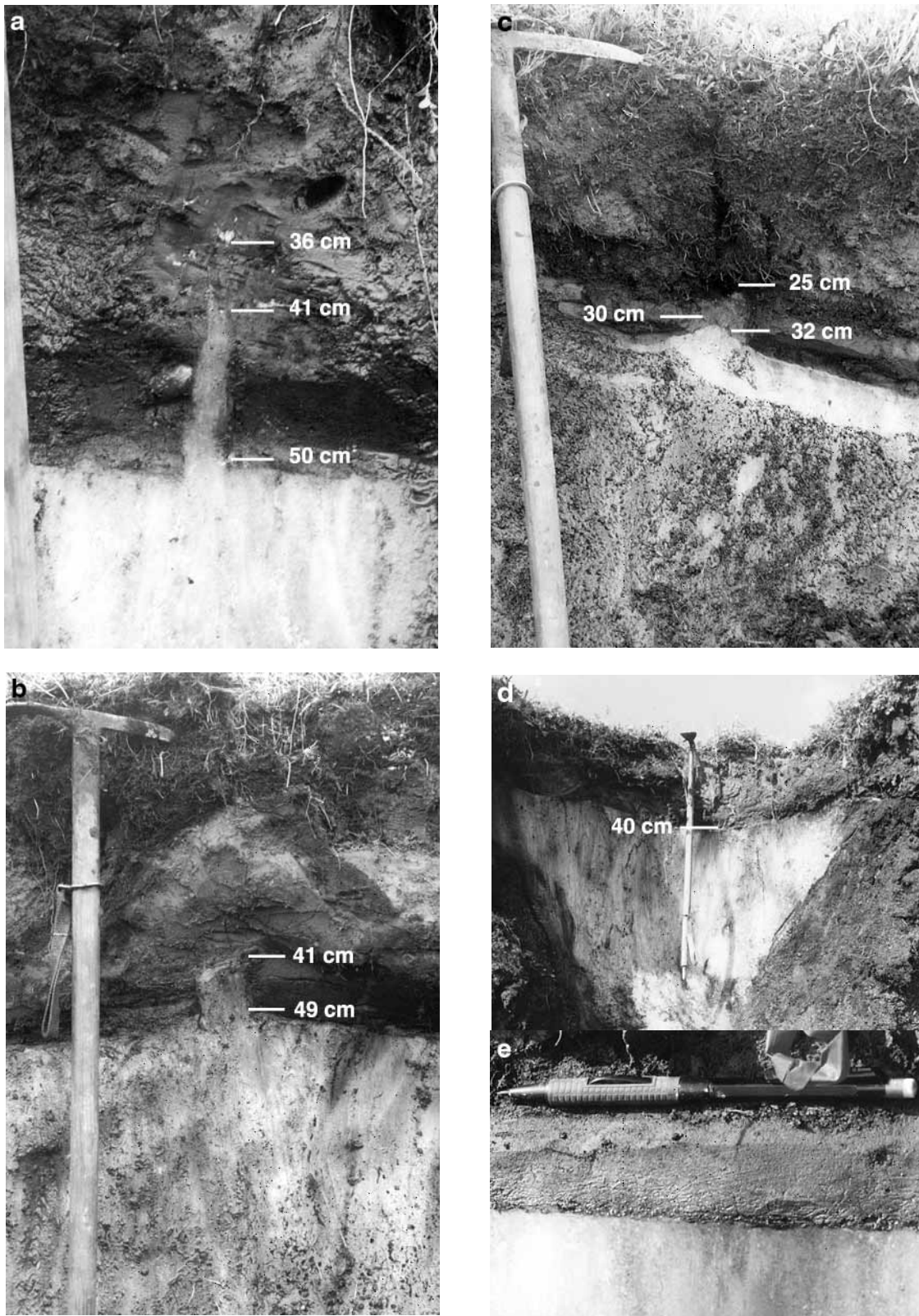
Figure 6. Photographs of the tops of ice wedges observed on Northern Richards Island and the Yukon coast in July 1999. a) Primary and secondary ice wedges with recent (tertiary) cracking at on northern Richards Island with depths to tops of wedges. b) Ice wedge at North Head with primary and secondary growth. The top of the secondary wedge has been abruptly truncated by thawing. c) Ice wedge at North Head with primary wedge at a depth of 32 cm and a residual secondary wedge at 30 cm. Ice overlying the residual wedge is pool ice, indicating refreezing of water above the wedge. d) Ice wedge with overlying trough along the Yukon coast. e) Modern roots in contact with the top of the ice wedge.
