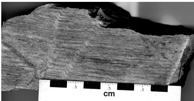
Figure 5. Sawn slab of quartz-feldspar augen schist (felsic metatuff; sample 99RAS-31-1) from the Dorsey assemblage. Grey specks and white dots are quartz and feldspar phenocrysts respectively.
