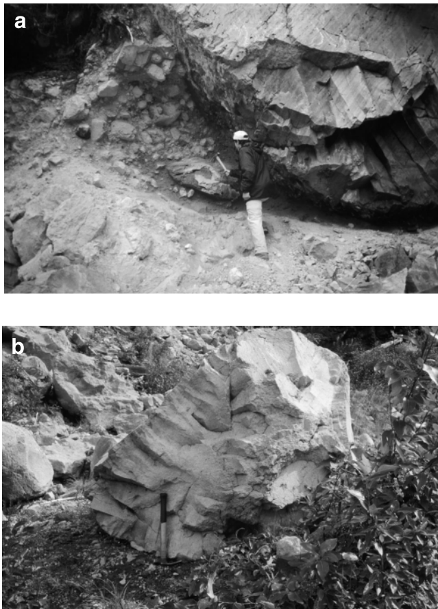
Figure 6. Field photographs of the hot avalanche deposit of the Plinth Formation. Specific details shown include a) a very large (>10 m) flow-banded block of dacite surrounded by poorly indurated, unsorted matrix; b) fine- and coarse-scale, radially oriented, prismatic jointing on a large block; and c) detail of the fine-scale jointing normal to the surface of the clast depicted in b). The hammer in b) is 45 cm long.
