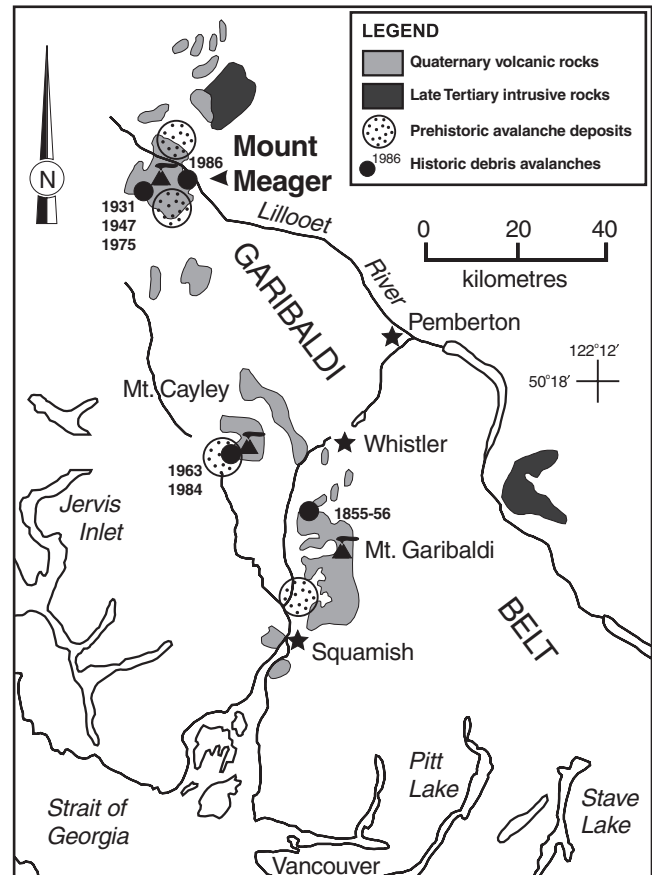
Figure 1. Location of the Mount Meager volcanic complex with respect to other Quaternary volcanic edifices in the Garibaldi Volcanic Belt of southwestern British Columbia (after Hickson, 1994). Also shown are the locations of large accumulations of prehistoric avalanche deposits and historical rock avalanches associated with the same volcanic terranes (after Evans, 1992).
