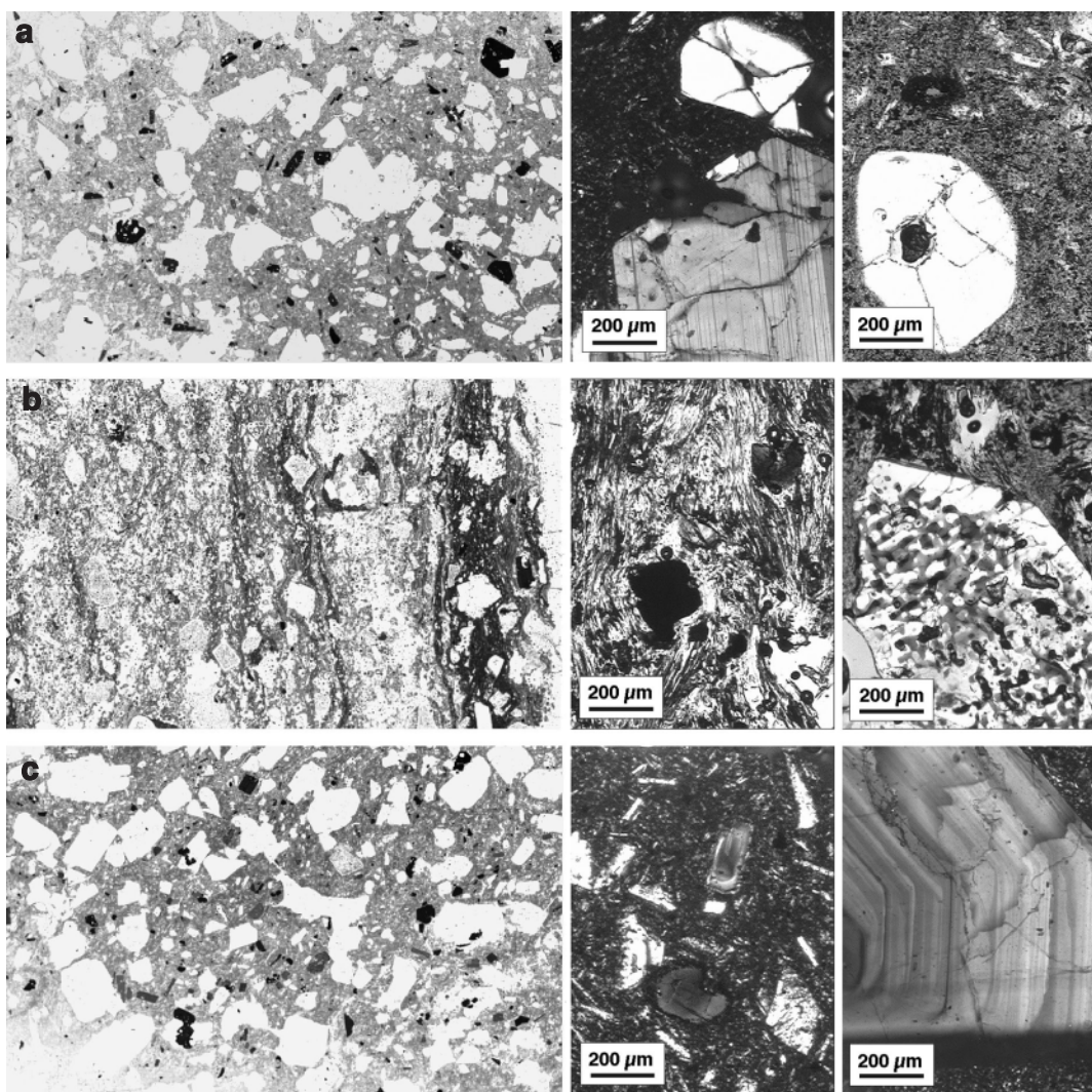
Figure 7. Digitally scanned images of thin sections under plane-polarized (ppl) and crosspolarized (cpl) light (sections are 4 cm by 2.5 cm). Images are of thin sections from a) cold Plinth avalanche deposit (ppl), showing rounded quartz and euhedral plagioclase phenocrysts (cpl) and a quartz phenocryst with amphibole inclusion in devitrified matrix (ppl); b) Hot Pebble Creek block-and-ash flow (ppl), showing flattened vesicles in a welded block and a sieve-textured (resorbed) coarse, euhedral plagioclase grain (ppl); and c) hot Plinth block-and-ash flow (ppl), showing microphenocryst-rich matrix (cpl) and a distinctly zoned and unresorbed plagioclase phenocryst (cpl).
