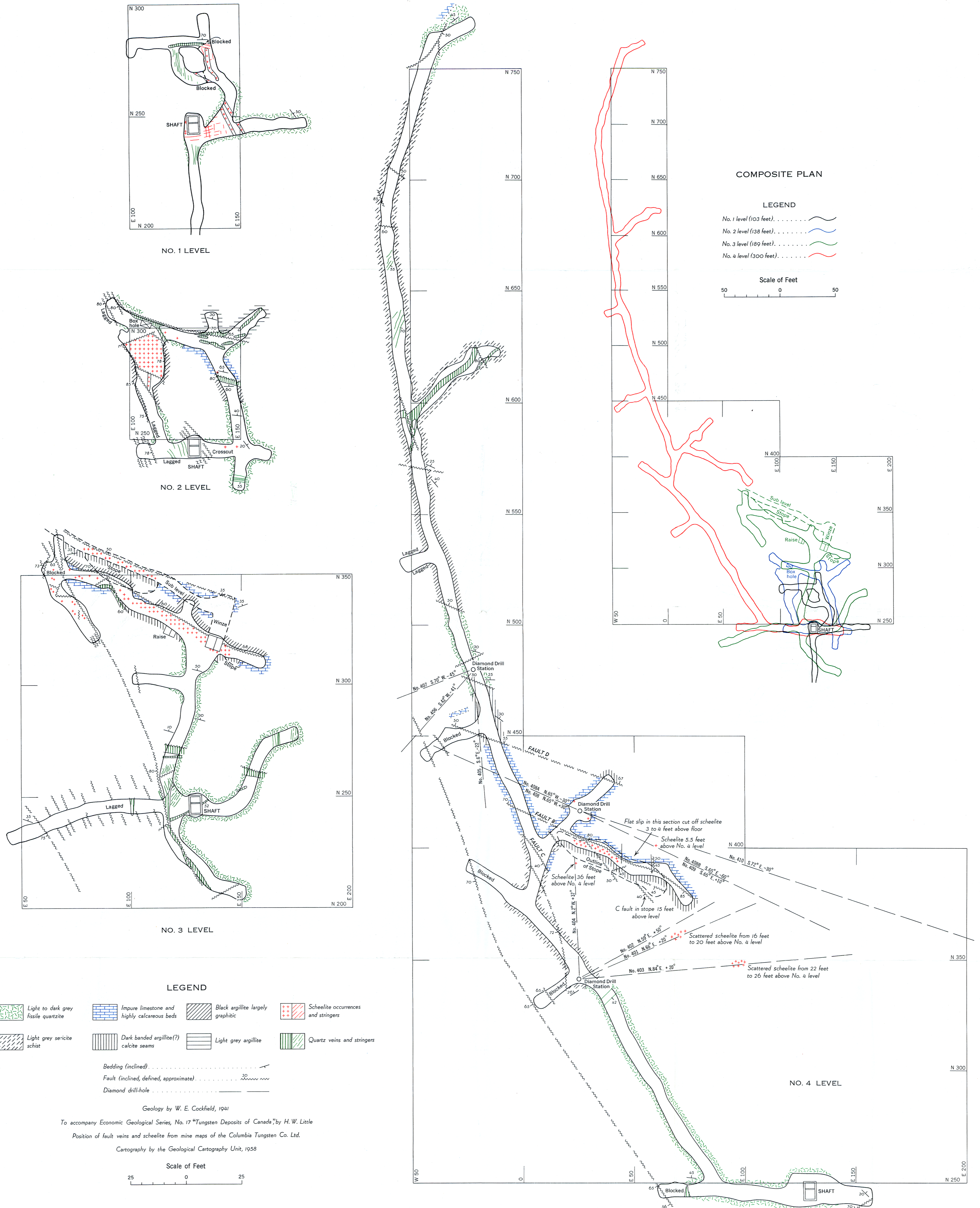
Figure 10. Underground workings with geology and tungsten occurrences, and composite plan of Hardscrabble Creek deposit, Cariboo Area, British Columbia
