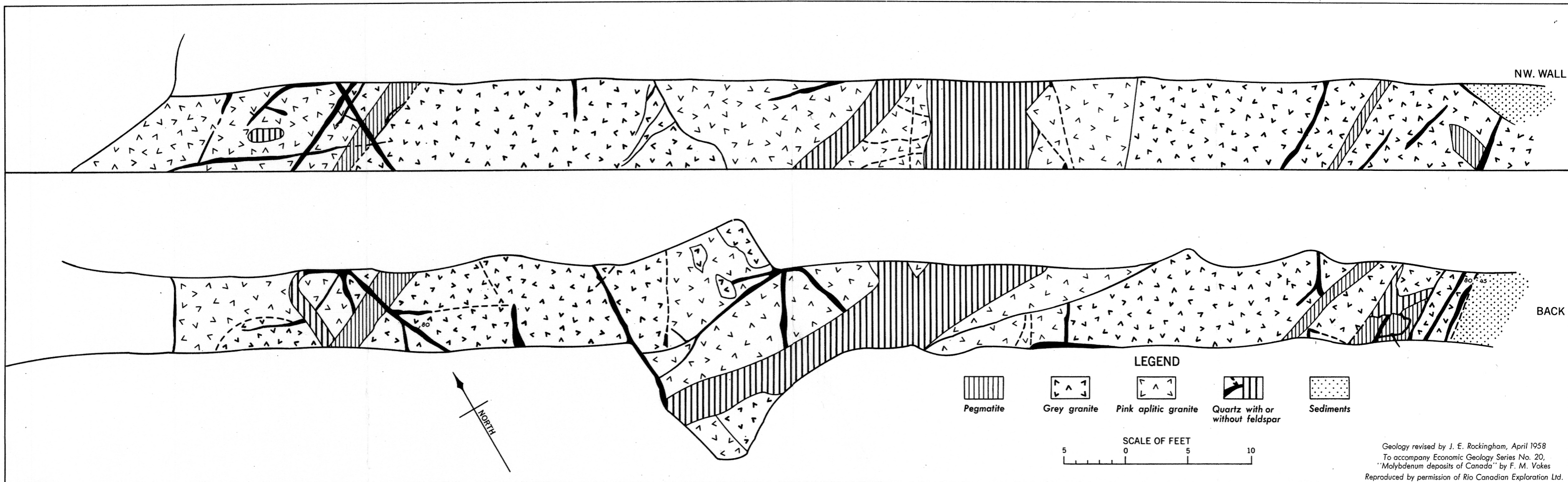
Figure 3. Geology of northwest wall and back of adit, Pidgeon Molybdenum property, Ontario
