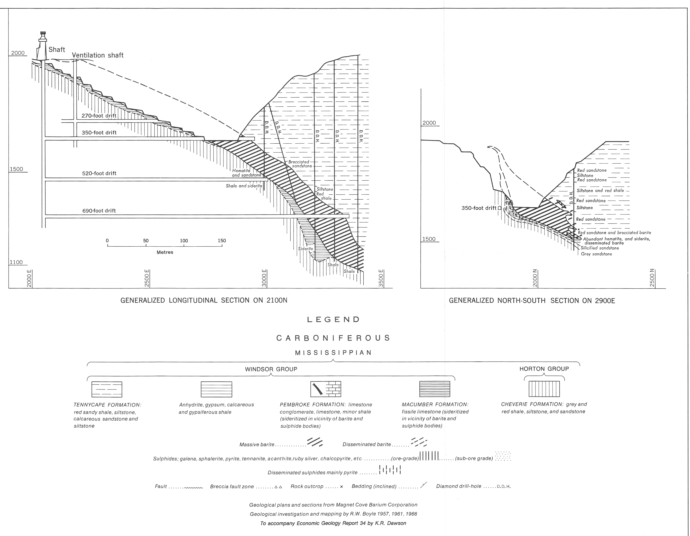
Figure 20. Surface plan and sections of the Walton, Nova Scotia, barium-silver-lead-zinc mine, after Boyle (1972).
