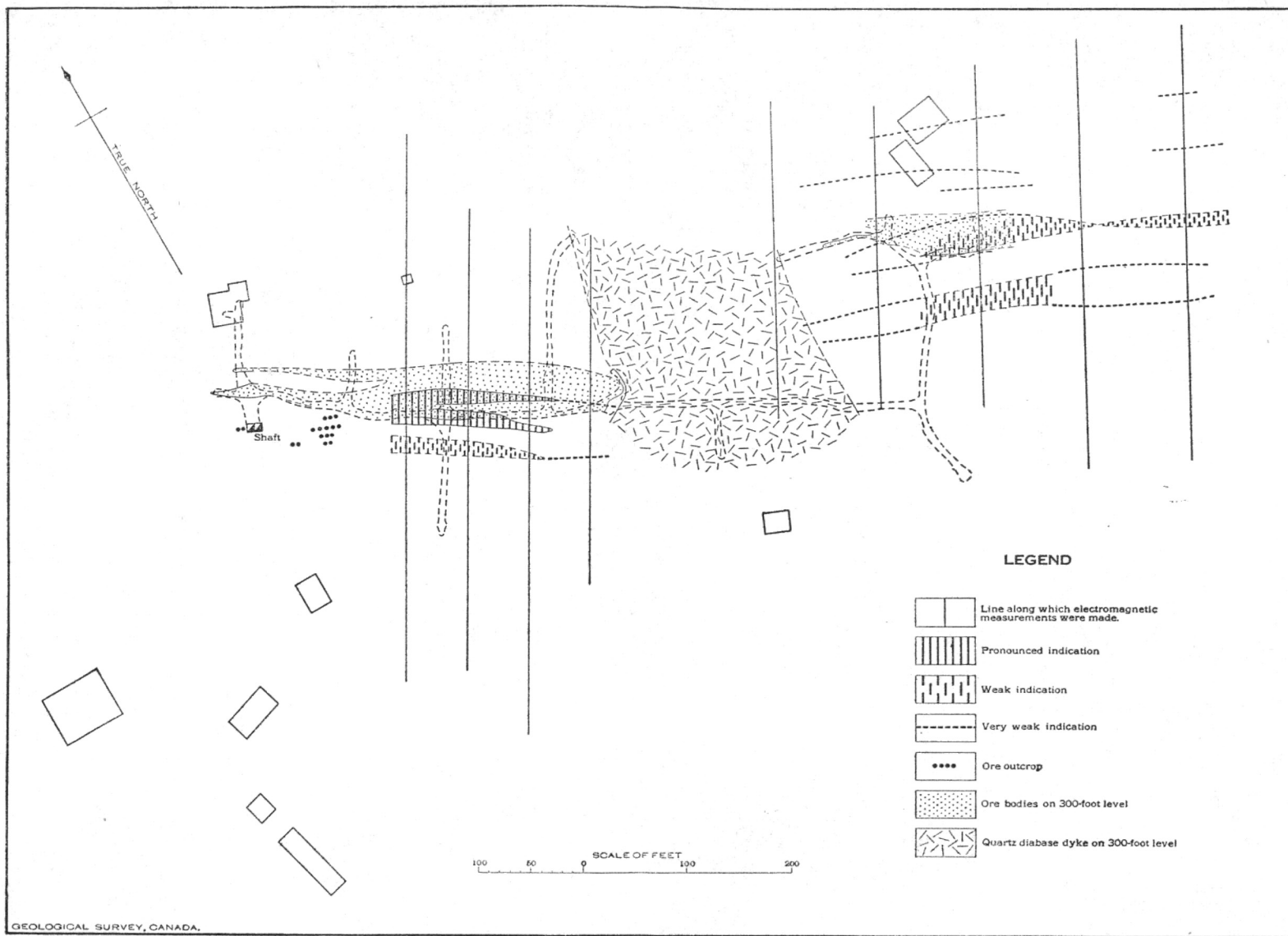
PLAN NO. 8 SURVEY OF ABANA MINE, DESMELOIZES TOWNSHIP, QUEBEC, BY SWEDISH AMERICAN PROSPECTING COMPANY OF CANADA, LIMITED. Results of survey by electromagnetic method.
