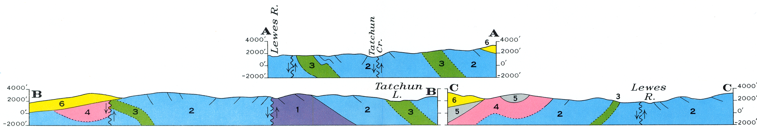
STRUCTURE SECTIONS ALONG LINES A-A, B-B, C-C
