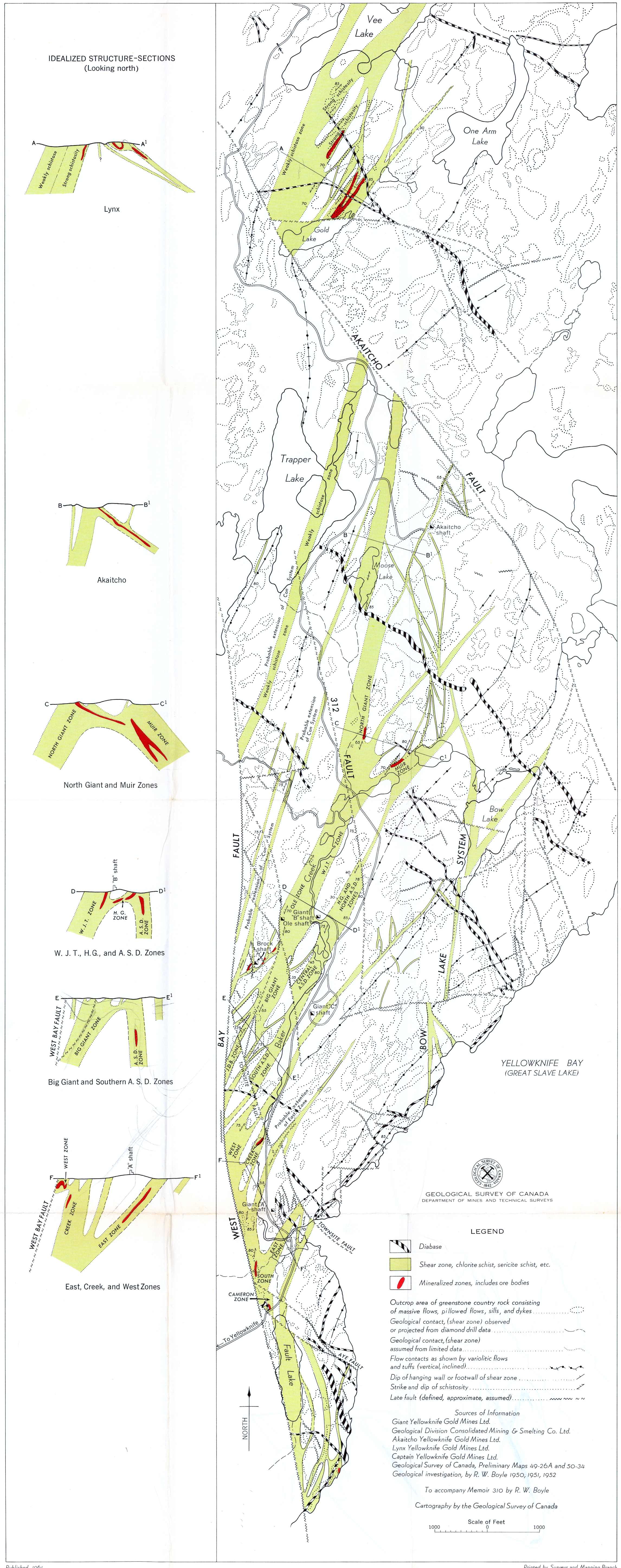
Figure 11, Surface plan and sections of the Giant system, Yellowknife area, District of Mackenzie, Northwest Territories
