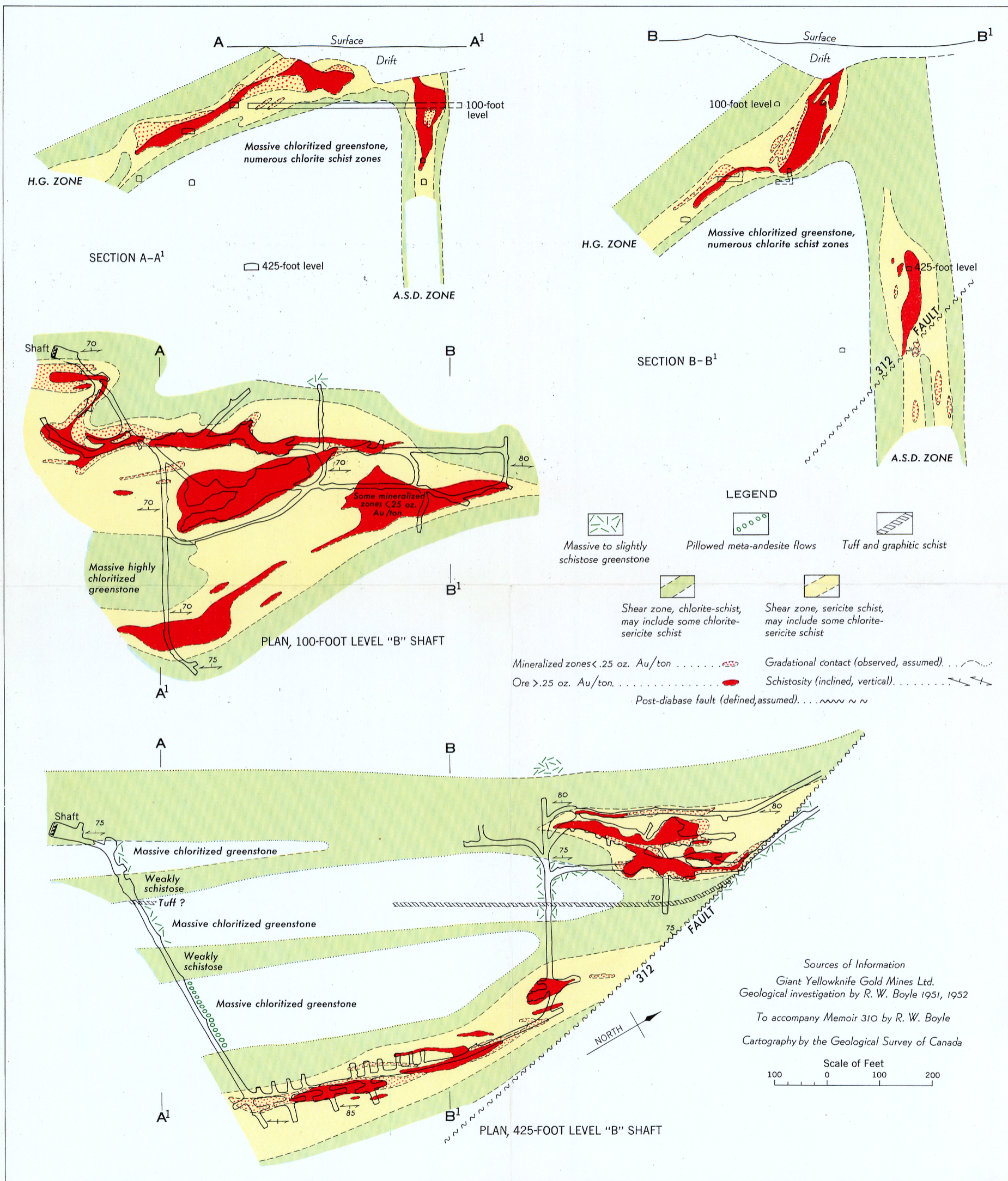
Figure 12, Geological plans and sections of the Giant mine, Yellowknife area, District of Mackenzie, Northwest Territories
