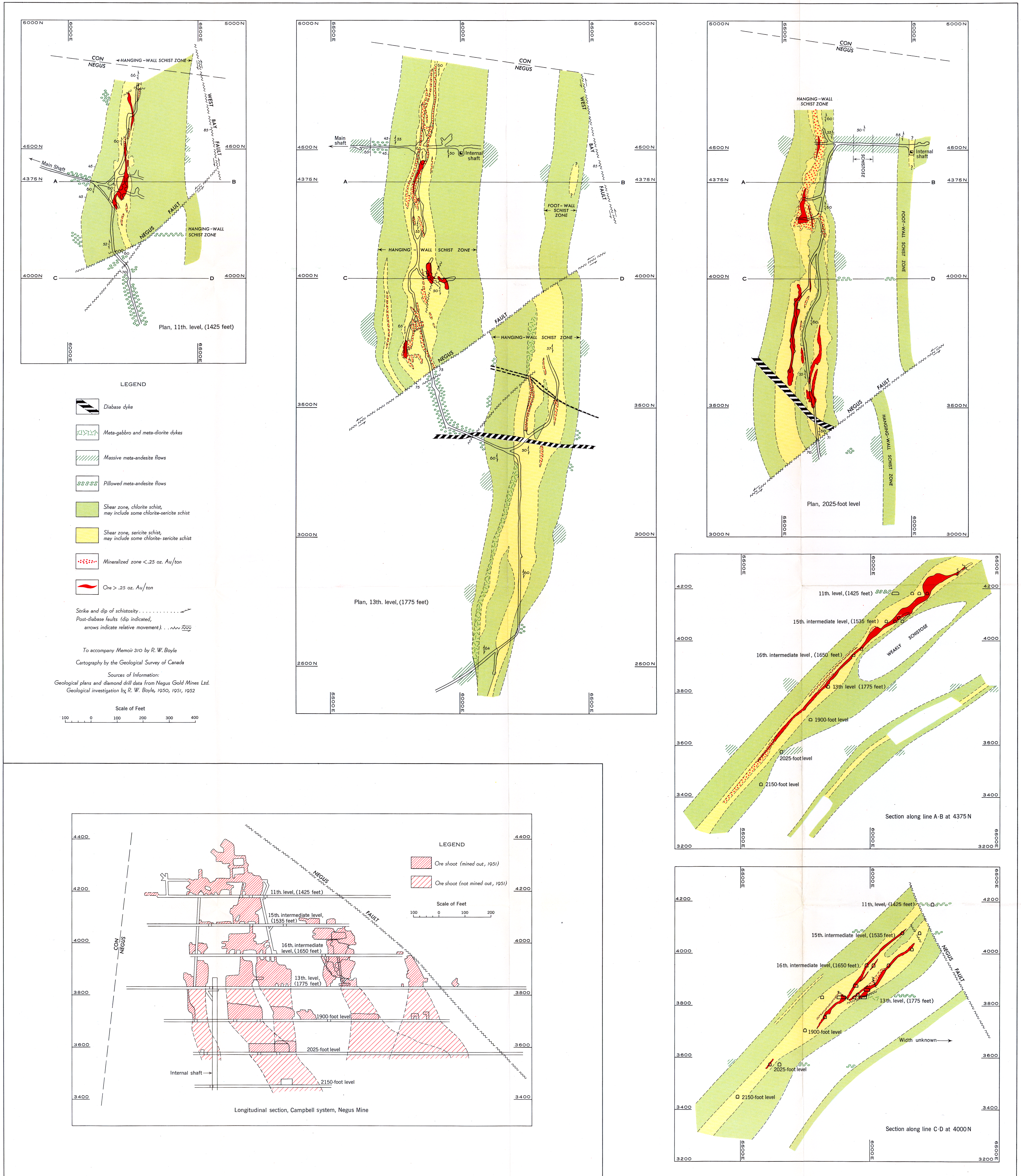
Figure 8. Geological plans and sections of the Negus Mine, Campbell system, Yellowknife area, District of Mackenzie, Northwest Territories
