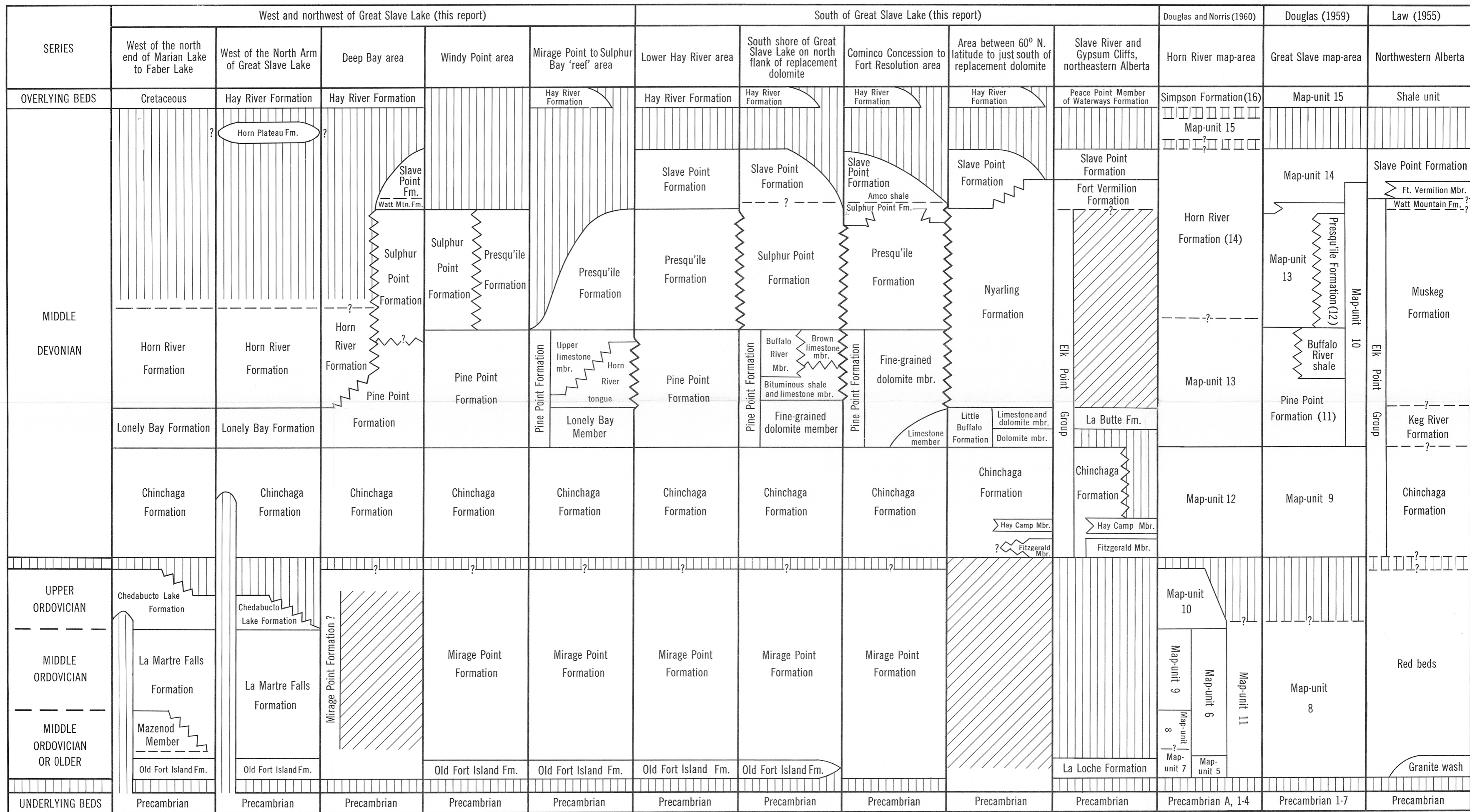
Figure 3. Nomenclature and relationship of Middle Devonian and Ordovician rock units of the Great Slave Lake region, District of Mackenzie
