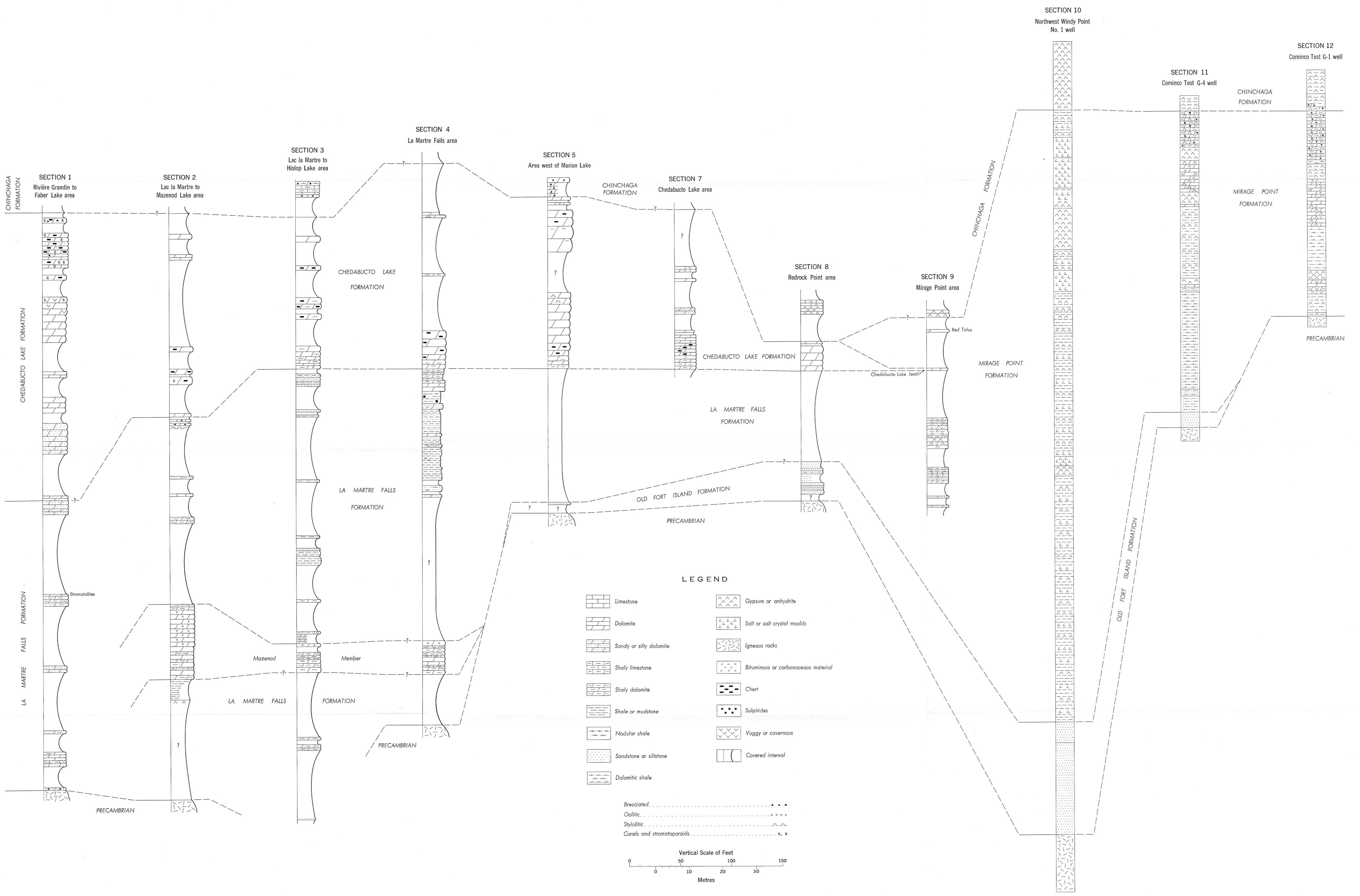
Figure 4. Composite outcrop and subsurface sections of the Old Fort Island Formation, La Martre Falls Formation and Mazenod Member, Chedabucto Lake Formation, and Mirage Point Formation, Great Slave Lake region, District of Mackenzie
