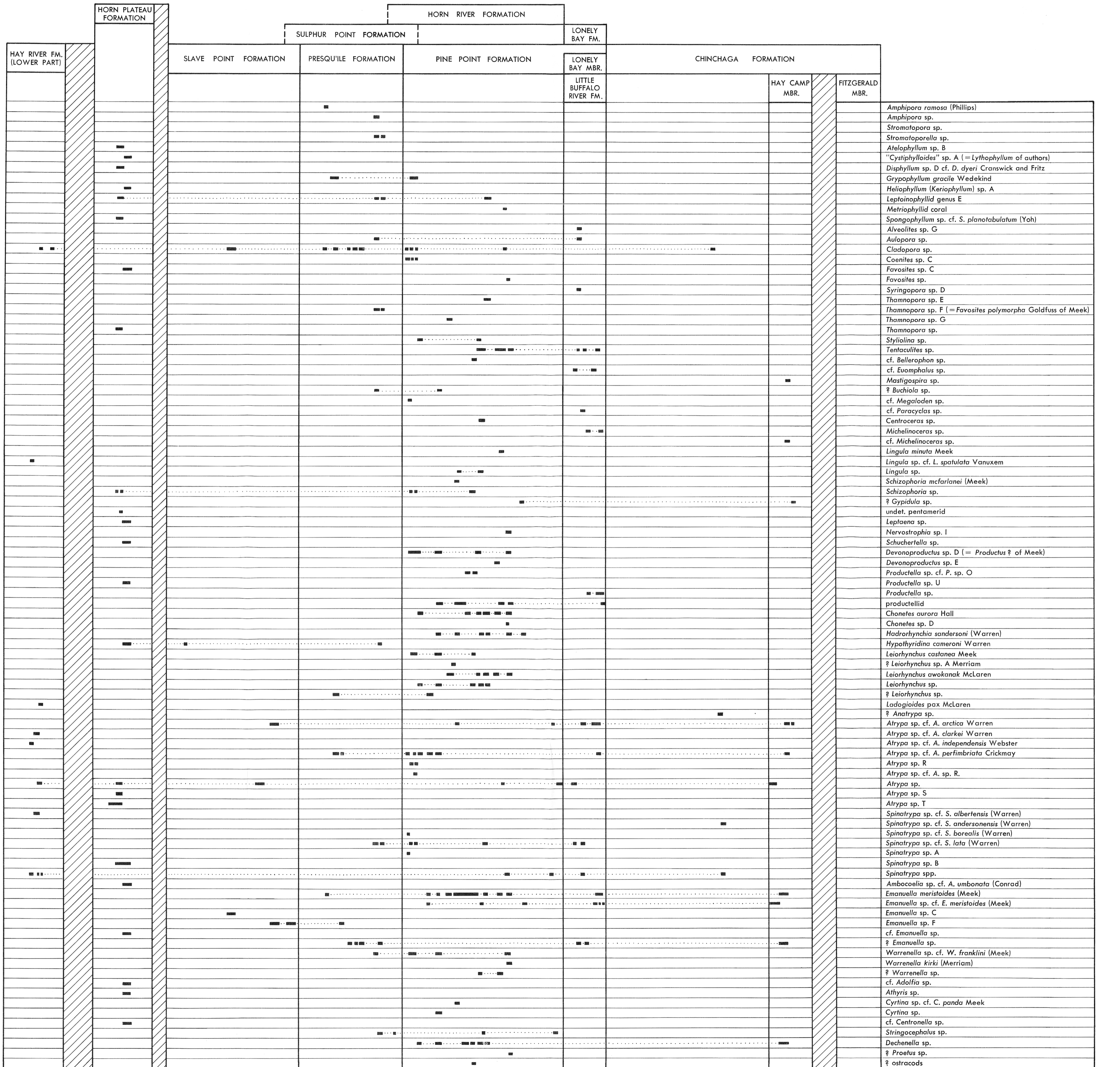
Figure 6. Distribution of Devonian fossils in the Great Slave Lake region, District of Mackenzie
