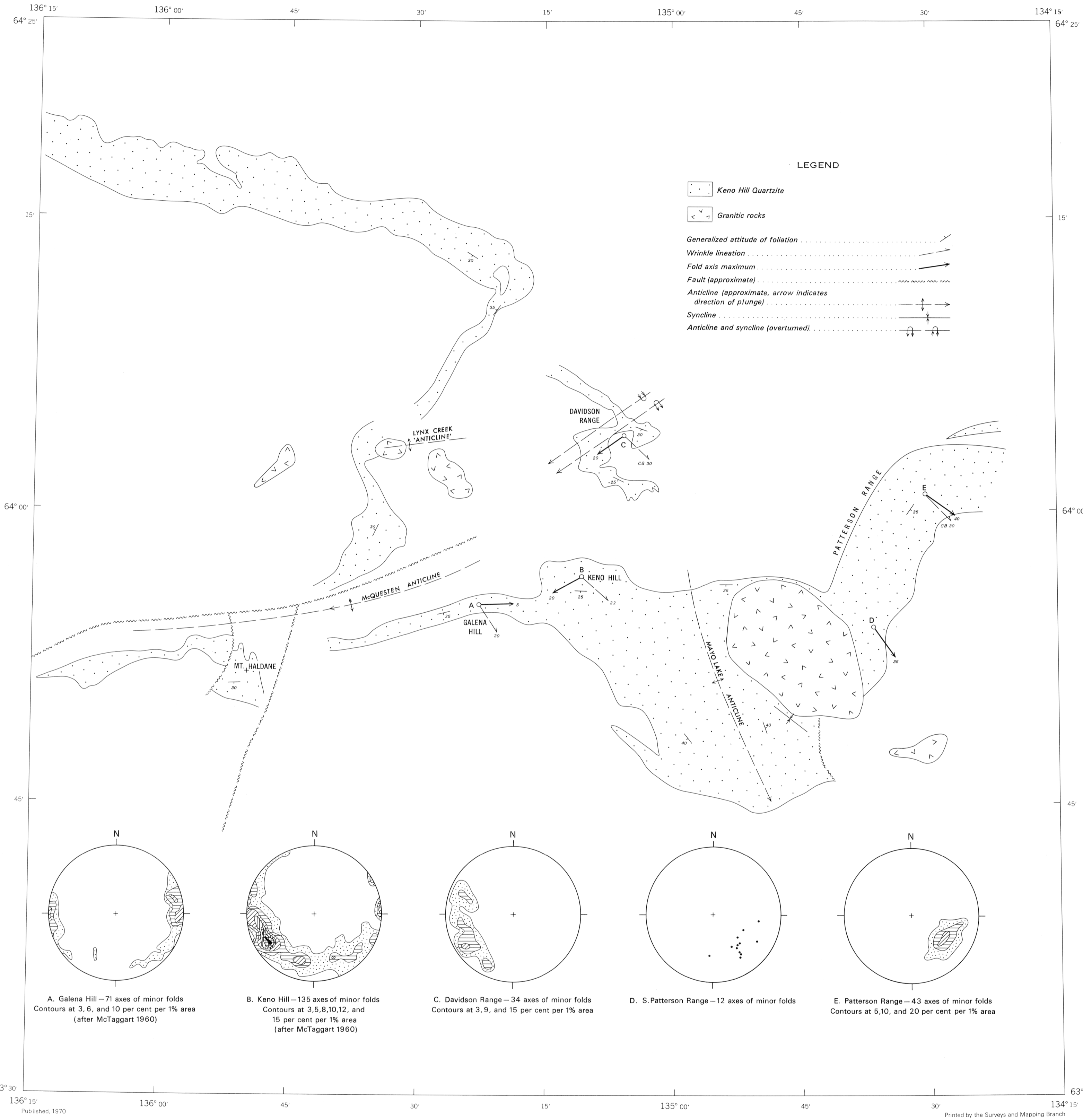
Figure 16. Structural elements, Keno and Galena Hills area, Yukon Territory.
