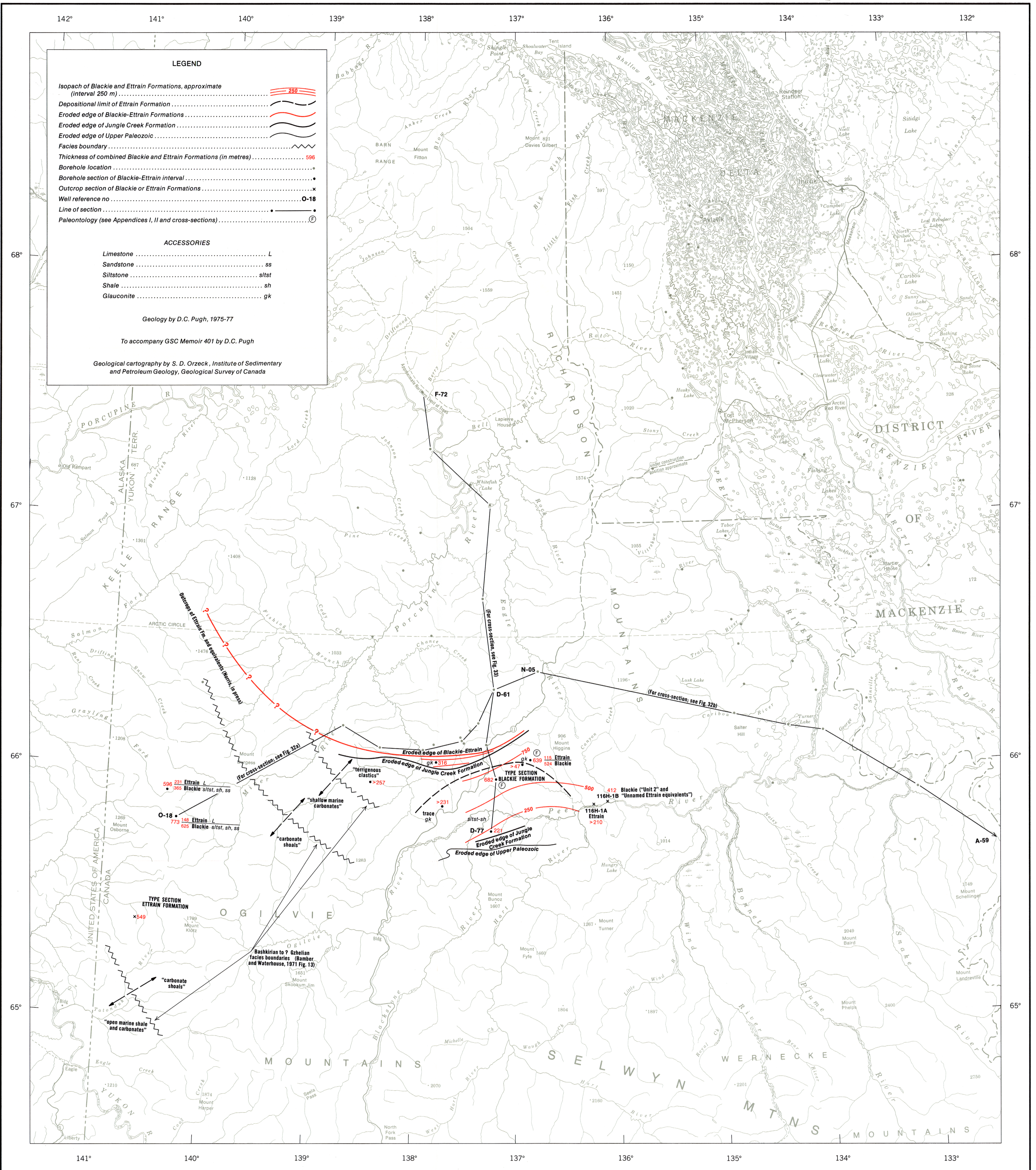
Figure 21. Isopach and lithofacies map of Blackie and Ettrain Formations
