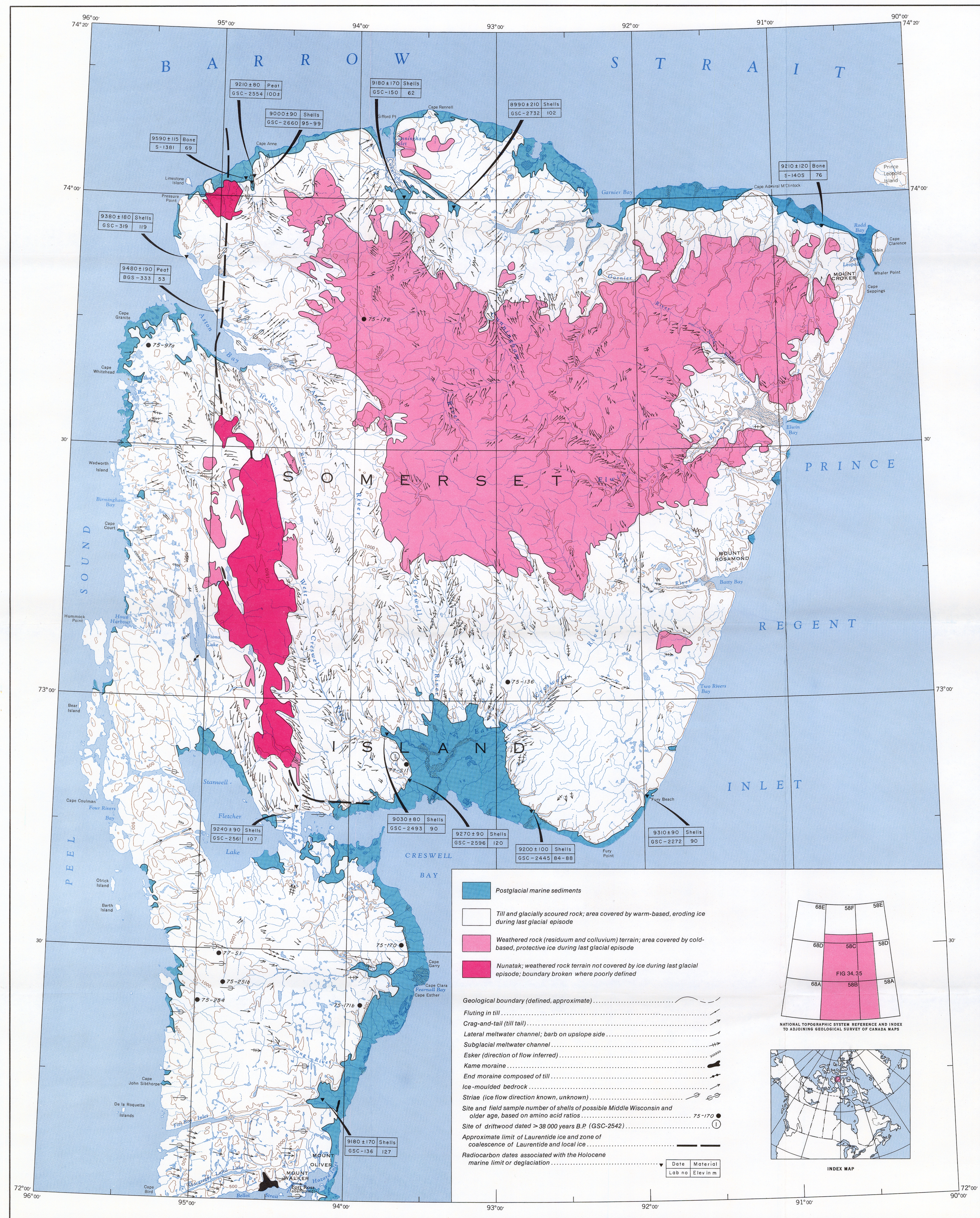
Figure 34. Simplified Quaternary geology map of Somerset Island
