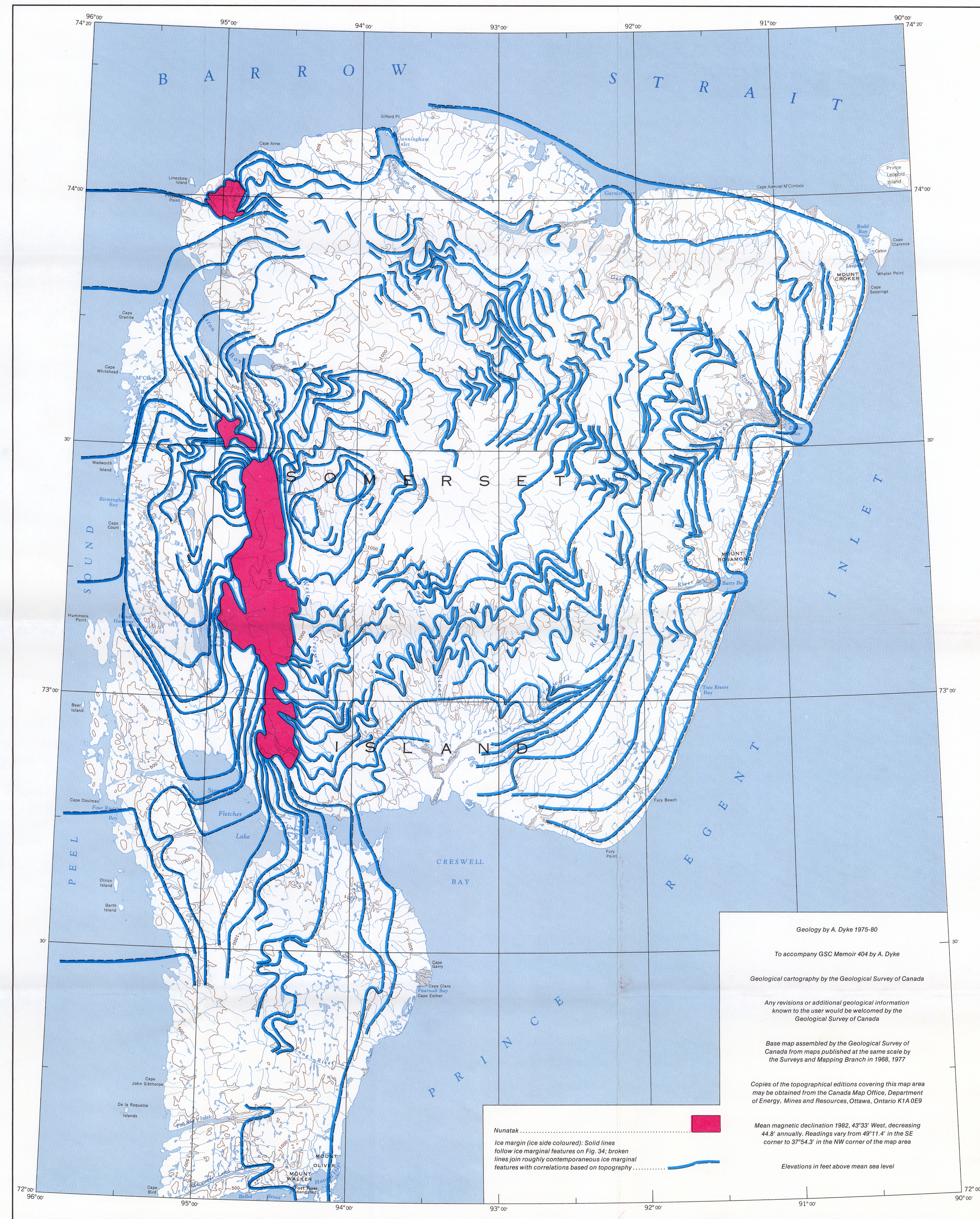
Figure 35. Pattern of ice marginal recession during the early Holocene on Somerset Island
