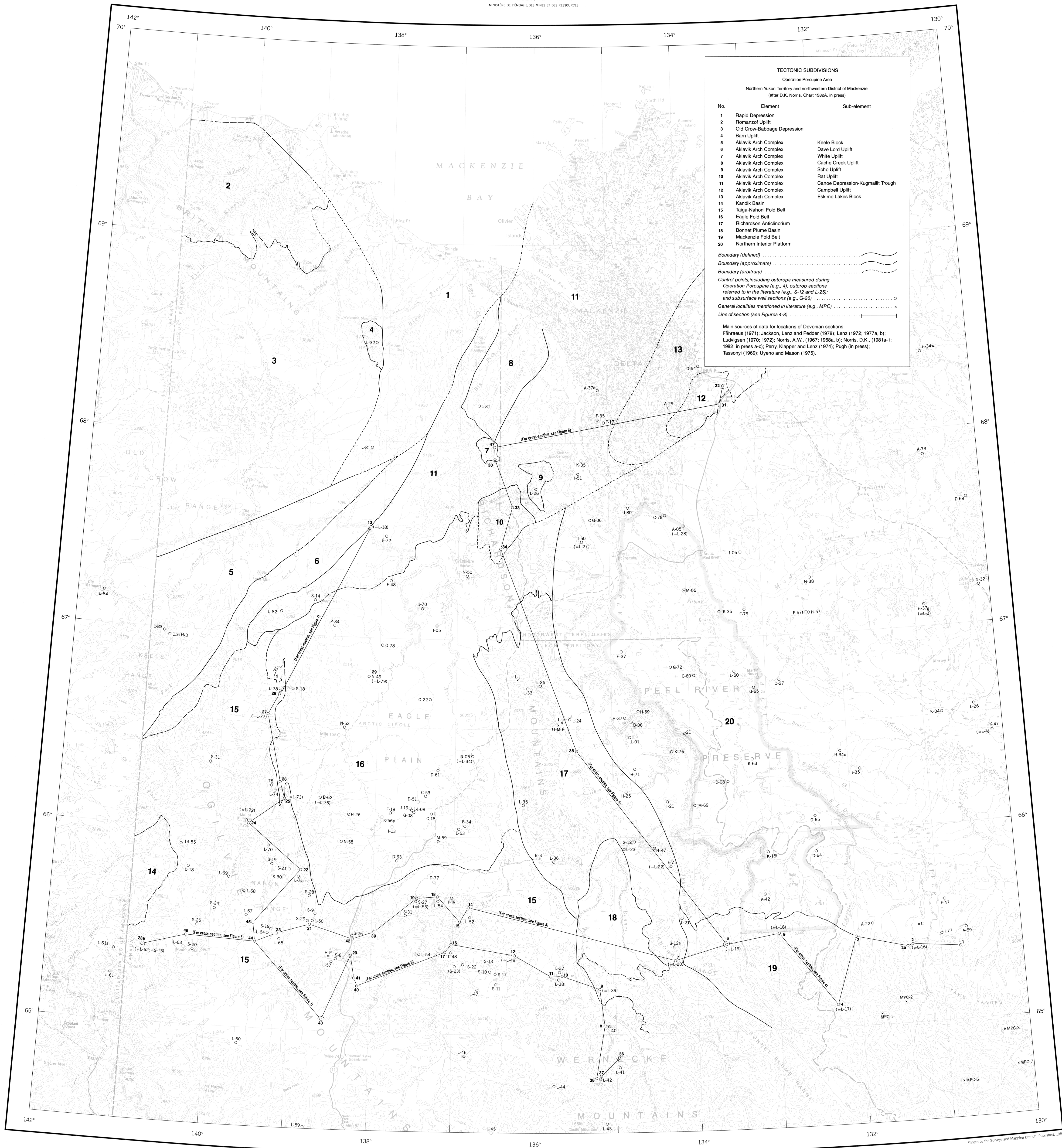
Figure 2. Tectonic subdivisions of the area, control points, and lines of section
